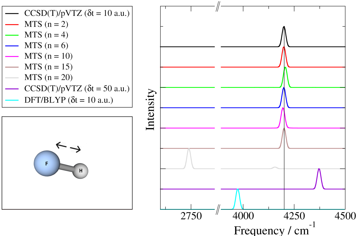
Figure 7: Vibrational spectra of hydrogen fluoride in vacuum obtained from AIMD simulations at the combined CCSD(T)/cc-pVTZ and BLYP/PW levels of theory with CCSD(T)/cc-pVTZ calculations only every n th step where n = 2, 4, 6, 10, 15 , or 20 . Frequencies are given in \text{cm}^{-1} .
