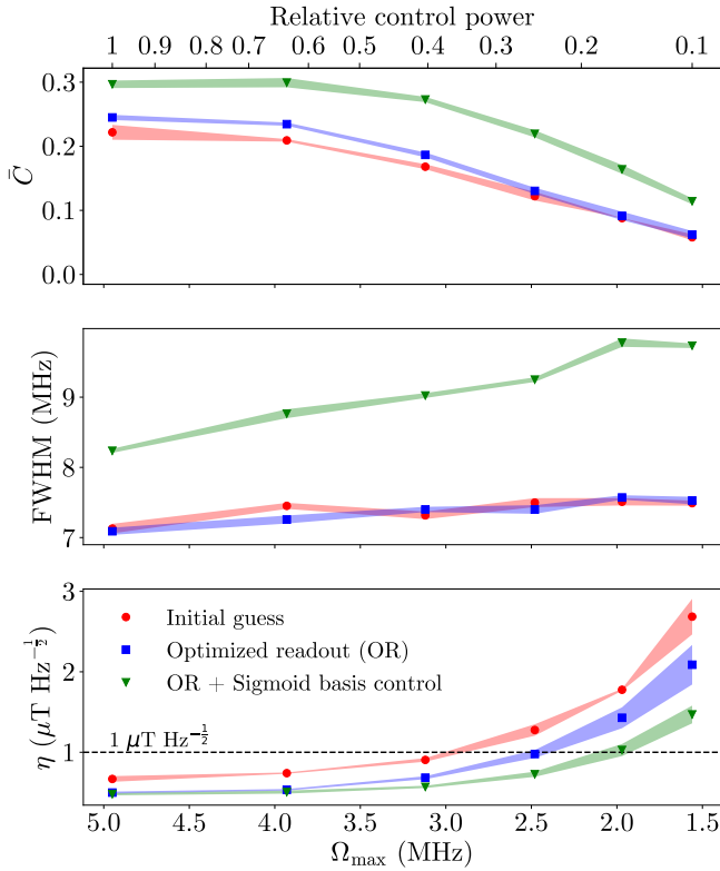
Figure 9. Comparison of pulsed ODMR measurements with optimized and standard spin state inversion pulses (NV3 from table I). Specifically, the robustness against amplitude variation is shown for pulses optimized in the Sigmoid basis. From top to bottom, the contrast, and FWHM of the resonance peaks as well as the corresponding average sensitivity \eta are shown. All results are obtained with different amplitude variations. The red curves indicate the initial guess. Blue curves correspond to the experiments performed with optimized spin readout parameters. The green curves show the results for the experiments using optimized MW pulses. The dashed line in the bottom plot shows the ceiling for the \eta of 1\mu\text{T Hz}^{-\frac{1}{2}} .
