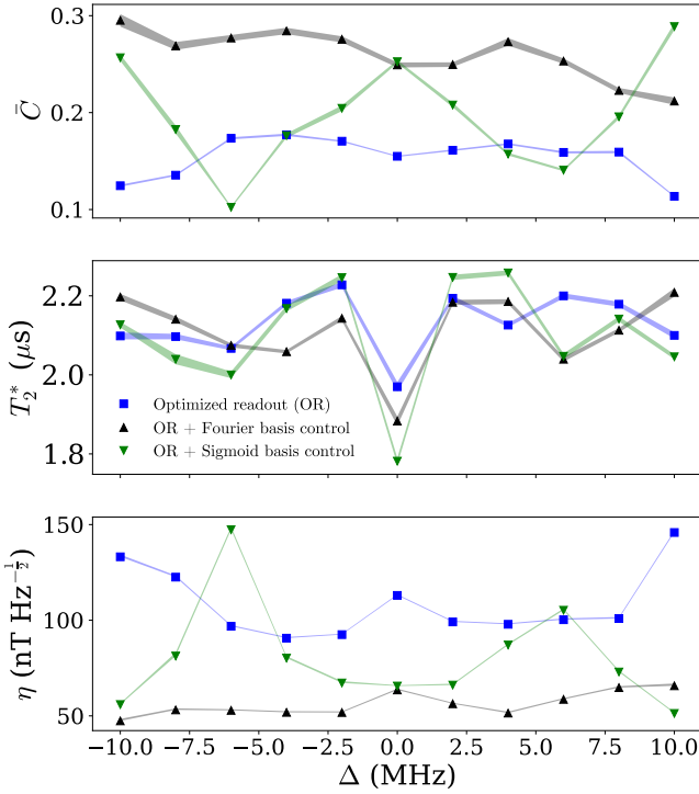
Figure 11. Comparison of Ramsey sequences with standard and optimized MW \pi/2 -pulses. All measurements are performed with optimized laser pulses for the readout and the optimizations were carried out with the amplitude-robust FoM from Eq. (11). The performance of the pulses optimized with the Fourier (black) and Sigmoid (green) basis is compared to the rectangular control pulse (blue) over a range of drive detunings \Delta . This range is equivalent to a variation of 0.35 mT in the external magnetic field. The upper panel shows the readout contrast \bar{C} . The respective T_2^* values are displayed in the middle panel. The bottom panel shows the resulting \eta . The sensitivity calculation is discussed in appendix C.
