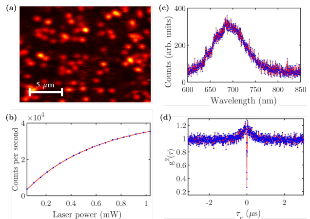
Figure 2. Sample characterization; (a) Confocal scan of the diamond sample with shallow single NV centers. (b) Count rate of a single NV vs. the input laser power (this corresponds to a source power in the range of 0 to 40 mW). The saturation behavior can be studied to obtain the excitation power with the best signal-to-background ratio for the experiments. Ideally, this lies below the saturating laser power. (c) Typical emission spectra of the single NV centers in the sample. The NV charge states have different spectral signature, the given spectrum indicates negatively charged NV state. (d) Exemplary second order correlation measurement, which is performed to identify single NV centers in the sample. \tau_c is the delay time in the photon antibunching measurement with the NV ( g_2(0) \approx 0.27 ).
