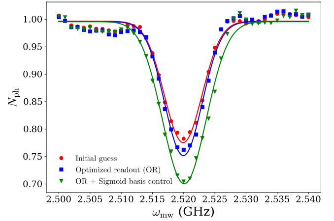
Figure 8. Pulsed ODMR in presence of a bias magnetic field ( B_{\text{NV}} \approx 12 mT, NV3 from table I) with optimized laser parameters and MW pulses. Following the results from Fig. 7 the optimization was done with the Sigmoid basis, using the bandwidth-limited restriction approach. The data shows the improvement in contrast with each step of the optimization. The initial contrast for the resonance peaks is ca. 0.22 (initial guess, red), which is further improved to ca. 0.24 with optimized laser parameters (blue). The MW pulse optimized in the Sigmoid basis on top improves the contrast to ca. 0.30 (green). The solid lines show the Gaussian fits for the respective data (see appendix C).
