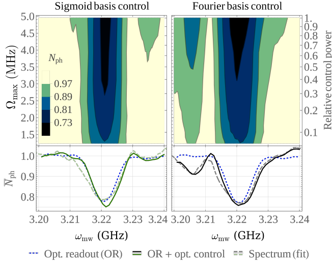
Figure 7. Comparison between two optimized spin inversion pulses in presence of a bias field B_{\text{NV}} = 12 mT (table I, NV2). The left (right) side shows the experimental results from a pulse optimized with the Sigmoid (Fourier) basis. (top) Normalized counts N_{\text{ph}} over a range of \Omega_{\text{max}} and drive frequencies \omega_{\text{mw}} . (bottom) Average normalized count \bar{N}_{\text{ph}} over all \Omega_{\text{max}} for the optimized pulse (solid) and initial guess (blue, dotted). The spectra of the pulses (dashed) are convoluted with the NV's natural emission line and fitted to the average counts.
