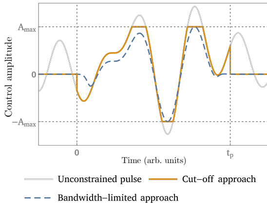
Figure 4. Restriction approaches. The unconstrained pulse may either be cut off at the amplitude \{-A_{\max}, A_{\max}\} and time \{0, t_p\} limits ("cut-off approach") or shifted and rescaled to fit within the available window ("bandwidth-limited approach").
