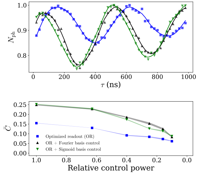
Figure 10. Optimized Ramsey measurements. The top plot shows the measurements performed at peak drive power with rectangular control pulses (blue) as well as optimized pulses in the Fourier basis (black) and Sigmoid basis (green). The optimized pulses exhibit almost double the contrast in comparison to the rectangular control pulse, with a similar precession frequency corresponding to the hyperfine levels of the transition. The length of the rectangular \frac{\pi}{2} -pulse is determined by performing Rabi measurements, and in this case is 67 ns. The bottom plot shows the variation in readout contrast with respect to the change in relative control power of the control pulse. The performance of the robust optimized pulses surpasses the rectangular control pulse over the entire range of tested control power (90% variation).
