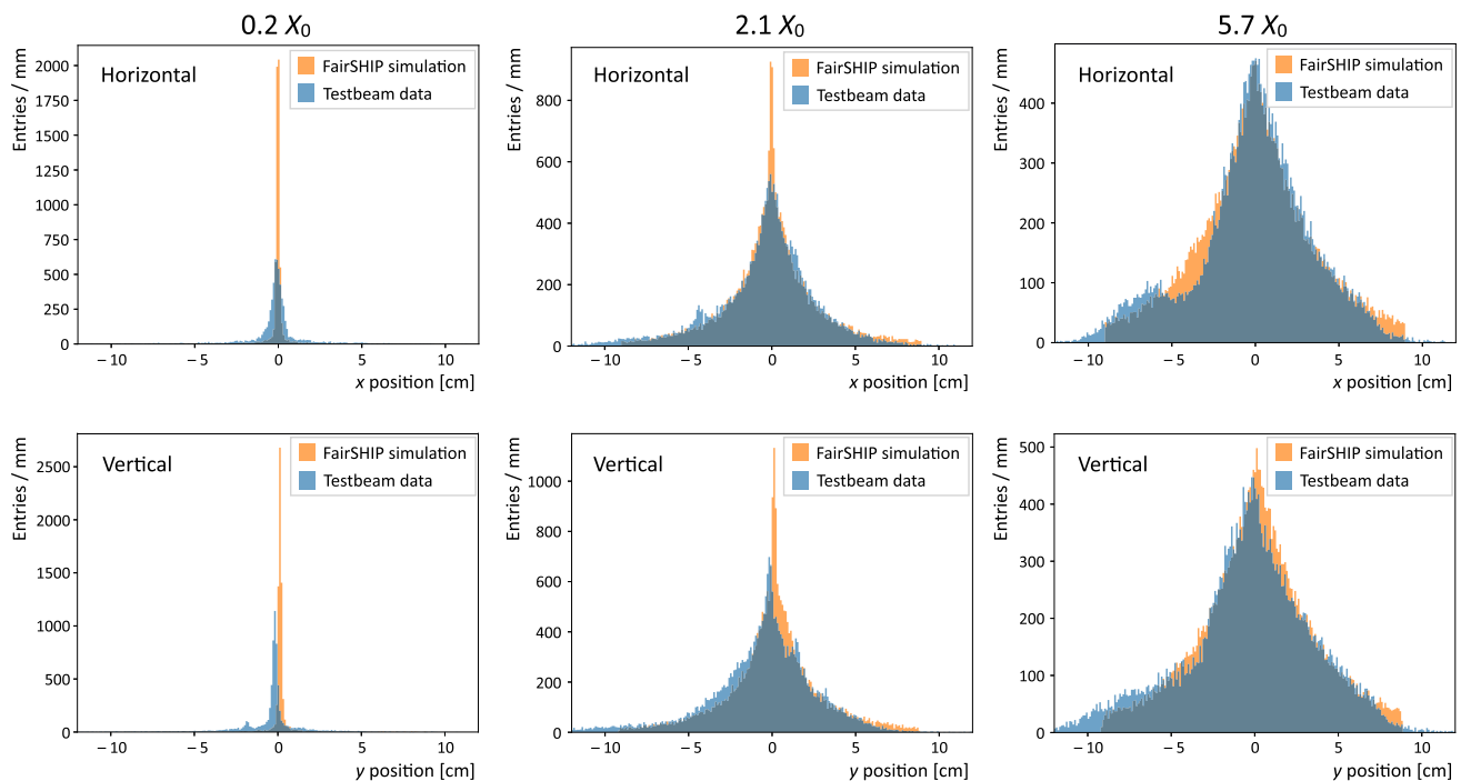
Fig. 20 Measured and simulated transverse electromagnetic-shower distribution with 5 GeV electrons from the CERN PS at different calorimeter depths. The small discrepancies between simulation and data are mostly due to known issues of the prototype read-out
