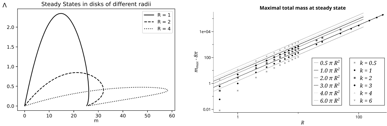
Fig. 1. Left: Curves of steady states as solutions of (76); shown is the Lagrange multiplier \Lambda plotted against the total mass m = \int_{\Omega} u for k = 1 and disks B_R(0) \subset \mathbb{R}^2 of radii R = 1 , R = 2 , and R = 4 , respectively. Note the more pronounced tilt to the right for increasing R and the common end points (0, 0) and (8\pi, 0) for all curves. Right: Log-log plot of the maximal value of m = \int_{\Omega} u , corrected for 8\pi , in numerically found steady state solutions in \Omega = B_R(0) \subset \mathbb{R}^2 depending on R for different values of k . The data points are the values determined from simulation, the dashed lines correspond to the curves m - 8\pi = k\pi R^2 .
