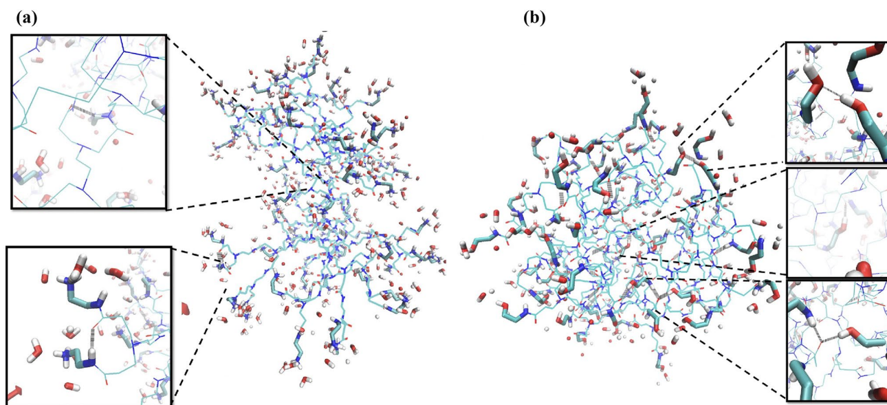
Fig. 3 Waters surrounding group terminals and hydrogen bonds formed between terminal groups and waters/dendrimer internal groups. a PAMAM- \text{NH}_2 and b PAMAM-OH, at neutral pH
