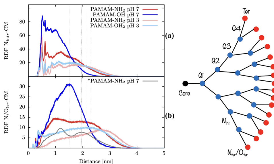
Fig. 6 Radial distribution function of molecular groups with respect of the dendrimer COM. a Internal nitrogen atoms and b terminal nitrogen/oxygen atoms. Schematic diagram at the right of the panel showing the internal and terminal nitrogens. GX states for the dendrimer generation. *Thinner grey line states for comparison from previous work in the literature [31]. Grey vertical dashed line represents the R_g of the dendrimers
