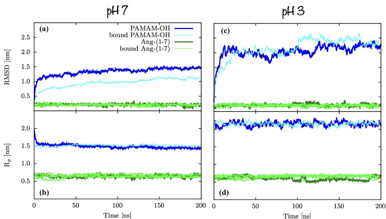
Fig. 20 Structural stability changes of peptide or PAMAM-OH upon binding. RMSD of structures in complex compared with same structures free in solvent for a neutral pH and c acidic pH. R g of structures
