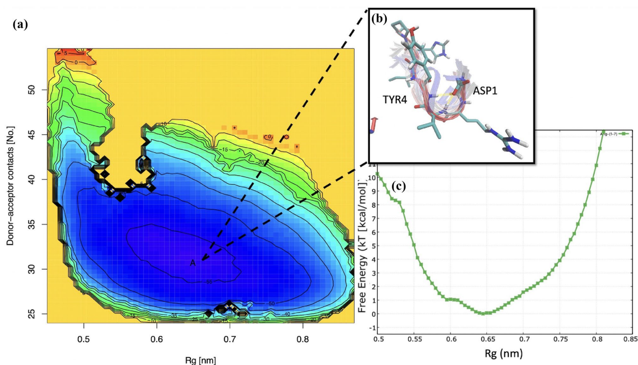
Fig. 10 Ang(1-7) 2D a Free Energy Surface (FES) as a function of the total number of donor-acceptor contacts and the R_g . Isoenergy lines are drawn every 5 kcal/mol. T = 300 K, pH 7. b Structures rep-
