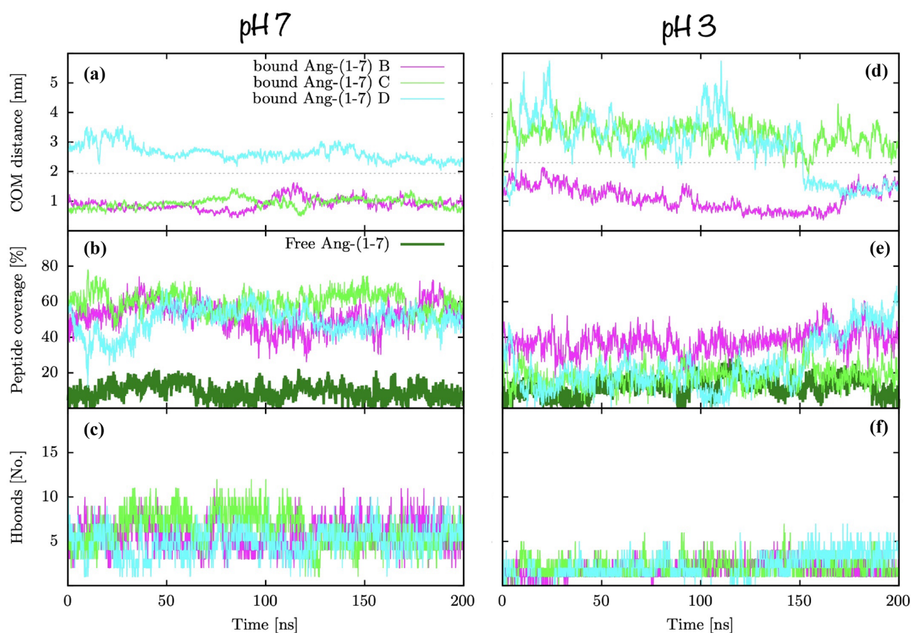
Fig. 15 [PNH-A] n ) stability. a Distance from dendrimer COM to Ang-(1-7) peptides, b peptide coverage according to SASA values and c number of hydrogen bonds between dendrimer and peptides. #
