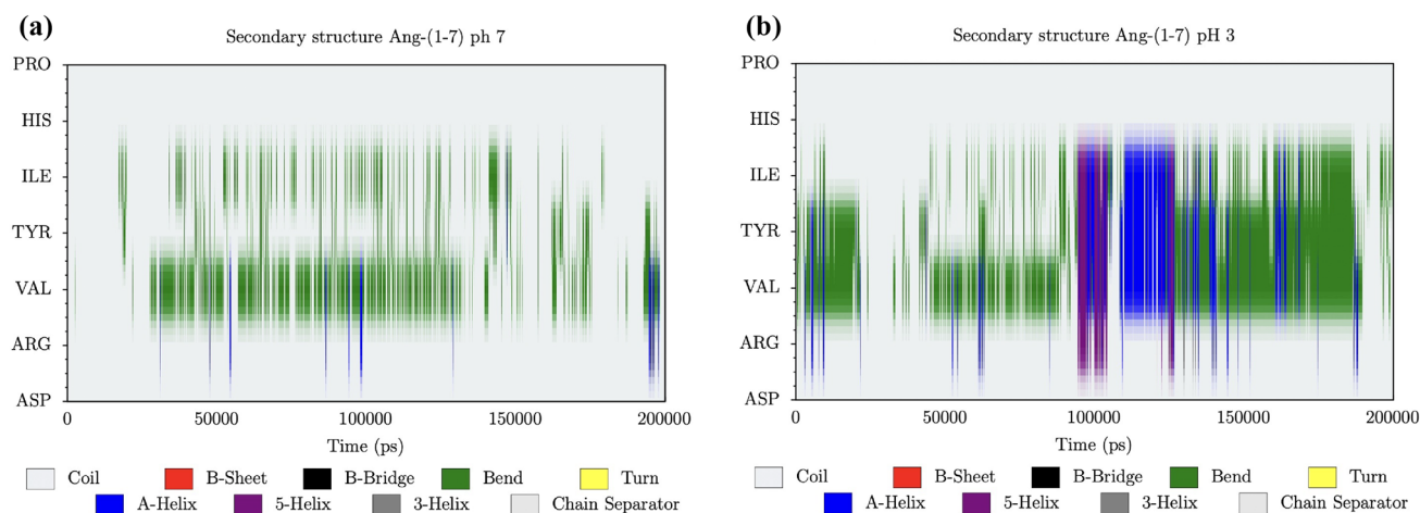
Fig. 8 Ang-(1-7) secondary structure as a function of time. a At neutral pH and b at acidic pH
