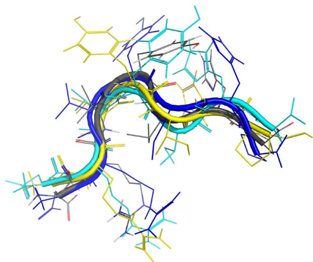
Fig. 9 Superimposition of: experimental NMR structure obtained at acidic pH (grey), structure repeated 40 % of the frames in classical MD simulation performed under neutral pH (blue), structure repeated 35 % of the frames in metadynamics simulation performed under neutral pH (cyan), structure repeated 60 % of the frames in classical MD simulation performed under acidic pH (yellow)
