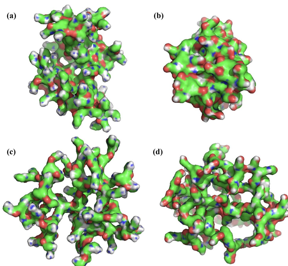
Fig. 5 Dendrimers cavities comparison. a PAMAM- \text{NH}_2^n , b PAMAM- \text{OH}^n , c PAMAM- \text{NH}_2^a and d PAMAM- \text{OH}^a at 200 ns. Letters “a” and “n” states for neutral and acidic pH
