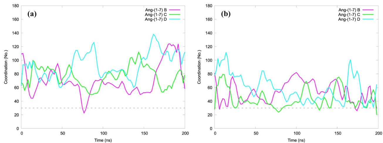
Fig. 22 PAMAM-OH/Ang-(1-7) coordination number along simulation time at a neutral pH and b acidic pH. Coordinations mean the number of atoms from the peptides that are within 0.3 nm of the dendrimer. # B-D refers to the different Ang-(1-7) peptides bonded
