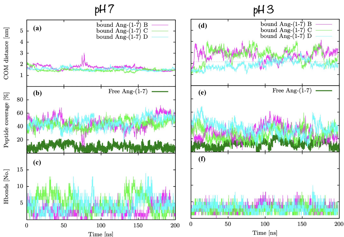
Fig. 21 [POH-A] n stability. a Distance from dendrimer COM to Ang-(1-7) peptides, b peptide coverage according to Solvent-Accessible Surface Area (SASA) values and c number of hydrogen bonds
