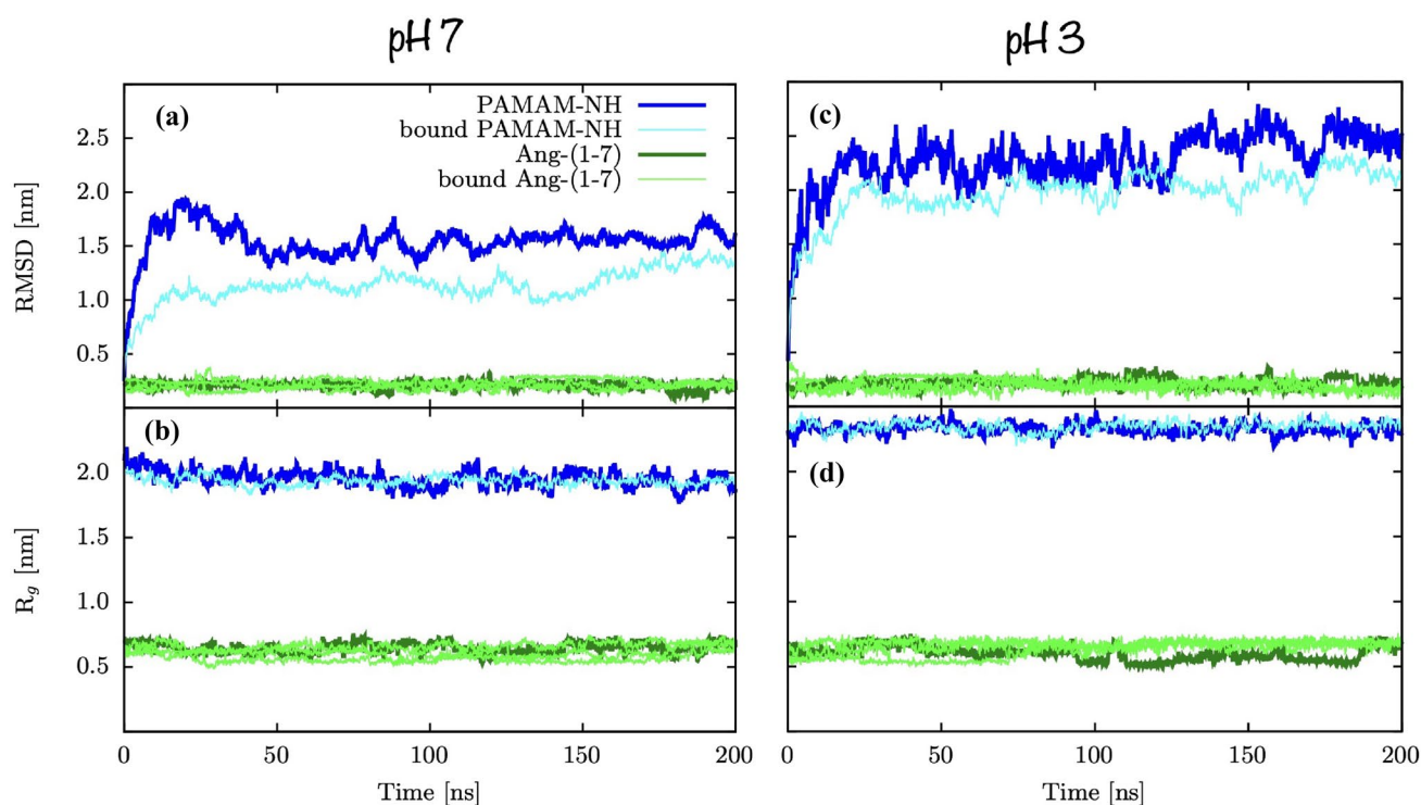
Fig. 14 Structural stability changes of peptide or PAMAM-NH upon binding. RMSD of structures in complex compared with same structures free in solvent for a neutral pH and c acidic pH. R_g of structures
