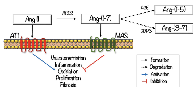
Fig. 1 Diagram representing the main metabolic effects driven by the Renin Angiotensin System bioactive peptides (Ang II and Ang-(1-7)) when interacting with its cell receptors AT1 and MAS, respectively. The main proteolytic cleavage of Ang-(1-7) by angiotensin-converting enzyme (ACE) and dipeptidyl peptidase 3 (DPP3), which is associated with Ang-(1-7) rapid degradation and limited therapeutic application
