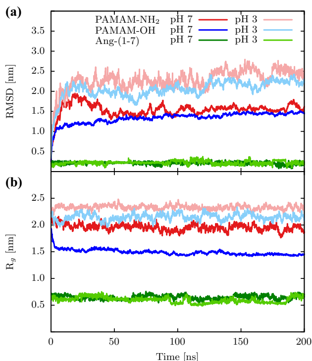
Fig. 2 Structural features of PAMAM-NH 2 , PAMAM-OH and Ang-(1-7) systems. a RMSD and b R_g values as function of time
