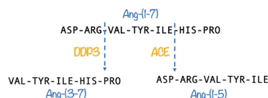
Fig. 17 Proteolytic cleavage of Ang-(1-7) by ACE and DPP3
