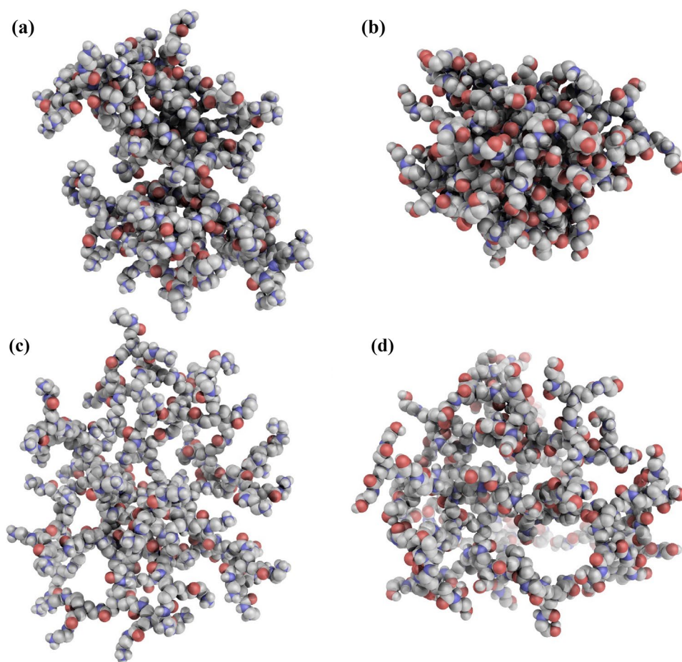
Fig. 4 Dendrimers shape comparison. a PAMAM- \text{NH}_2^n , b PAMAM- \text{OH}^n , c PAMAM- \text{NH}_2^a and d PAMAM- \text{OH}^a at 200 ns of MD simulation. Letters “a” and “n” states for neutral and acidic pH
