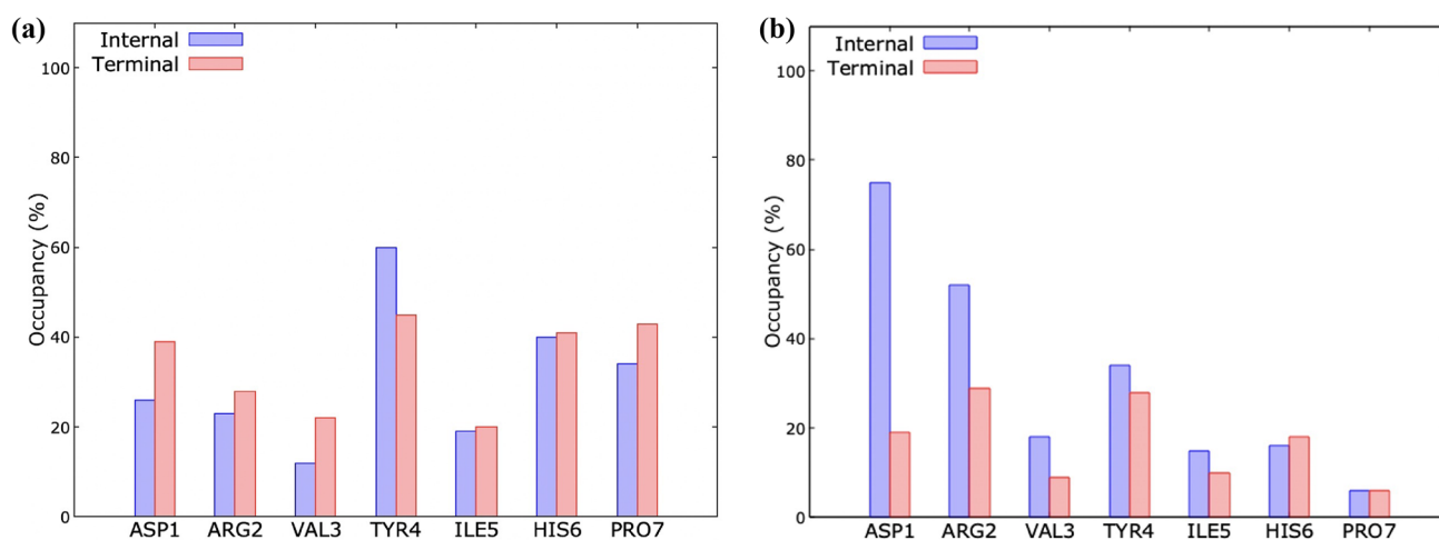
Fig. 24 Occupancy percentage of the amino acids in the final 100 ns of MD simulation at a neutral pH and b acidic pH. Determined by considering the contacts per amino acids at 3.0 Å from the dendrimer
