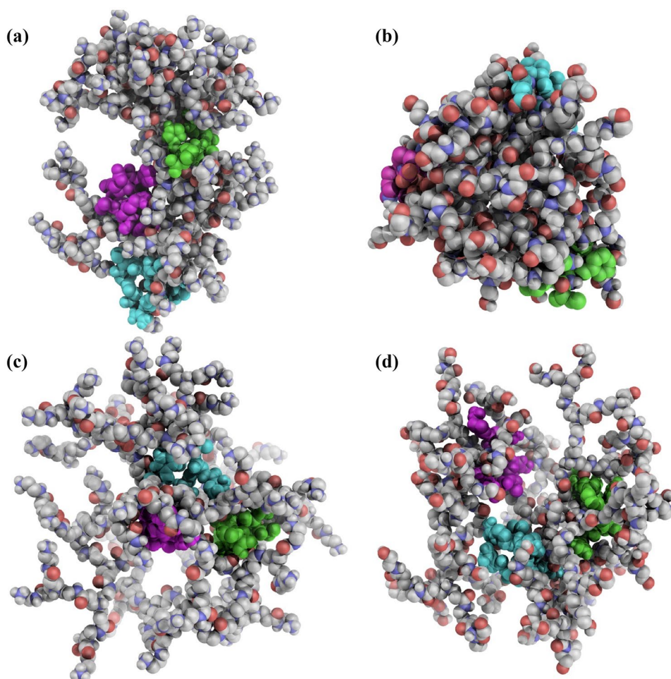
Fig. 12 Double-docking schematic representation. Each of the peptides conformer is allowed to find a site by using a blind rigid docking, afterwards, once the peptide found a reasonable site, a flexible docking allows it to better accommodate into the site
