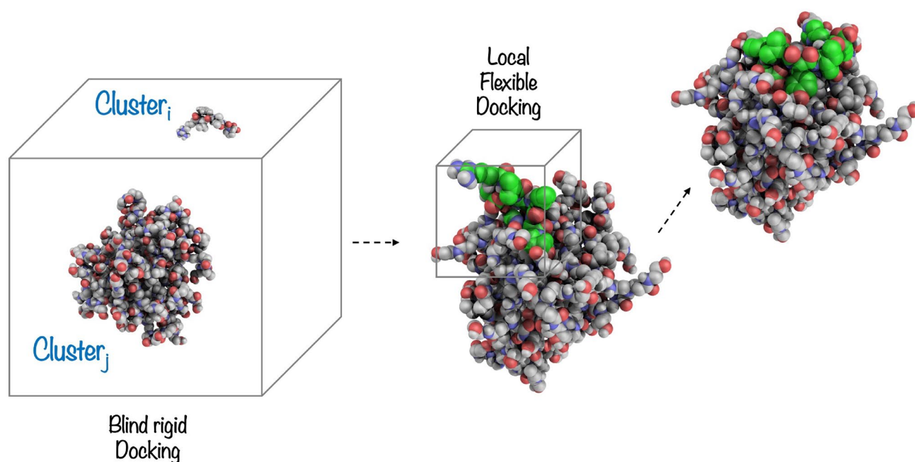
Fig. 12 Double-docking schematic representation. Each of the peptides conformer is allowed to find a site by using a blind rigid docking, afterwards, once the peptide found a reasonable site, a flexible docking allows it to better accommodate into the site
