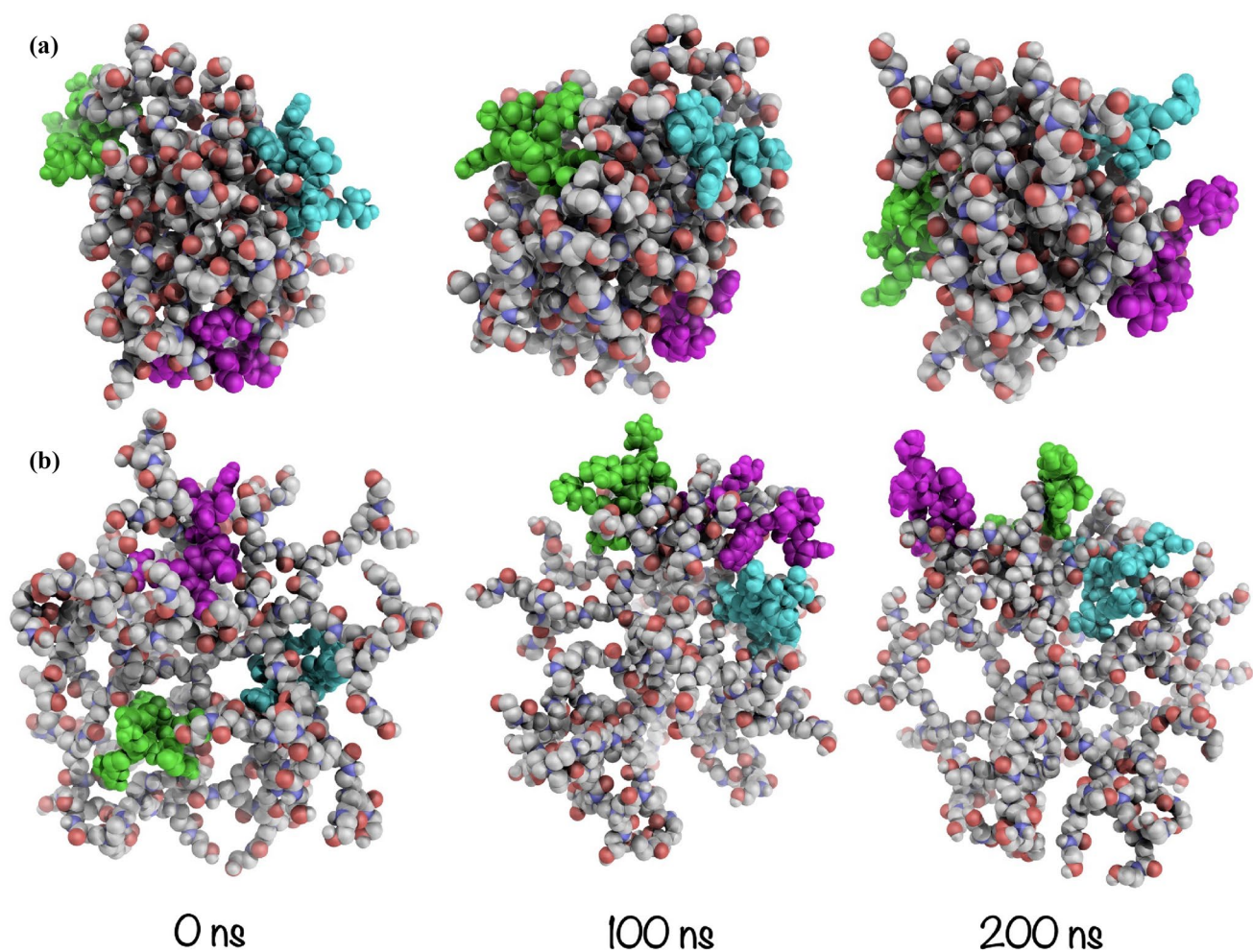
Fig. 23 Time evolution of PAMAM-OH/Ang-(1-7) complex structures at a neutral pH and b acidic pH
