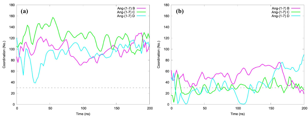
Fig. 16 PAMAM-NH/Ang-(1-7) coordination number along simulation time at a neutral pH and b acidic pH. Coordination mean the number of atoms from the peptides that are within 0.3 nm of the dendrimer. # B-D refers to the different Ang-(1-7) peptides bonded
