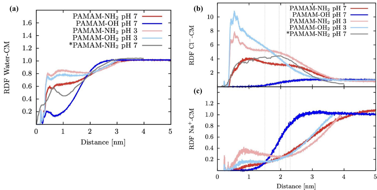
Fig. 7 Radial distribution function of molecules with respect of the dendrimer COM. a Water molecules and b \text{Cl}^- ions and c \text{Na}^+ ions. *Thinner grey line states for comparison from previous work in the literature [31]. Grey vertical dashed line represents the R_g of the dendrimers
