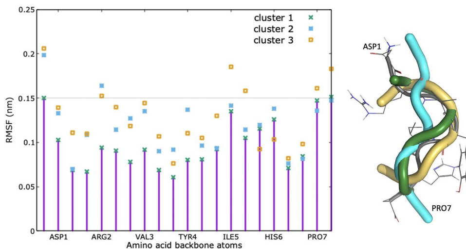
Fig. 11 RMSF of Basin A main clusters as a function of aminoacid backbone atoms. Structures representative of the basin A main clusters are superimposed in the right Fig.. Grey represent the NMR structure. Threshold of 0.15 nm is marked to visualize the most flexible atoms. Cluster 1 is marked also with impulses to guide visualization
