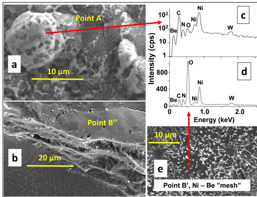
Figure 13. Surface structure and composition of co-deposits on the beryllium IWG limiter after all three ILW campaigns. Sampling areas A and B are marked in Figure 12. Figures 13(c) is reproduced from [171].
