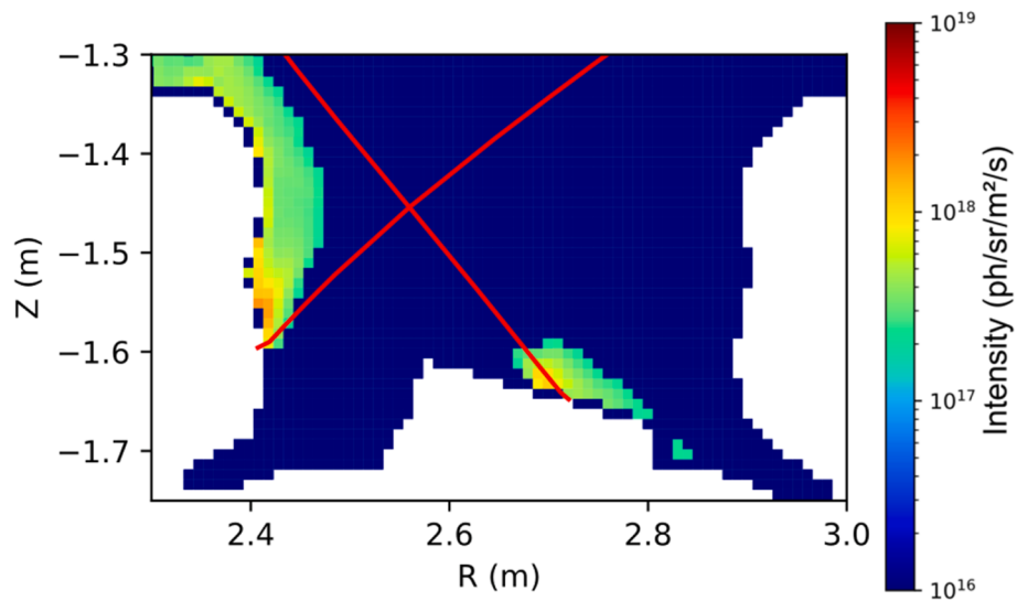
Fig. 4. Poloidal tomographic reconstruction of W I 400.9 nm line emission in the JET divertor in JPN 94,605 (10 s) measured using a tangentially viewing endoscope camera equipped with a wavelength filter. Intensities below 2 \cdot 10^{17} ph sr -1 m -2 s -1 are masked to zero due to significant contributions from continuum radiation.
