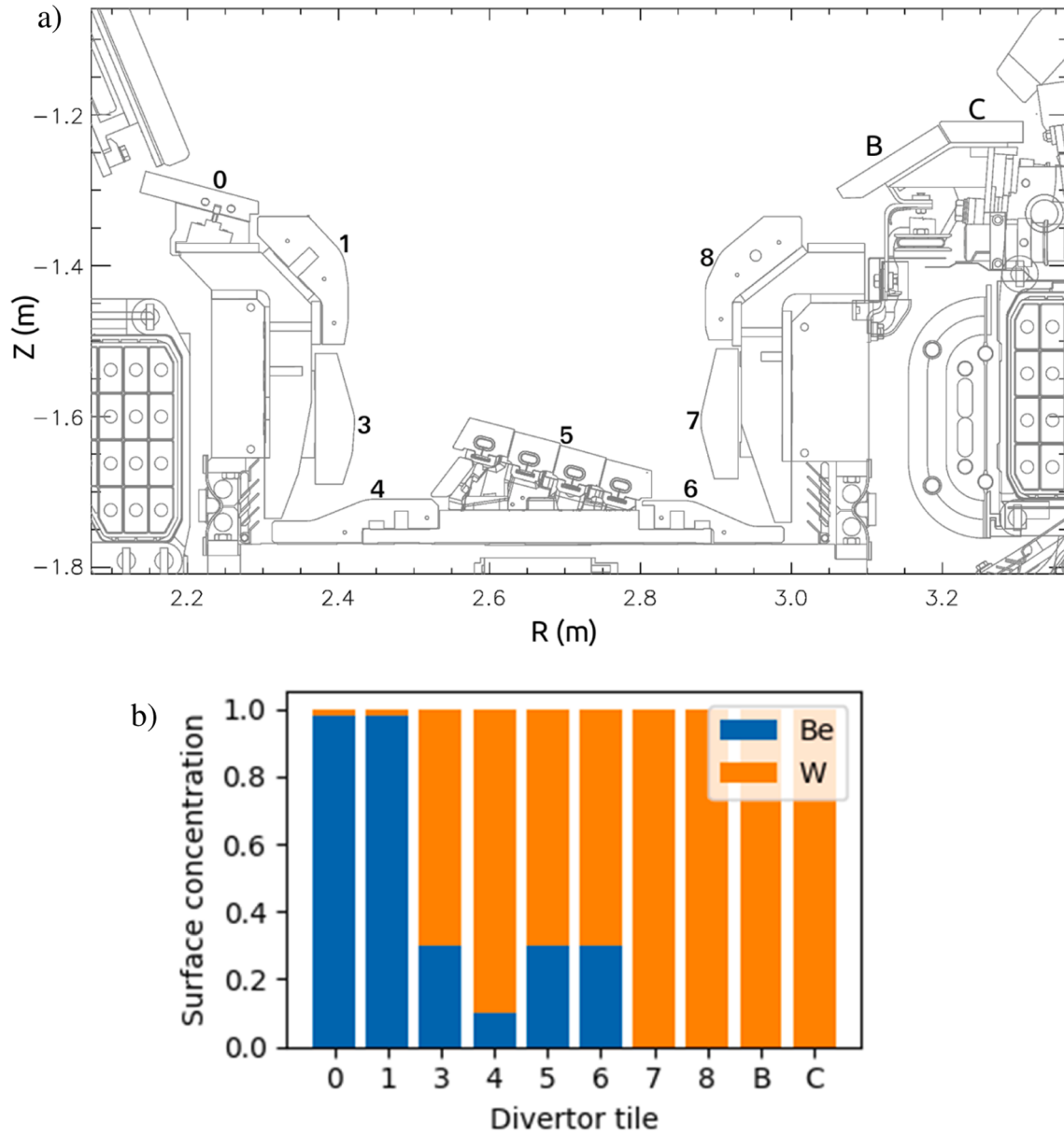
Fig. 1. JET-ILW divertor plasma-facing components. a) Poloidal cross-section of the divertor geometry with labels for each W divertor tile. b) Surface concentration of Be and W assumed in ERO2.0 within a 5 nm surface layer. The justification for the 30 % Be concentration [6] assumed on tiles 3, 5, and 6 is to obtain an ERO2.0 plasma Be concentration consistent with the Be concentration inferred from measured divertor Be II emission, as the value 30 % is not based on observations of the Be surface concentration in experiments or post-mortem tile analysis [16].
