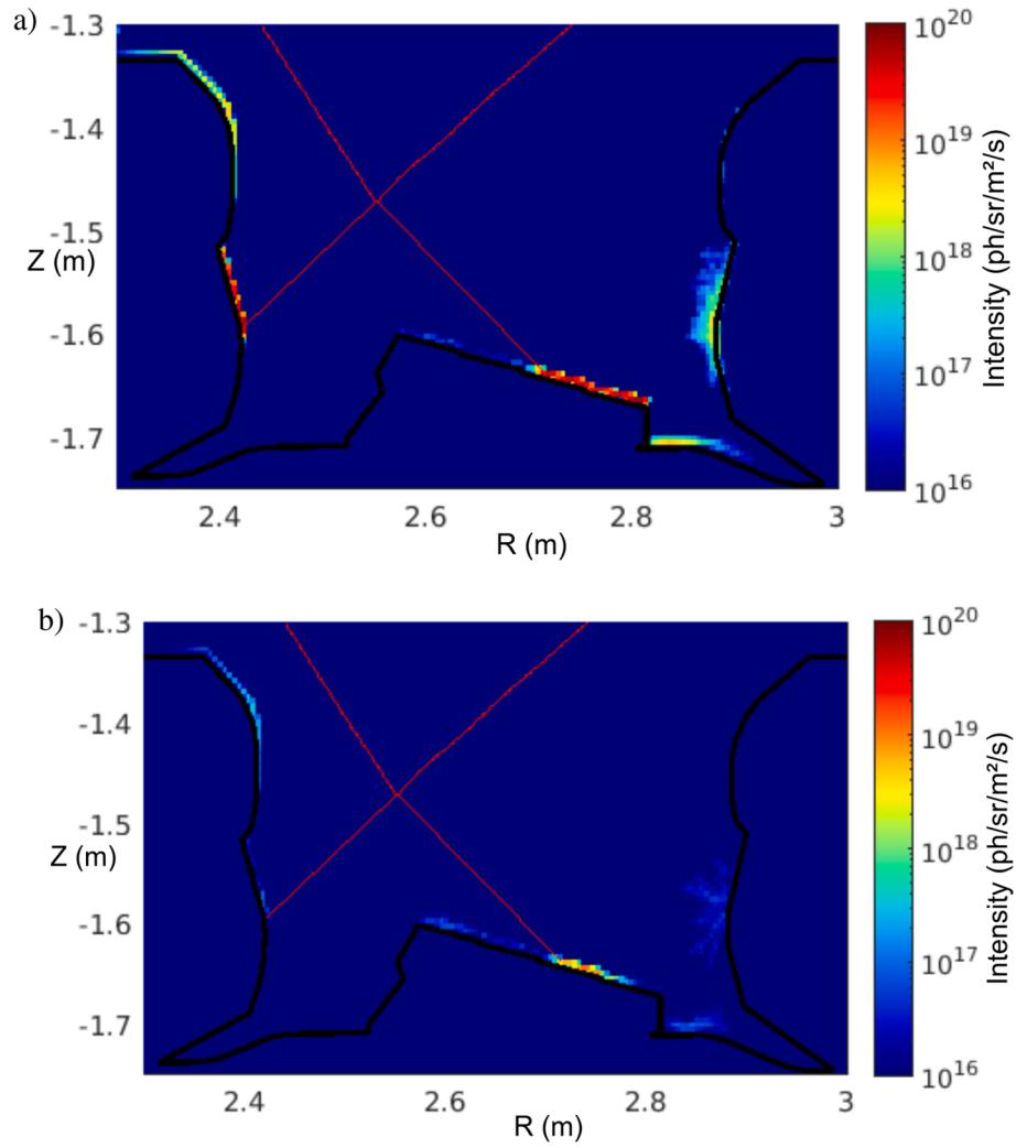
Fig. 3. Synthetic reconstructions of the W I 400.9 nm line emission predicted by ERO2.0 for the ELM (a) and inter-ELM (b) phases of JPN 94,605 (10 s).
