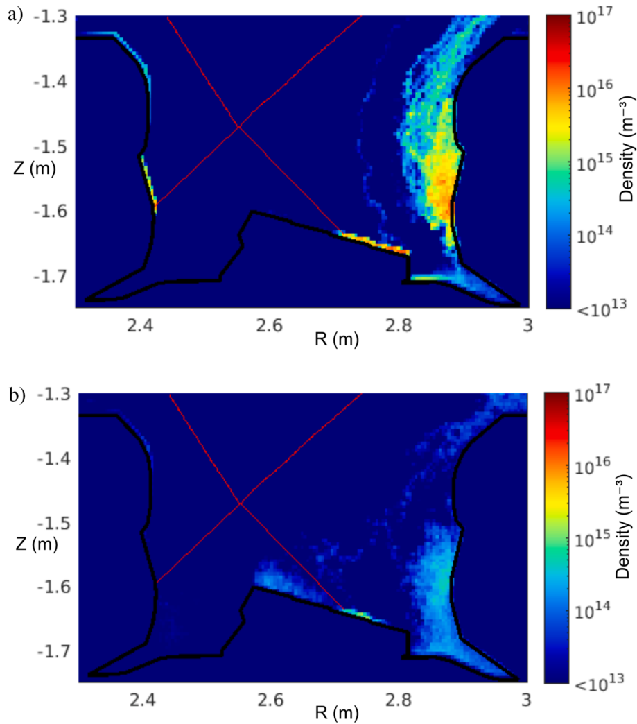
Fig. 2. Poloidal cross-sections of W density profiles in the JET divertor predicted by ERO2.0 for steady-state ELM (a) and inter-ELM (b) phases of JPN 94,605 (10 s).
