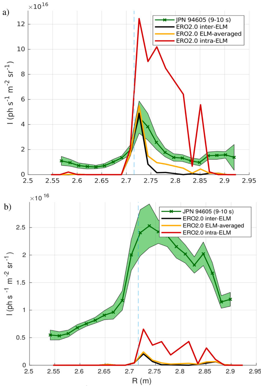
Fig. 5. Line-integrated W I 400.9 nm emission (a) and W II 434.8 nm emission (b) in the JET low-field side divertor in JPN 94,605 (9–10 s) measured by a mirror-link Czerny-Turner divertor spectrometer with a time resolution of 25 Hz (green, with shaded area indicating one standard deviation) and predicted by ERO2.0 for the inter-ELM (black) and intra-ELM (red) phases. The duration-weighted ELM-averaged W I intensity, assuming an ERO2.0 ELM cycle with 2 ms ELM duration and 40 Hz frequency, is shown in orange. The vertical dashed blue line indicates the radial location of the strike line. (For interpretation of the references to colour in this figure legend, the reader is referred to the web version of this article.)
