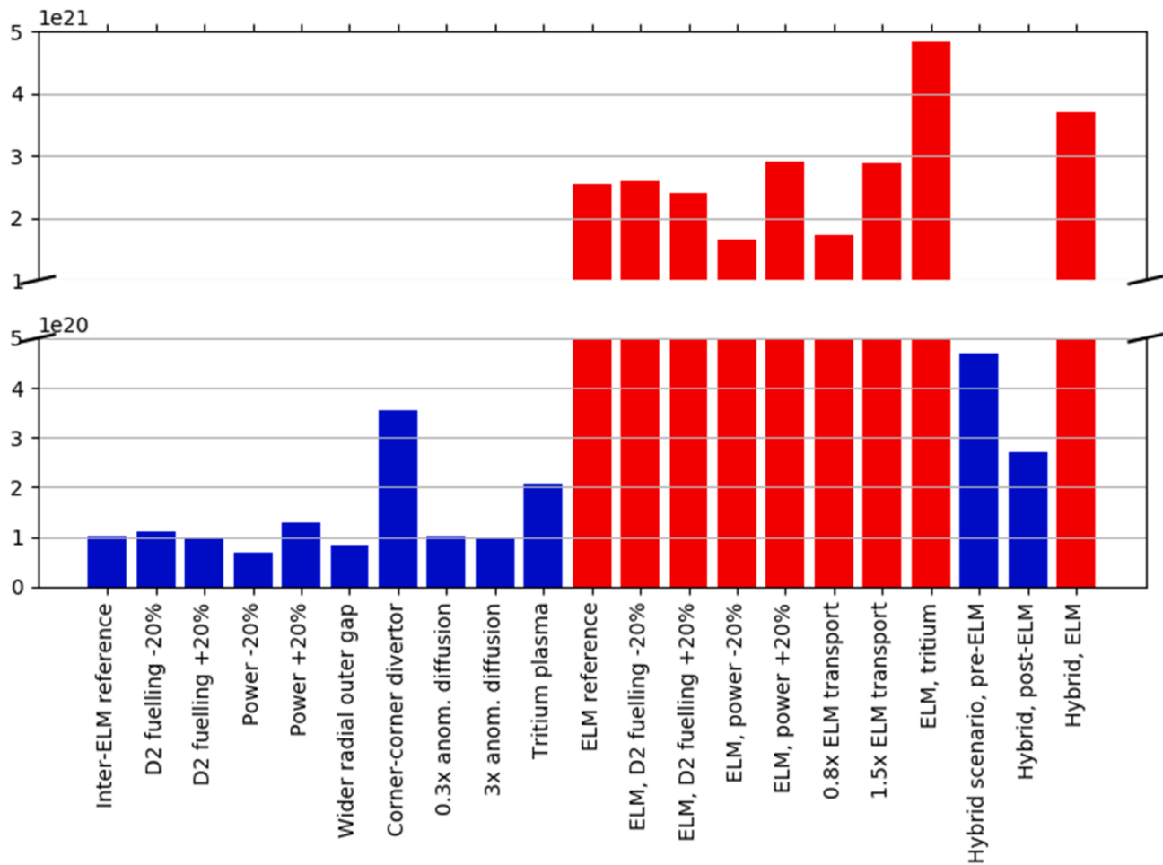
Fig. 6. Total W gross erosion rate predicted by ERO2.0 in the modelled plasma scenarios, including the sputtering by atomic and ionic D (or T), Be, and W on all JET-ILW W plasma-facing components. Inter-ELM phases are represented in blue and ELM phases in red. The y-axis is cut, and the top and bottom parts are shown on different scales for readability. (For interpretation of the references to colour in this figure legend, the reader is referred to the web version of this article.)
