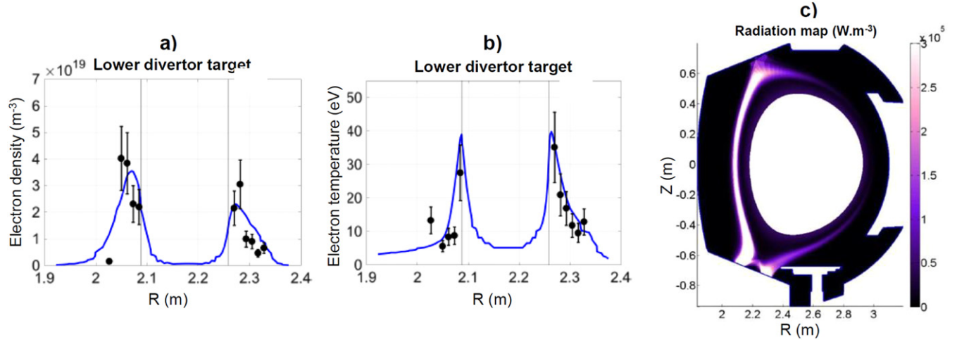
Figure 16. (a) Profiles of electron density and (b) electron temperature at the lower divertor target for the WEST #54067. In blue solid line SOLEDGE2D simulation, in black symbols the LP measurements. (c) Radiation map from SOLEDGE2D simulation. The total radiated power is 780 kW in quantitative agreement with the bolometry measurements in the outer region.
