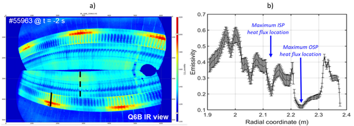
Figure 15. (a) IR image showing two 30° sectors of the lower divertor (optically recombined on one camera); (b) estimated emissivity along the W-coated tiles in the poloidal direction; usual locations of the inner strike point (ISP) and outer strike point (OSP) are indicated.
