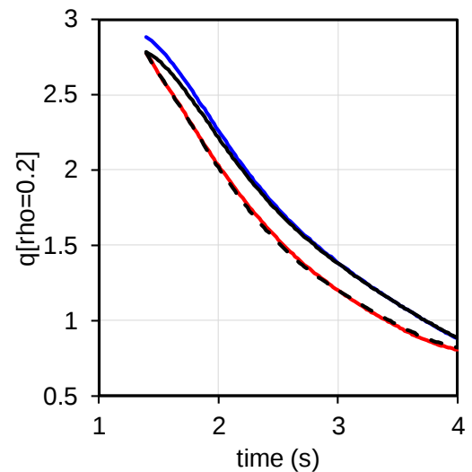
Fig.3 Modelled q[\rho=0.2] evolution for: D plasma (blue); H plasma (red); H plasma with \langle Z_{\text{eff}} \rangle_l & \langle T_e \rangle_v scaled to match D plasma (dashed black); H plasma with \langle Z_{\text{eff}} \rangle_l & T_e(r) taken from D plasma (solid black)
