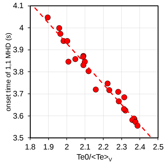
Fig.5 Delay in arrival time of q=1 surface plotted against electron temperature peaking averaged over t=1.5-3.5s .
