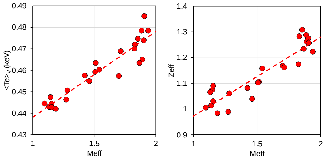
Fig.2. Volume averaged electron temperature (left) and Z_{\text{eff}} (right) plotted against the effective main ion isotope mass. All measurements averaged over t = 1.5\text{--}3.5\text{s} .
