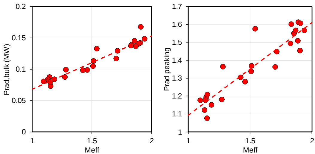
Fig.4. Bulk plasma radiation and central radiation peaking plotted against the effective main ion isotope mass. The radiation peaking is defined as the ratio of on-axis and off-axis horizontal channel signals from the bolometer camera. All measurements averaged over t=1.5-3.5s .
