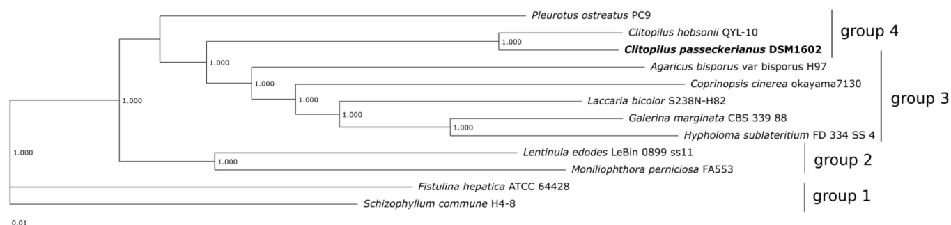
Figure 3. Phylogenetic tree of twelve selected Agaricales. The phylogenetic tree was build using SH-like local support values computed with ‘FASTtree 2.1’ within the comparative genomics tool ‘EDGAR 3.0’ on the bases of 1303 core genes. Branches show a perfect support value of 1.000.
