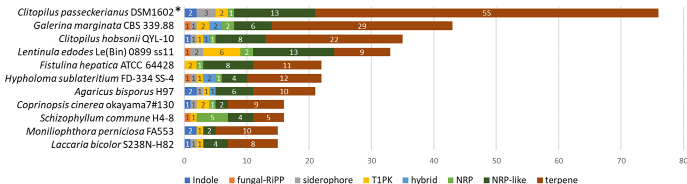
Figure 4. Distribution of BGCs in genomes of selected Agaricales. * Note that the genome of C. passeckerianus derives from the dikaryon and the actual number of BGCs presumably is even higher (see main text for details).
