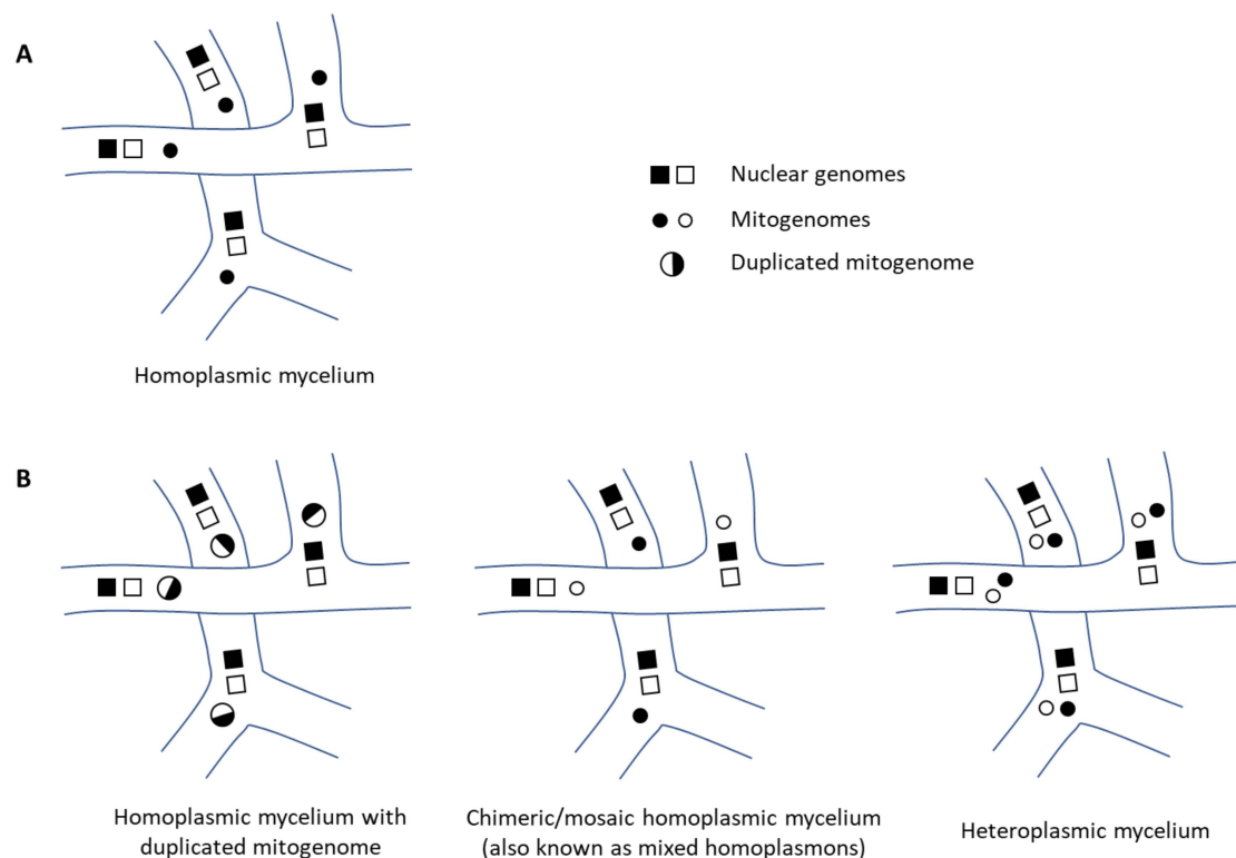
Figure 2. Distribution of mitogenomes and nuclear genomes in fungal mycelium. (A) Common scenario in Agaricales. (B) Possible scenario in C. passeckerianus .
