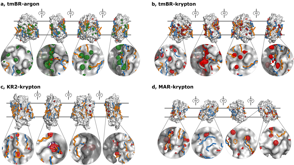
Fig. 2 Illustration of noble gas positions on the surfaces of the derivatised structures. tmBR ( a , argon; b , krypton), KR2-krypton ( c ), MAR-krypton ( d ). Each panel shows four orthogonal side views in the membrane. The hydrophobic membrane region is delimited with two black parallel lines. Krypton and argon atoms are shown as red and green spheres, respectively. Lipid fragments present in the derivatised structures are shown in sky-blue; lipid fragments from native structures are shown in orange for comparison. On the bottom of each panel four representative noble gas binding sites in each view are enlarged and the anomalous difference density krypton (red grid) or argon (green grid) are drawn at the 3.0 r.m.s. level. Symmetry-related molecules are shown in transparent dark to better illustrate the contacts.
