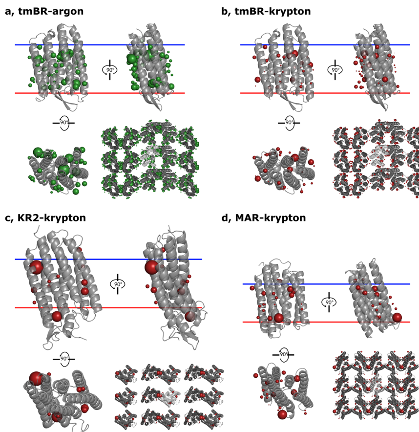
Fig. 1 Cartoon representations of the structures of tmBR-argon, tmBR-krypton, KR2-krypton, MAR-krypton. a tmBR-argon. b tmBR-krypton. c KR2-krypton. d MAR-krypton. Each panel shows side views of the proteins sitting in the membrane (top left and top right figures), a top view perpendicular to the membrane (bottom left), and a view of crystal packing contacts in the XY-plane (bottom right figure). Noble gas atoms are shown as red (krypton) and green (argon) spheres. Sphere sizes are proportional to atom occupancy.
