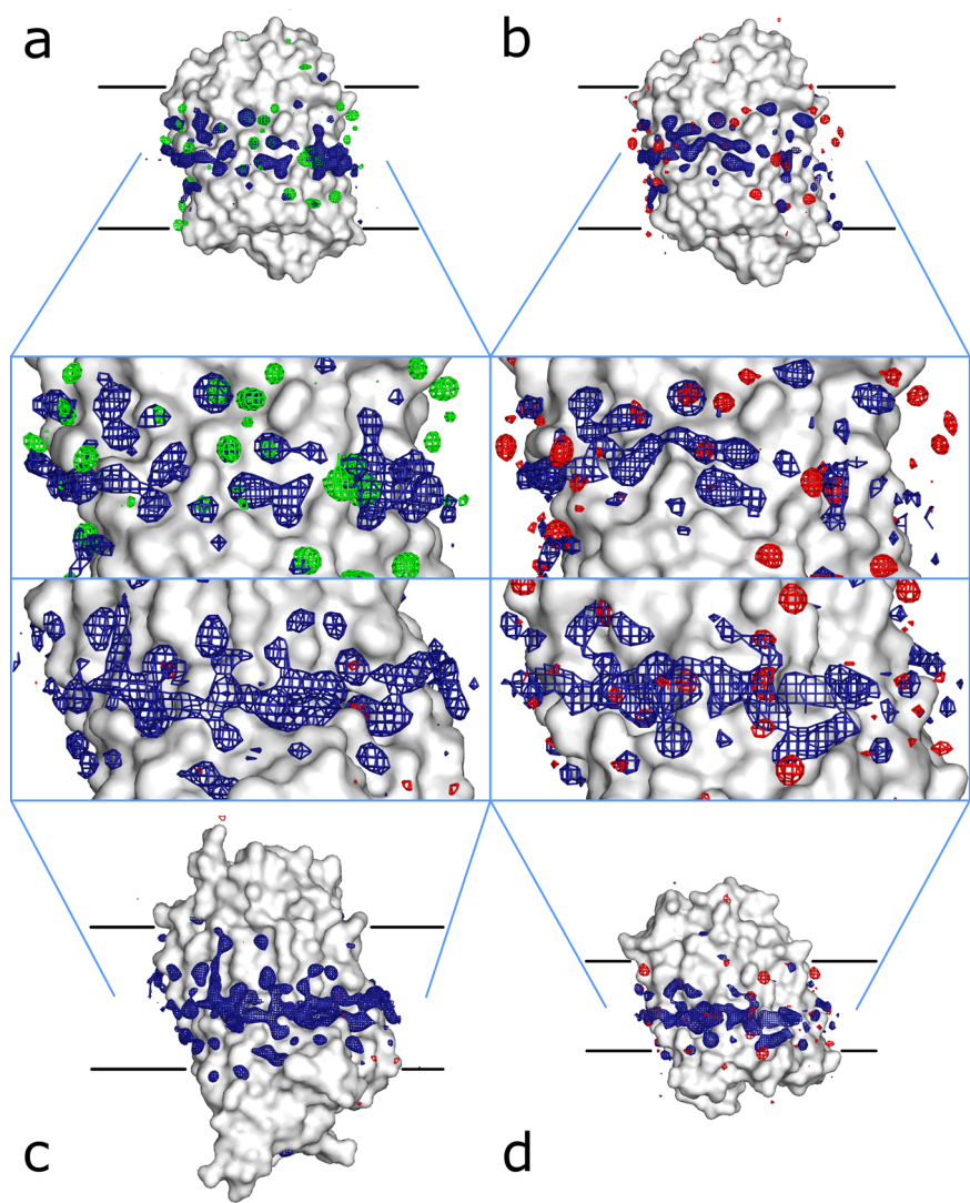
Fig. 4 Arrangement of peaks of the MD maps. MD maps are sampled at the level of {mean + 3.5×std.dev.} (navy blue grid) on the surface of the proteins. a tmBR-argon. b tmBR-krypton. c KR2-krypton. d MAR-krypton. Peaks in the anomalous difference maps obtained in crystallographic studies are shown (sampled at 3.5×r.m.s. level) in red (krypton) and green (argon).
