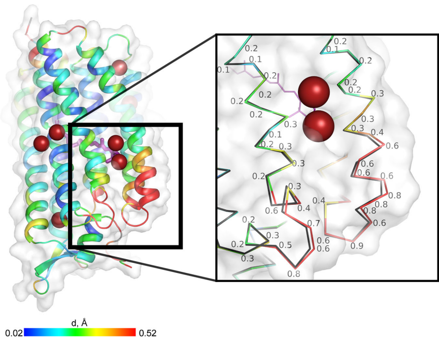
Fig. 3 Cartoon representation of the crystal structure of KR2-krypton. Cartoon colour illustrates C \alpha -position discrepancy (Å) between the derivatised and the native structures (with the scale at the bottom). In the zoom window, those discrepancies are detailed for each atom. Krypton atoms are shown as red spheres.
