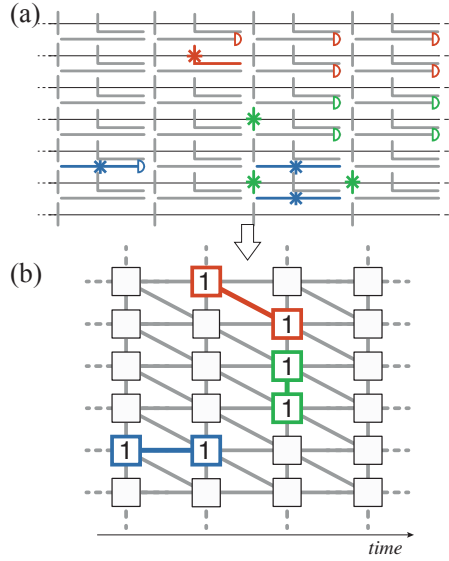
Figure 11: (a) Example of an error graph generated by physical errors. Positions where qubit, measurement and correlated data phase-flip and measurement errors can happen are represented by vertical, horizontal and L-shaped edges, respectively. Colored links represent occurred error events while colored semicircles represent the ancilla qubits triggered by an error event. From this graph we derive syndrome volume which is the input for the MWPM decoder. (b) Syndrome volume graph derived by the error graph in (a). The boxes labeled with 1s represent defects, i.e. ancilla qubits where the measurement outcome differs from the previous round of measurements. The colored diagonal red, vertical green and horizontal edges represent a possible matching of the defects.
