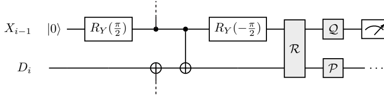
Figure 4: Cutout of one ancilla and one data qubit of the QEC circuit. All noise contributions of the circuit-level noise model (see Fig. 1(a) of the main text) can be merged into the three channels \mathcal{P} , \mathcal{Q} and \mathcal{R} . The effective error rates are given in Eq. (9).
