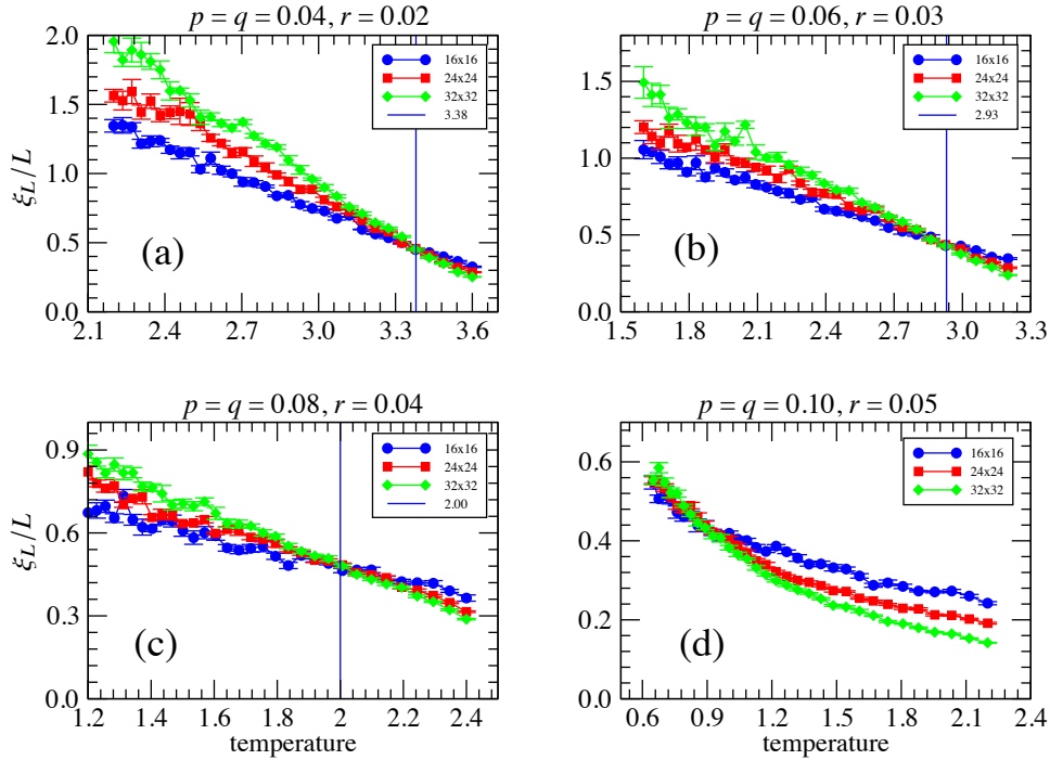
Figure 9: Critical temperatures from finite size scaling. The critical temperatures are found by locating the points where the lines representing the quantities \xi_L/L cross each other for different systems sizes L . Examples of the occurrence of a phase transition are shown in (a) for p = q = 0.04, r = 0.02 , in (b) for p = q = 0.06, r = 0.03 , in (c) for p = q = 0.08, r = 0.04 . If it is not possible to identify a temperature where the lines with the quantities \xi_L/L cross, the transition does not occur. This is shown in panel (d) for p = q = 0.10, r = 0.05 .
