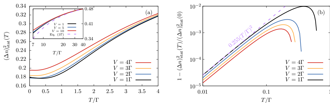
Figure 2: Stationary charge fluctuations (\Delta n)_{\text{stat}}^2 as function of temperature for U = 8\Gamma , \epsilon = -U/2 and several bias voltages. (a) Low and intermediate temperature regime. Inset: High temperature regime. (b) Scaling of the fluctuation for T \ll \Gamma .
