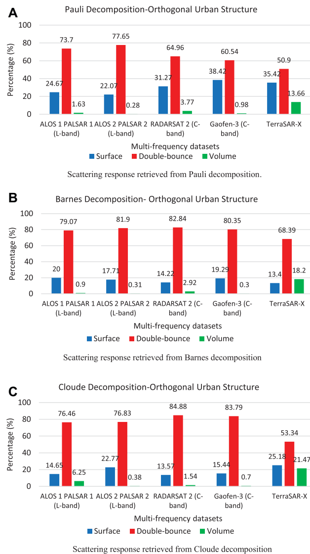
FIGURE 7 | Backscattering response for orthogonal urban structure obtained from Pauli, Barnes, and Cloude decomposition models. (A) Scattering response retrieved from Pauli decomposition. (B) Scattering response retrieved from Barnes decomposition. (C) Scattering response retrieved from Cloude decomposition.
