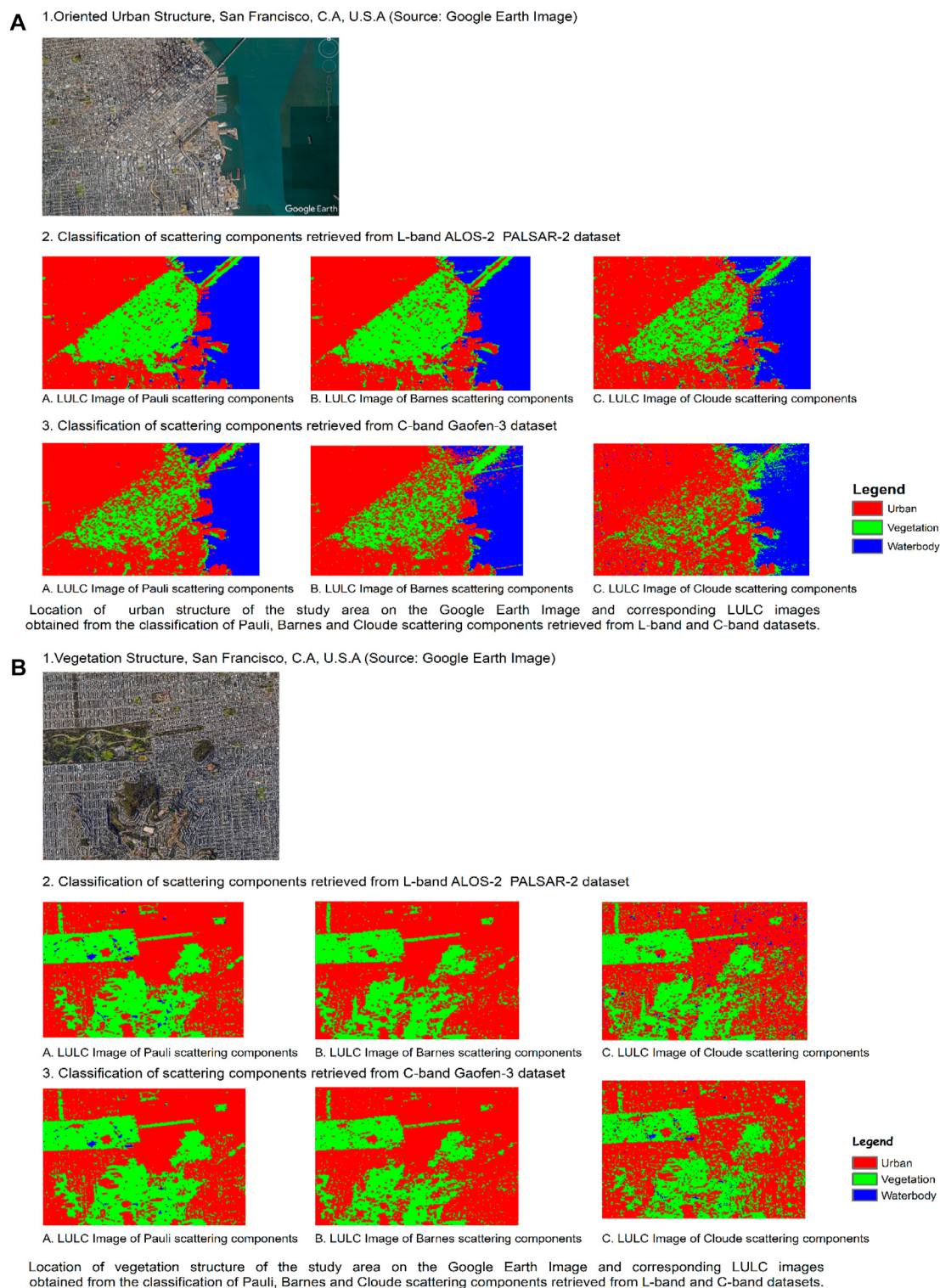
FIGURE 12 | Location of vegetation structure and urban structure of study area on Google Earth Image and corresponding LULC images obtained from classification of Pauli, Barnes, and Cloude scattering components retrieved from L-band and C-band datasets.
