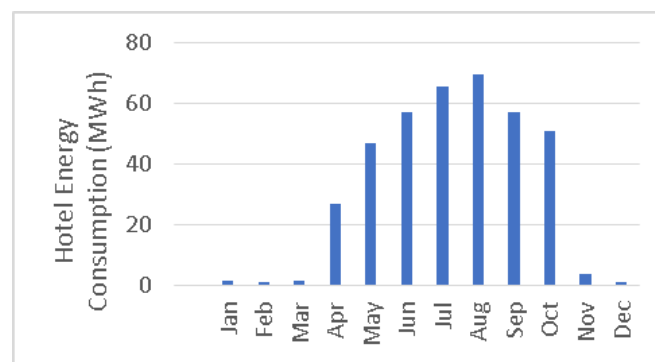
Figure 2. Total electricity consumption recorded during 2019 at the Kolymia Bay Hotel. Data supplied by Volterra [26]. Total annual consumption equates to 385 MWh, with a TAC of EUR 88,550 for an electricity price of 0.23 EUR/kWh.
