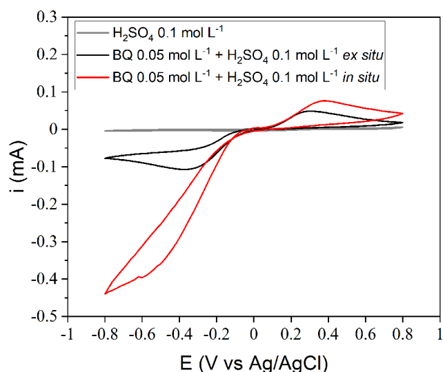
Figure 2. Cyclic voltamograms acquired, using graphite–epoxy composite electrodes, in situ (red line) and ex situ (black line).
