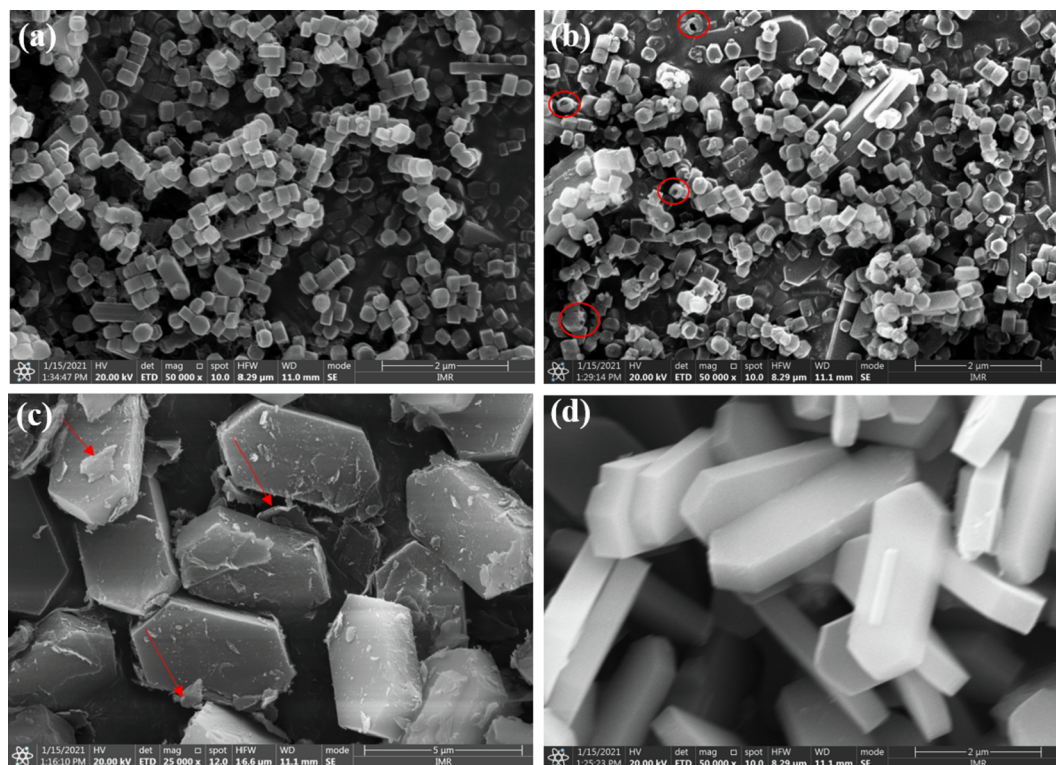
Fig. 2. SEM micrographs of the calcined (a) 5Ni/S-1, (b) 5Ni@hol S-1, (c) 5Ni@EDA-S1 and (d) 5Ni@SiO 2 -S1 catalysts.
