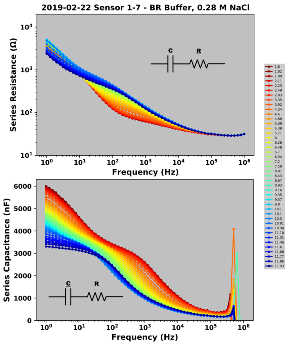
Figure F.4 Series resistance and series capacitance plots for sensor 1-7 in the 0.28 M NaCl buffer, with each pH point color coded from red (acidic) to more basic (blue).
