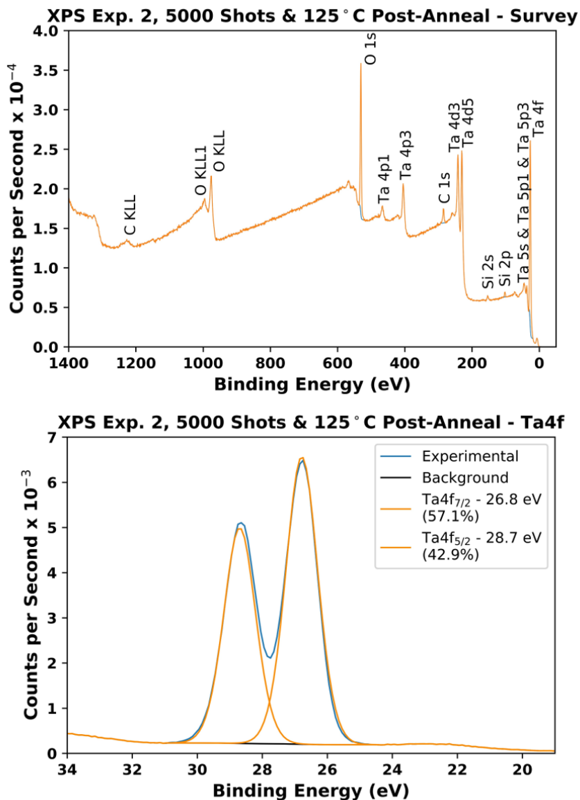
Figure 4.14 XPS after flash lamp annealing followed by another thermal anneal at 125°C.
