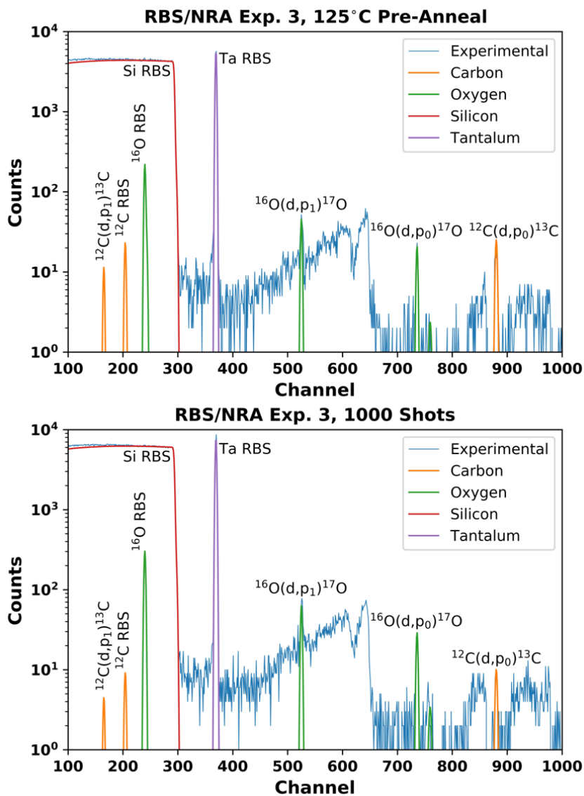
Figure 4.20 RBS/NRA spectra of “125°C pre-anneal” and “1000 shots with pre-anneal” samples (© The Royal Society of Chemistry 2020). 136,137
