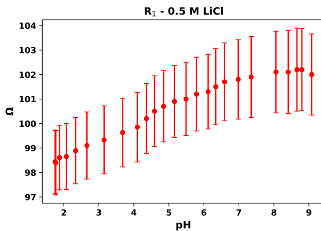
Figure 5.19 R_1 in the simplified, high ionic strength circuit for 0.5 M LiCl, with no clear pH dependence while considering error (© 2022 Elsevier B.V. All rights reserved.). 220
