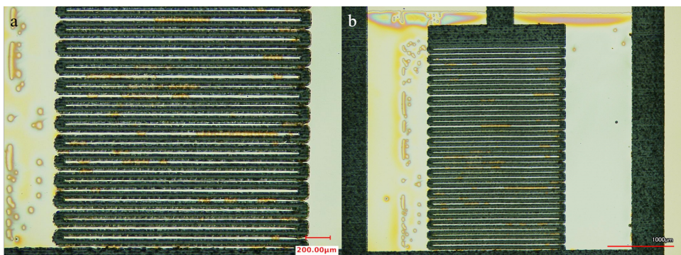
Figure C.7 Sample 7 Firing Parameters (reiteration) - 20x at 2 Hz, 692 \text{ mJ cm}^{-2} , 450 V, 500 \mu\text{s} , 5 \mu\text{pulses} with 50% duty cycle, no capacitance change (a - before flash lamp, b - after flash lamp).
