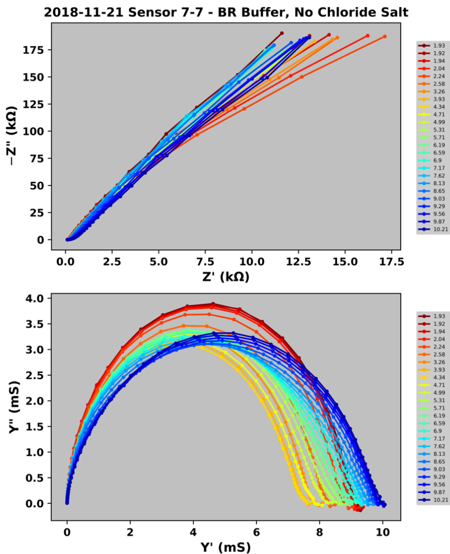
Figure E.5 Nyquist and admittance plots for the “no added chloride salt” buffer, with each pH point color coded from red (acidic) to more basic (blue) ((© 2022 Elsevier B.V. All rights reserved.), 220
