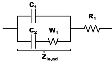
Figure 5.13 Assumed and simplified circuit for high ionic strength solutions. In fitting the simplified circuit to the 0.5 M KCl solution, the C_2 - W_1 branch was omitted, reducing it to C_1 - R_1 and fitting from 100 Hz to 1 MHz.
