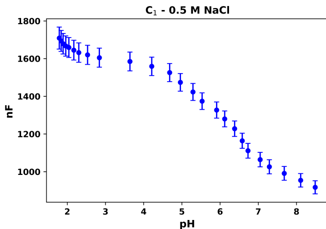
Figure 5.22 C_1 in the simplified, high ionic strength circuit for 0.5 M NaCl, where C_1 appears pH dependent. The C_1 double layer capacitance magnitude for 0.5 M NaCl here appears larger than for 0.5 M LiCl in Figure 5.23 (the opposite is true for C_2 ) (© 2022 Elsevier B.V. All rights reserved.). 220
