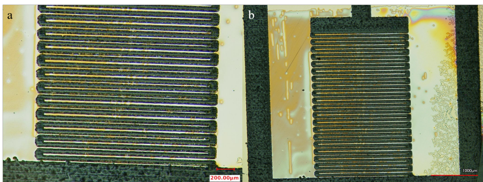
Figure C.10 Sample 10 Firing Parameters (increase shot count) - 1200x at 2 Hz, 739 \text{ mJ cm}^{-2} , 450 V, 500 \mu s, 7 \mu pulses with 50% duty cycle, no capacitance change (a - before flash lamp, b - after flash lamp).
