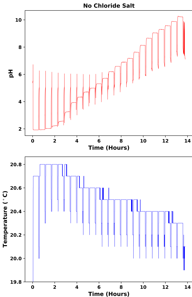
Figure 5.8 pH and temperature for the “no added alkali chloride salt” buffer, with “spikes and dips” between the 30 minute pH measurement intervals being when the pH electrode was removed from the measurement solution (© 2022 Elsevier B.V. All rights reserved.). 220
