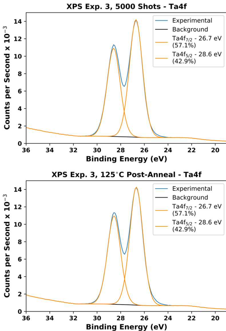
Figure 4.25 XPS Ta 4f spectra of “5000 shots with pre-anneal” and “125°C post-anneal (pre-anneal and 5000 shots before)” samples.
