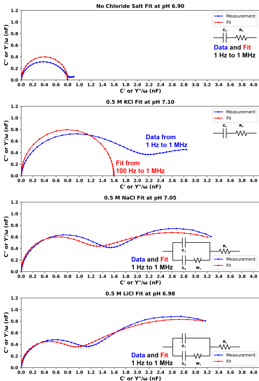
Figure 5.15 Levenberg-Marquardt fit examples for all solutions at roughly pH 7.
