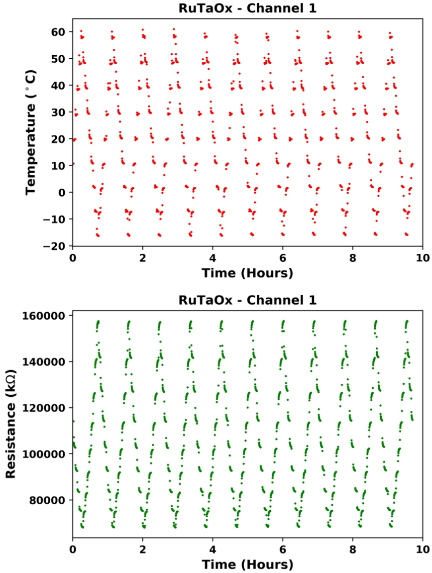
Figure 6.5 Temperature and resistance over time for channel 1 and RuTaOx material from Experiment 2.
