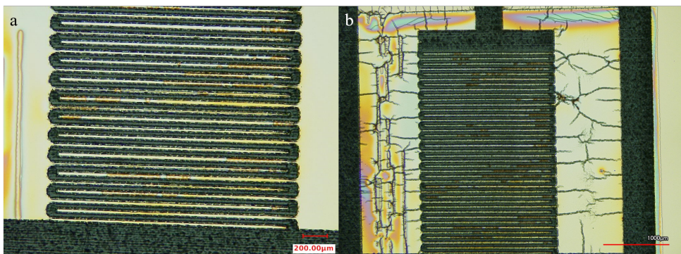
Figure C.1 (Same as Figure 4.2) Sample 1 Firing Parameters - 1 \times 770 \text{ mJ cm}^{-2} , 350 V, 500 \mu\text{s} , 1 undivided pulse, no capacitance change (a - before flash lamp, b - after flash lamp).
