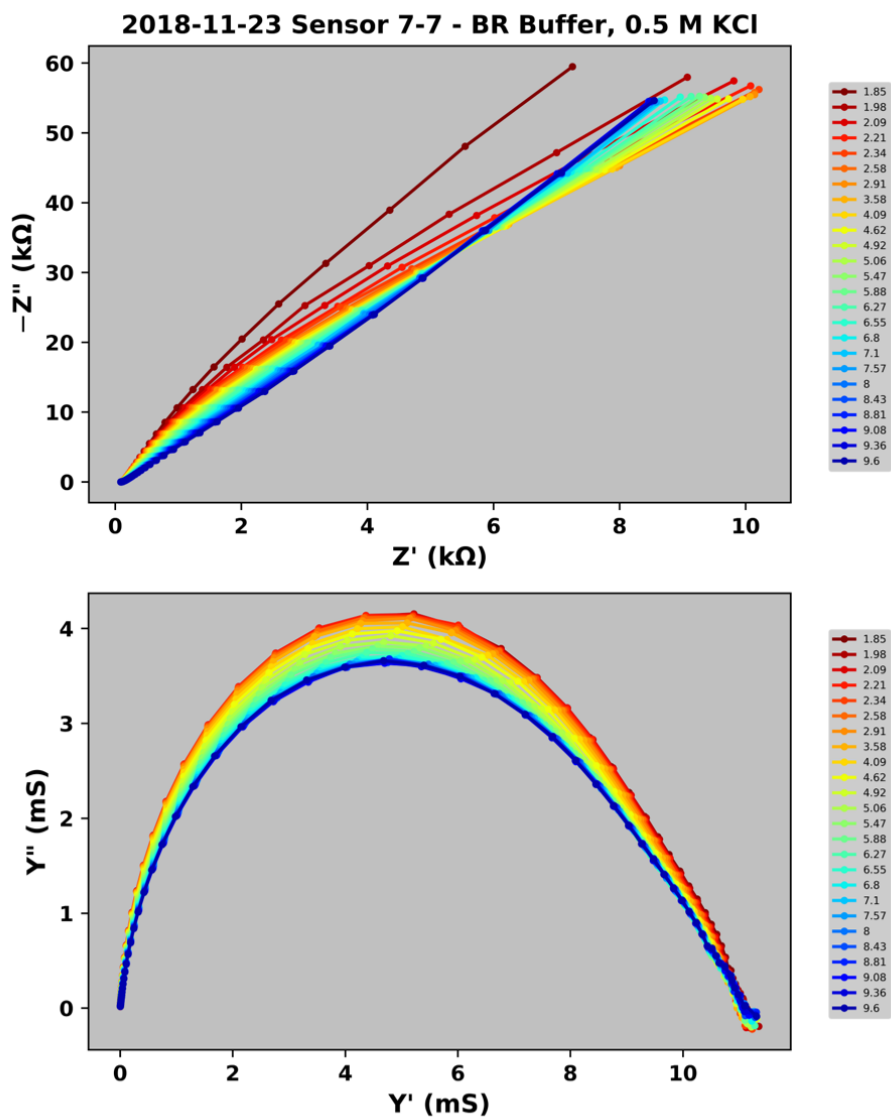
Figure E.6 Nyquist and admittance plots for the 0.5 M KCl buffer, with each pH point color coded from red (acidic) to more basic (blue) (© 2022 Elsevier B.V. All rights reserved.). 220
