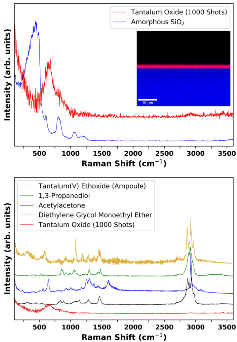
Figure 4.19 Raman spectra of the photocured acetylacetone based film versus a-SiO 2 and solution precursors (© The Royal Society of Chemistry 2020). 136,137
