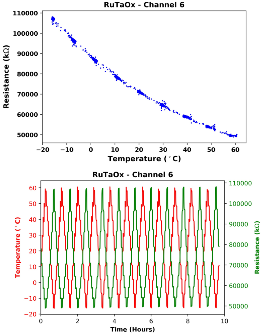
Figure 6.8 Temperature versus resistance for channel 6 and RuTaOx material from Experiment 2.
