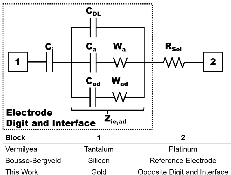
Figure 5.5 Bousse-Bergveld circuit with interfering, specifically adsorbing ions based on prior work from Vermilyea 53,54 and Bousse, Bergveld. 256 C_i is the insulator capacitance, C_{DL} is the double layer capacitance without specific adsorption, C_a is the pH specific adsorption capacitance, W_a is the pH related Warburg element for semi-infinite linear ion diffusion, C_{ad} is the interfering ion specific adsorption capacitance, W_{ad} is the interfering ion related Warburg element, and R_{Sol} is the solution resistance. Additional elements, such as the global capacitance for the interdigitated electrode (IDE) device, 262 were left out for the sake of brevity (© 2022 Elsevier B.V. All rights reserved.). 220
