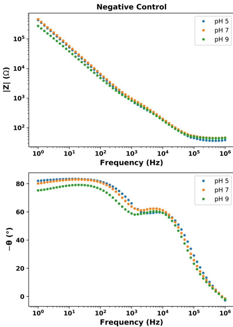
Figure 4.4 Average spectra ( n = 5 ) for pH buffer solution dropped on bare gold electrodes.
