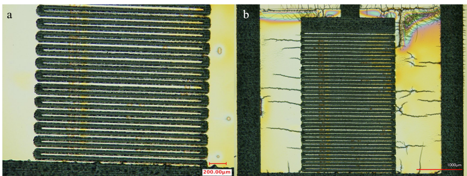
Figure C.5 Sample 5 Firing Parameters (decrease shot envelope) - 20x at 2 Hz, 862 \text{ mJ cm}^{-2} , 450 V, 600 \mu\text{s} , 5 \mu\text{pulses} with 50% duty cycle, no capacitance change (a - before flash lamp, b - after flash lamp).
