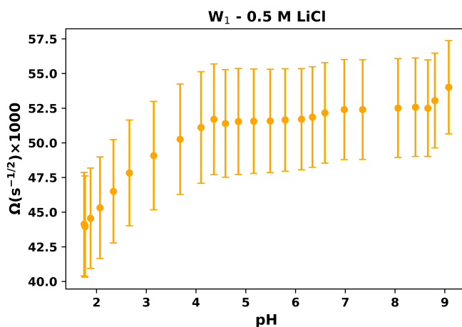
Figure 5.27 W_1 in the simplified, high ionic strength circuit for 0.5 M LiCl, which may increase with pH but with significant error (© 2022 Elsevier B.V. All rights reserved.). 220
