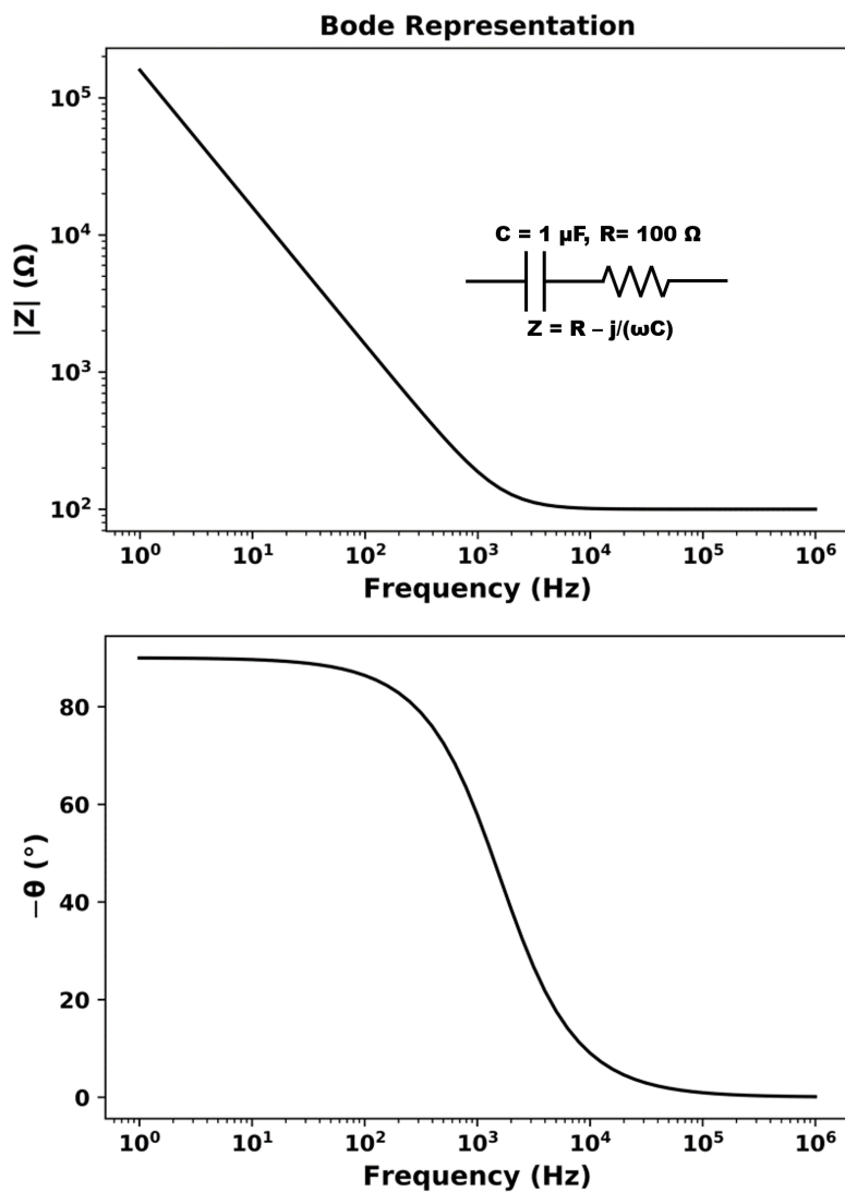
Figure 5.1 Bode plot for a series RC circuit, where R = 100 \Omega and C = 1 \mu\text{F} .
