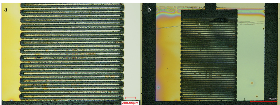
Figure C.6 Sample 6 Firing Parameters (decrease shot envelope) - 20x at 2 Hz, 692 \text{ mJ cm}^{-2} , 450 V, 500 \mu\text{s} , 5 \mu\text{pulses} with 50% duty cycle, no capacitance change (a - before flash lamp, b - after flash lamp).
