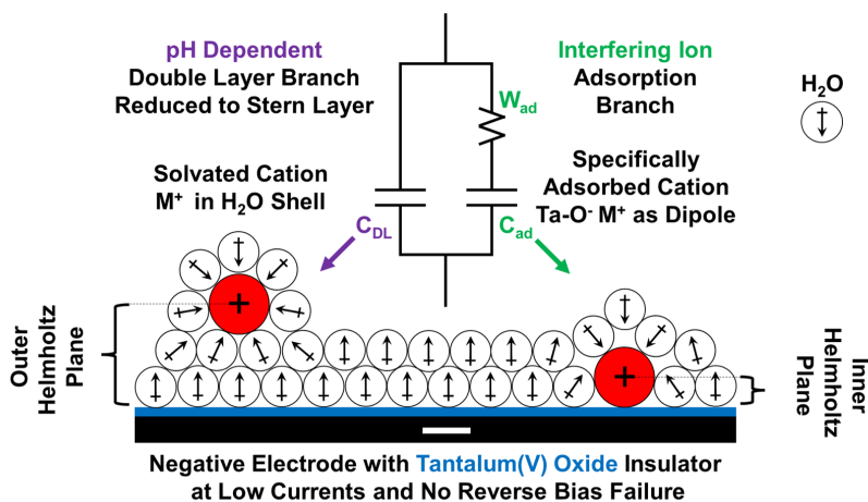
Figure 5.4 Parallel branches of Z_{ie,ad} which omits C_a and reduces C_{DL} to the Stern layer, shown with a simplified illustration of a solvated cation ( M^+ ) in the outer Helmholtz plane for C_{DL} , and a specifically adsorbed cation ( M^+ ) on tantalum(V) oxide in the inner Helmholtz plane for C_{ad} . This illustration was modified and adopted from Bootsma, de Rooij, and van Silfhout 257 (© 2022 Elsevier B.V. All rights reserved.). 220
