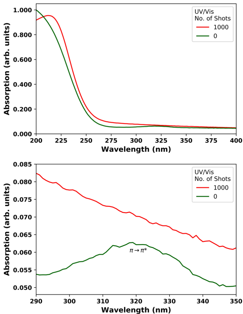
Figure 4.16 UV-Vis absorption spectrum for the acetylacetone based film and different treatments (© The Royal Society of Chemistry 2020). 136,137
