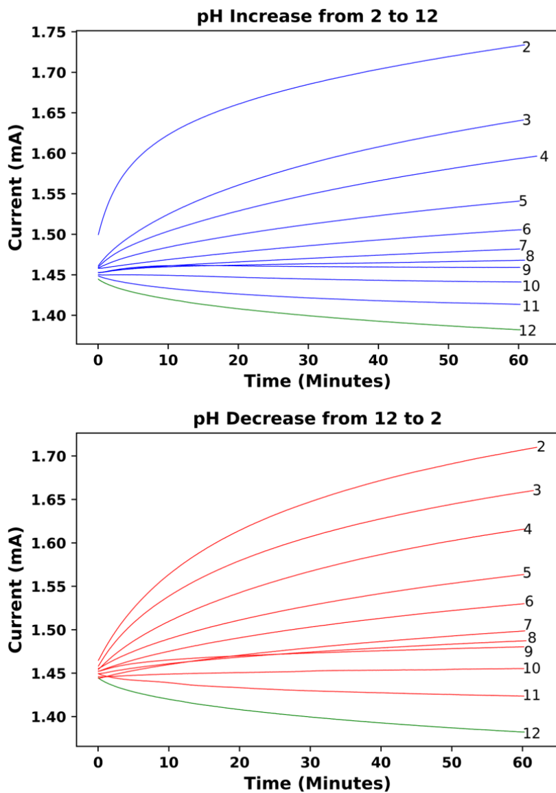
Figure 4.11 Continuous measurement of drain current from pH 2 to pH 12, and back to pH 2 (only one measurement at pH 12). After the 1 hour measuring period, the sensing electrode was rinsed with Milli-Q and N_2 , and the circuit was reset in the new solution (sensing and reference electrodes shorted).
