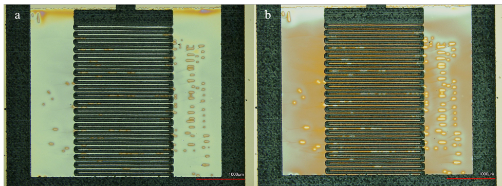
Figure C.13 Sample 13 Firing Parameters (decrease duty cycle) - 2400x at 2 Hz, 663 \text{ mJ cm}^{-2} , 450 V, 500 \mu\text{s} , 7 \mu\text{pulses} with 40% duty cycle, [3.3 pF before, 5.0 pF after, 1.2 pF parasitics] (a - before flash lamp, b - after flash lamp).
