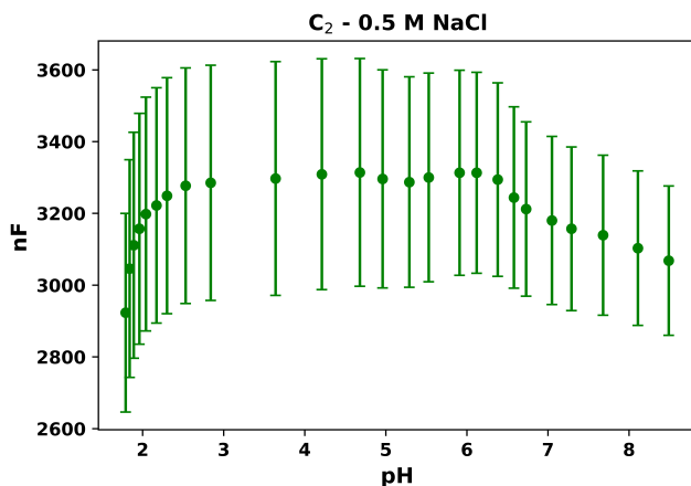
Figure 5.24 C_2 in the simplified, high ionic strength circuit for 0.5 M NaCl, with no clear pH dependence while considering error. The C_2 specific adsorption capacitance magnitude for 0.5 M NaCl here appears smaller than for 0.5 M LiCl in Figure 5.25 (the opposite is true for C_1 ) (© 2022 Elsevier B.V. All rights reserved.). 220
