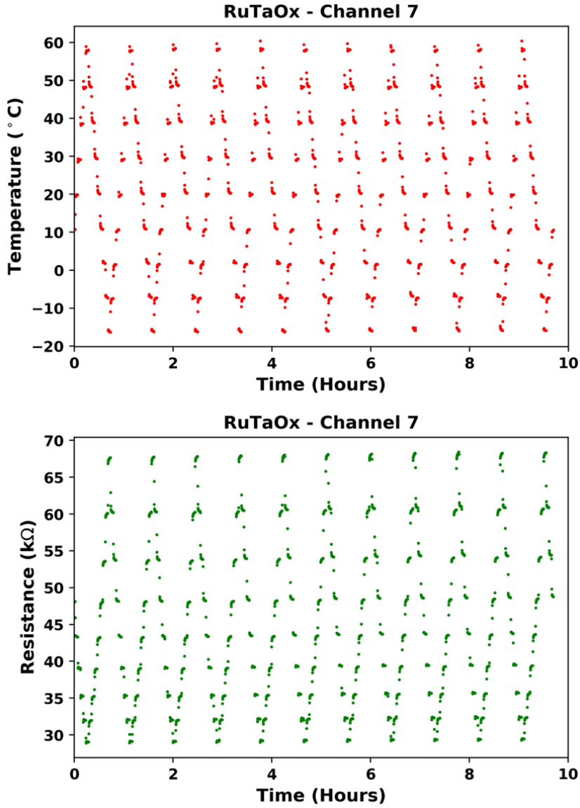
Figure 6.9 Temperature and resistance over time for channel 7 and RuTaOx material from Experiment 2.
