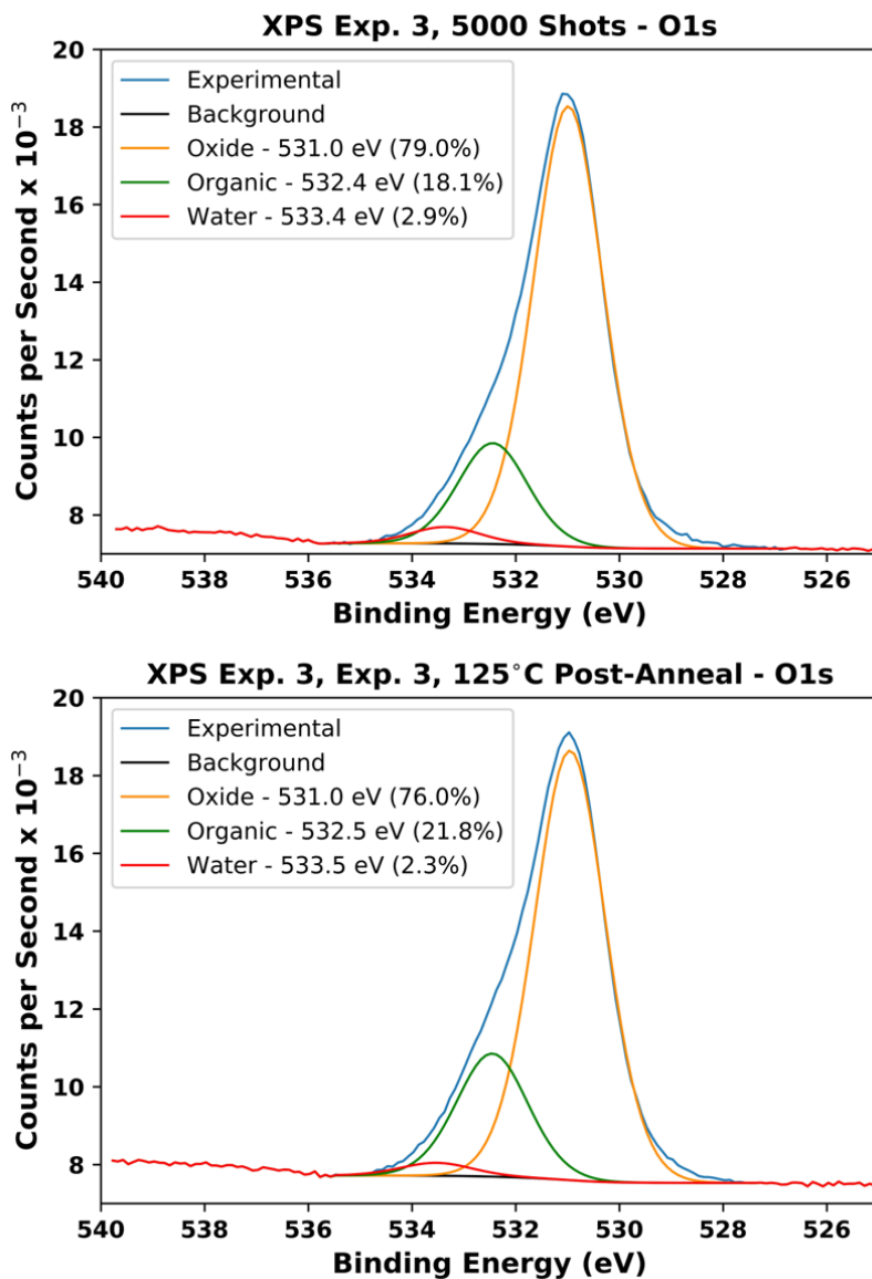
Figure 4.27 XPS O 1s spectra of “5000 shots with pre-anneal” and “125°C post-anneal (pre-anneal and 5000 shots before)” samples.
