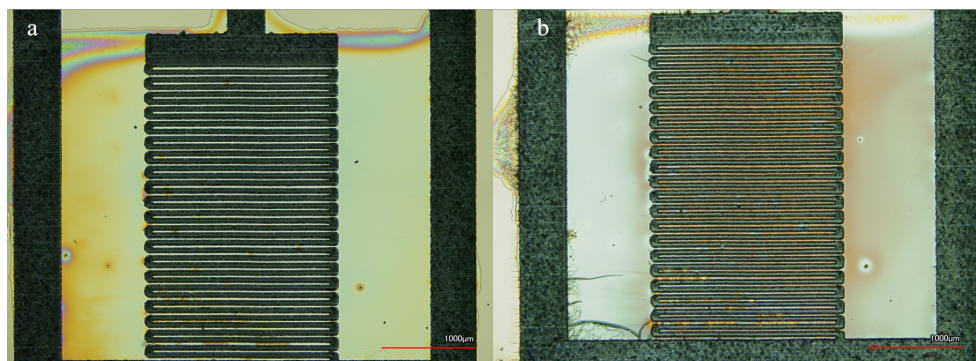
Figure C.11 Sample 11 Firing Parameters ( increase shot count ) - 2400x at 2 Hz, 739 \text{ mJ cm}^{-2} , 450 V, 500 \mu\text{s} , 7 \mu\text{pulses} with 50% duty cycle, [3.4 pF before, 4.2 pF after, 1.2 pF parasitics] (a - before flash lamp, b - after flash lamp).
