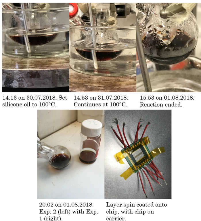
Figure 6.4 Synthesis and fabrication of temperature sensors for Experiment 2.
