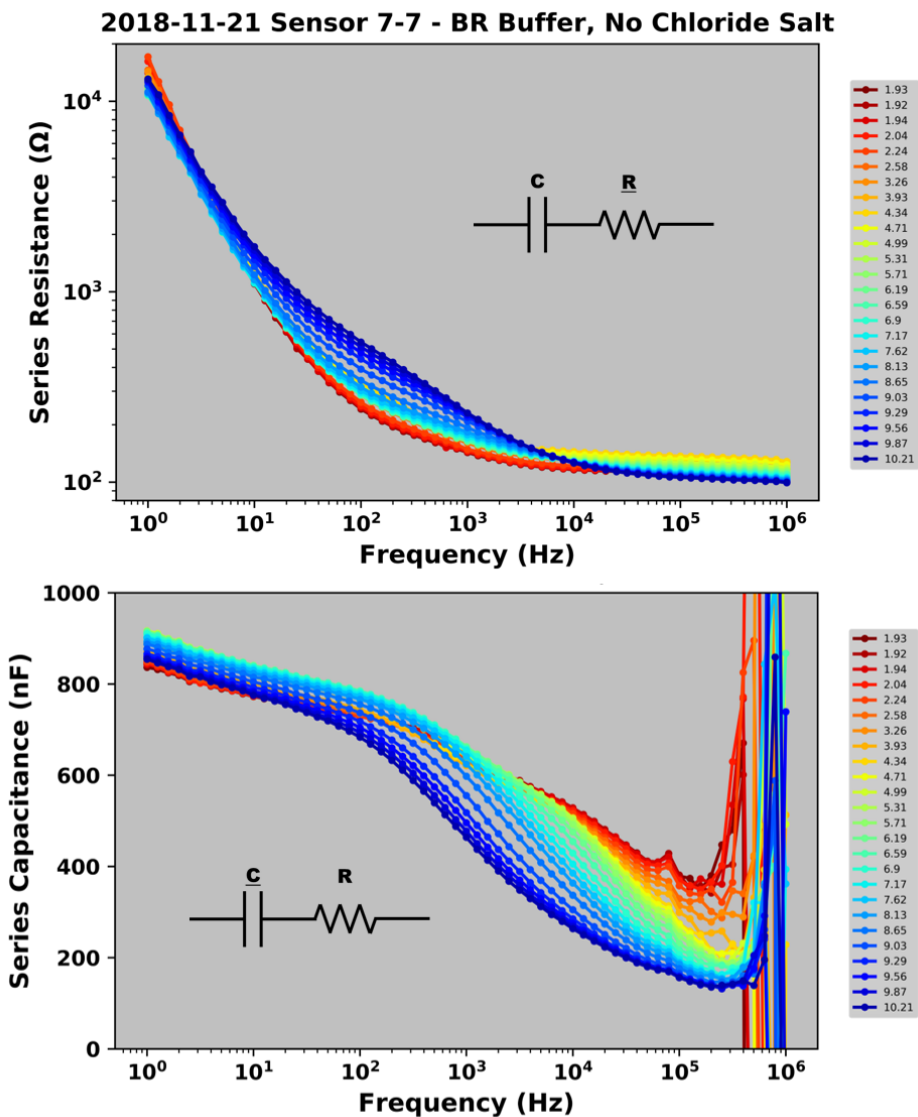
Figure E.9 Series resistance and series capacitance plots for the “no added chloride salt” buffer, with each pH point color coded from red (acidic) to more basic (blue) (© 2022 Elsevier B.V. All rights reserved.). 220
