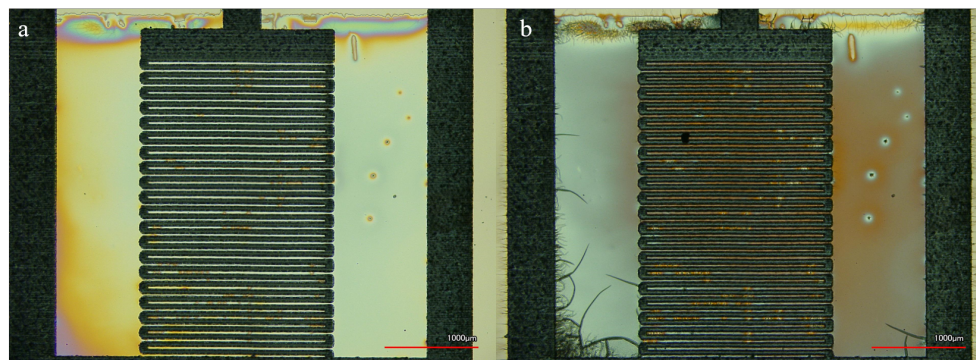
Figure C.12 Sample 12 Firing Parameters (reiteration) - 2400x at 2 Hz, 739 \text{ mJ cm}^{-2} , 450 V, 500 \mu\text{s} , 7 \mu\text{pulses} with 50% duty cycle, [3.5 pF before, 4.3 pF after, 1.2 pF parasitics] (a - before flash lamp, b - after flash lamp).
