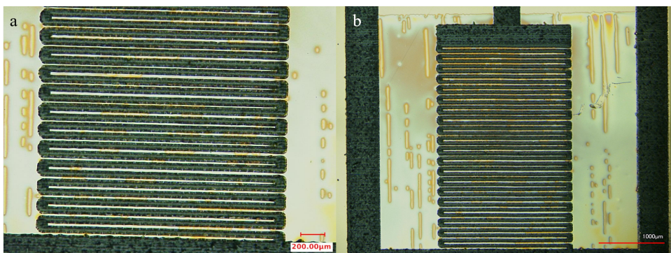
Figure C.9 Sample 9 Firing Parameters (add \mu pulses) - 120x at 2 Hz, 739 \text{ mJ cm}^{-2} , 450 V, 500 \mu s, 7 \mu pulses with 50% duty cycle, no capacitance change (a - before flash lamp, b - after flash lamp).
