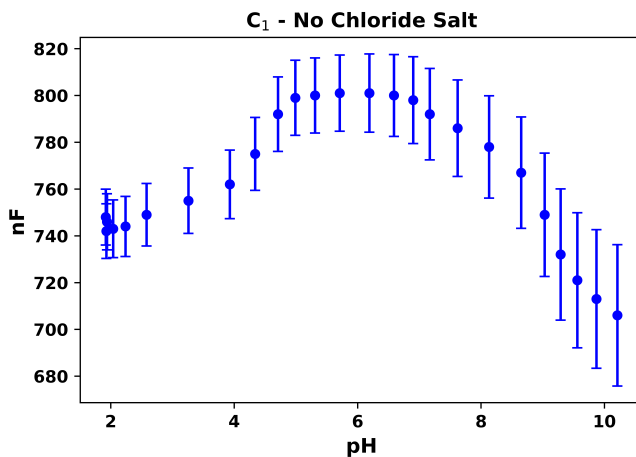
Figure 5.20 C 1 in series with R 1 for “no added alkali chloride salt” solution, where C 1 peaks around pH 6 but with significant error.
