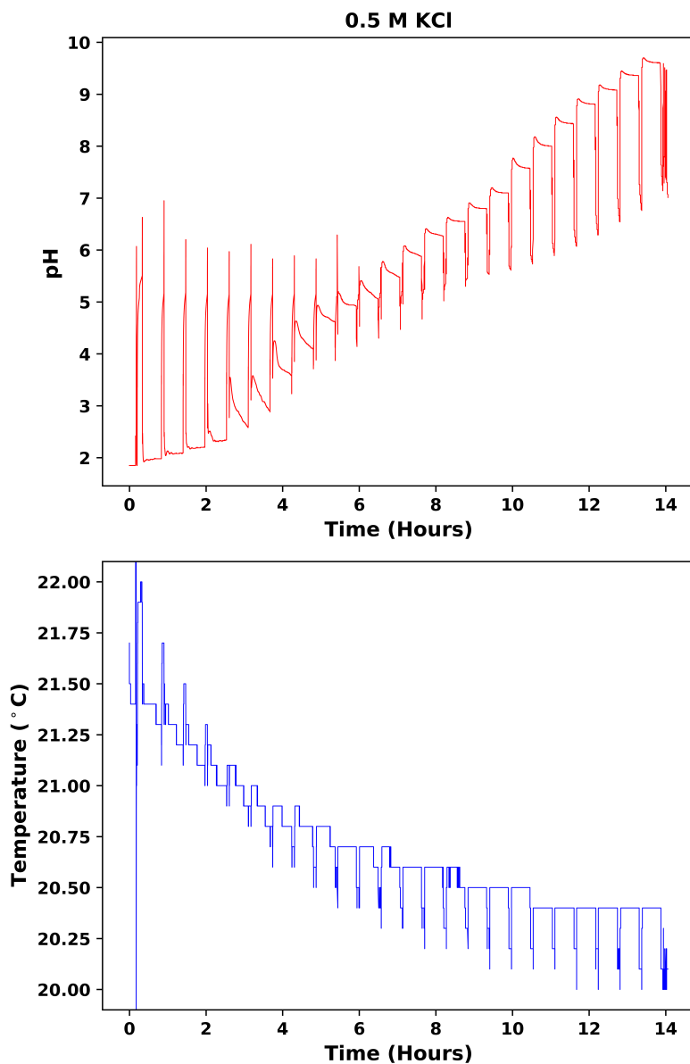
Figure 5.9 pH and temperature for the 0.5 M KCl buffer, with “spikes and dips” between the 30 minute pH measurement intervals being when the pH electrode was removed from the measurement solution (© 2022 Elsevier B.V. All rights reserved.). 220
