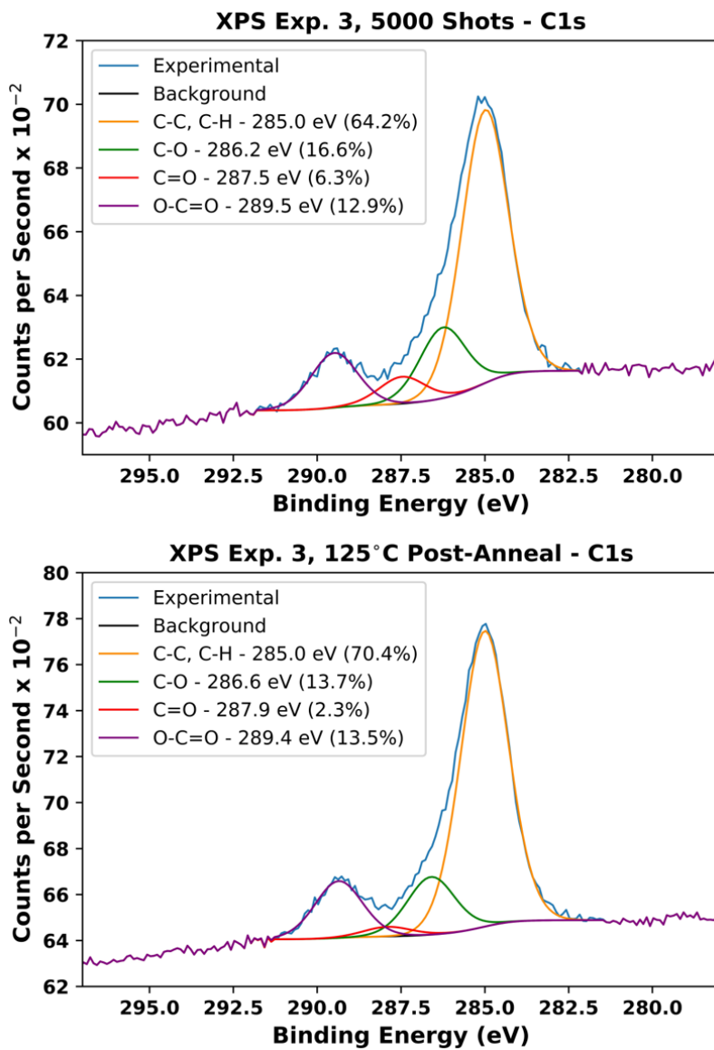
Figure 4.29 XPS C 1s spectra of “5000 shots with pre-anneal” and “125°C post-anneal (pre-anneal and 5000 shots before)” samples.
