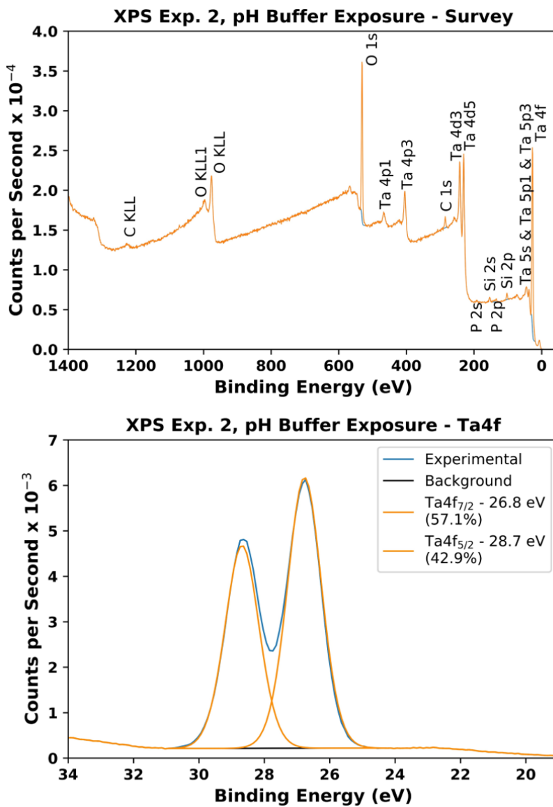
Figure 4.15 XPS after 24 hour pH buffer exposure and EGFET measurement.
