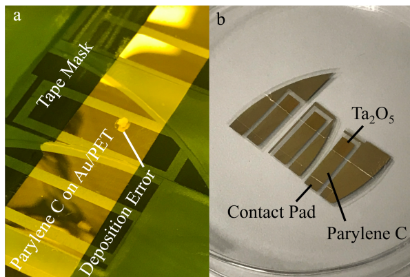
Figure 4.9 Tape mask on tantalum oxide and contact pads after parylene C deposition (a) and tape mask removal (b).
