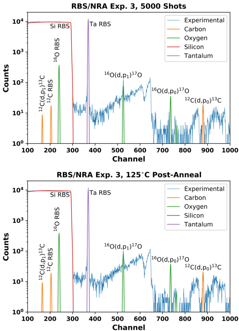
Figure 4.21 RBS/NRA spectra of “5000 shots with pre-anneal” and “125°C post-anneal (pre-anneal and 5000 shots before)” samples.
