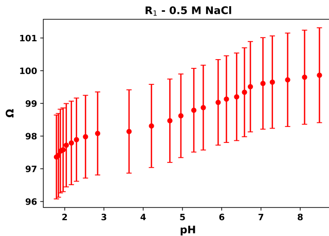
Figure 5.18 R_1 in the simplified, high ionic strength circuit for 0.5 M NaCl, with no clear pH dependence while considering error (© 2022 Elsevier B.V. All rights reserved.). 220
