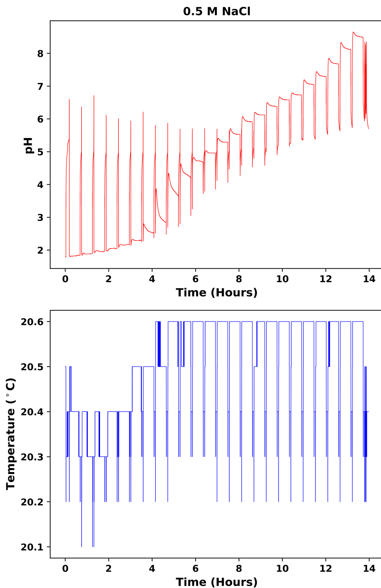
Figure 5.10 pH and temperature for the 0.5 M NaCl buffer, with “spikes and dips” between the 30 minute pH measurement intervals being when the pH electrode was removed from the measurement solution (© 2022 Elsevier B.V. All rights reserved.). 220
