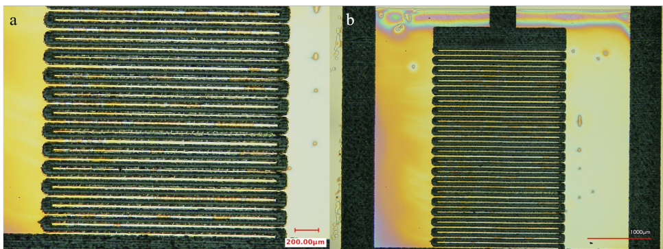
Figure C.3 Sample 3 Firing Parameters ( increase shot count ) - 20x at 2 Hz, 558 \text{mJ cm}^{-2} , 450 V, 400 \mu\text{s} , 5 \mu\text{pulses} with 50% duty cycle, no capacitance change (a - before flash lamp, b - after flash lamp).
