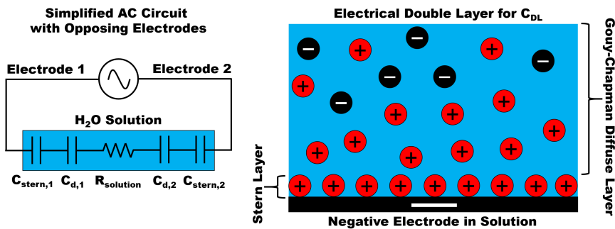
Figure 5.3 Simplified AC circuit for two opposing and chemically inert electrodes in solution, along with a simplified illustration (ignoring the solvation shells and water molecules) of the series combination of the Gouy-Chapman diffuse layer (described with Boltzmann statistics) with the condensed Stern layer. 255
