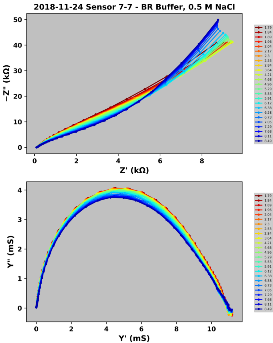
Figure E.7 Nyquist and admittance plots for the 0.5 M NaCl buffer, with each pH point color coded from red (acidic) to more basic (blue) (© 2022 Elsevier B.V. All rights reserved.). 220
