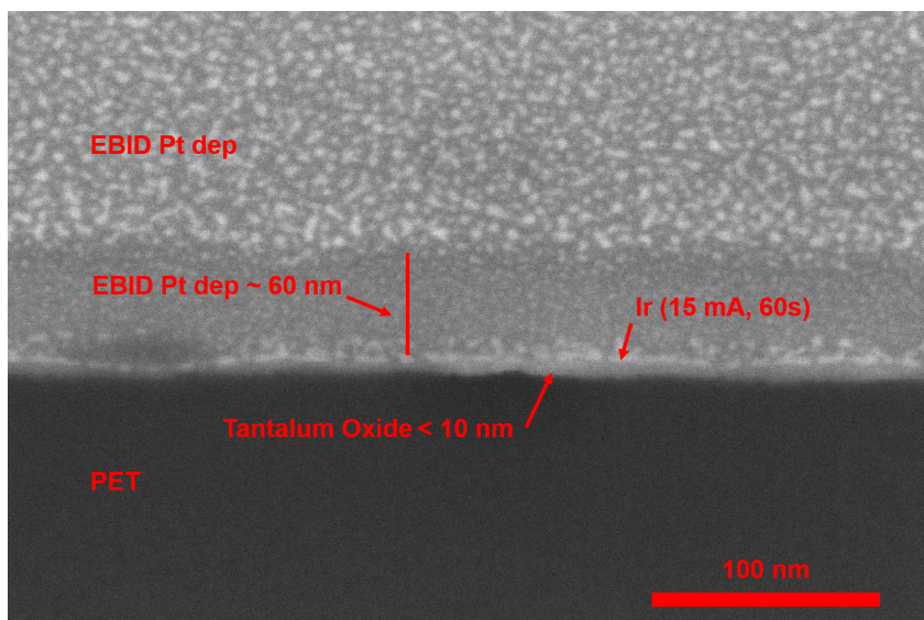
Figure 4.31 FIB/SEM of a sample exposed to a 125°C pre-anneal, 5000 flash lamp shots, and a 125°C post-anneal (© The Royal Society of Chemistry 2020). 136,137
