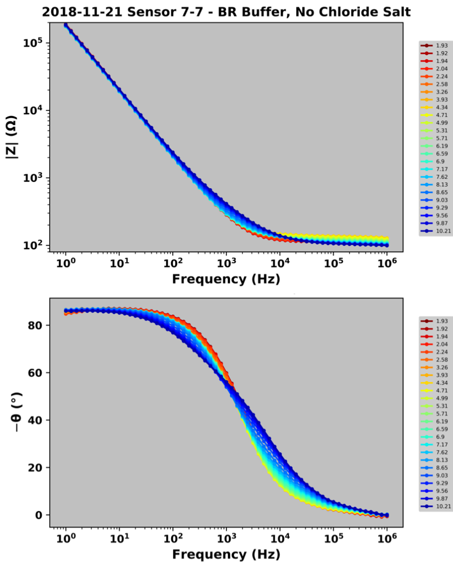
Figure E.1 Bode plot for the “no added chloride salt” buffer, with each pH point color coded from red (acidic) to more basic (blue) (© 2022 Elsevier B.V. All rights reserved.). 220
