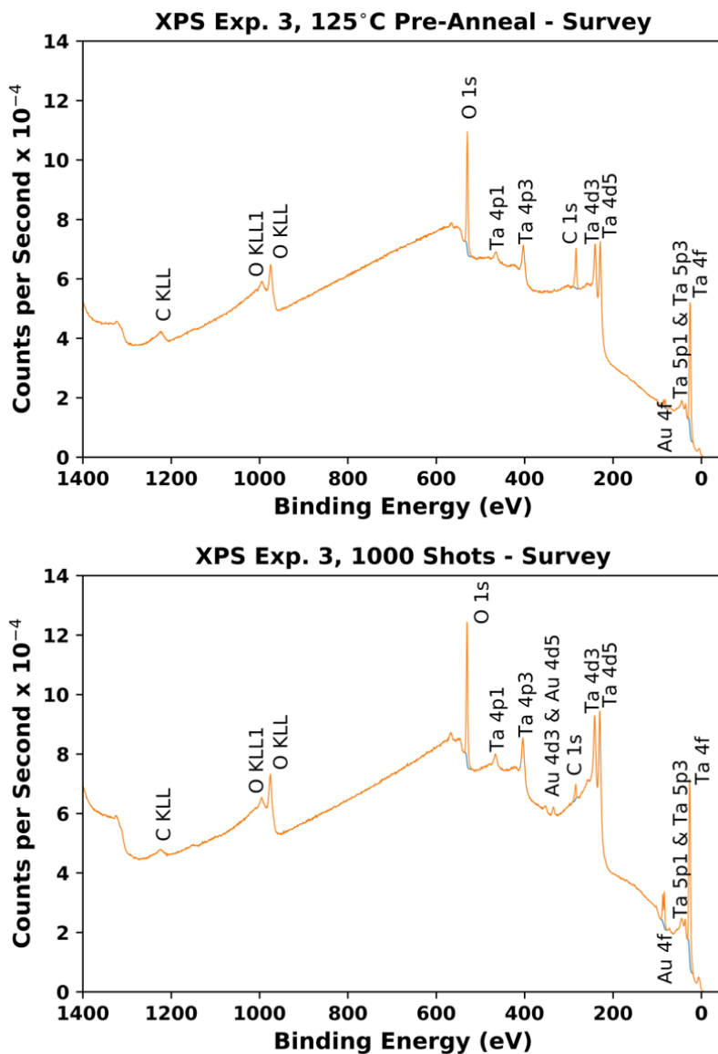
Figure 4.22 XPS survey spectra of “125°C pre-anneal” and “1000 shots with pre-anneal” samples (© The Royal Society of Chemistry 2020). 136,137
