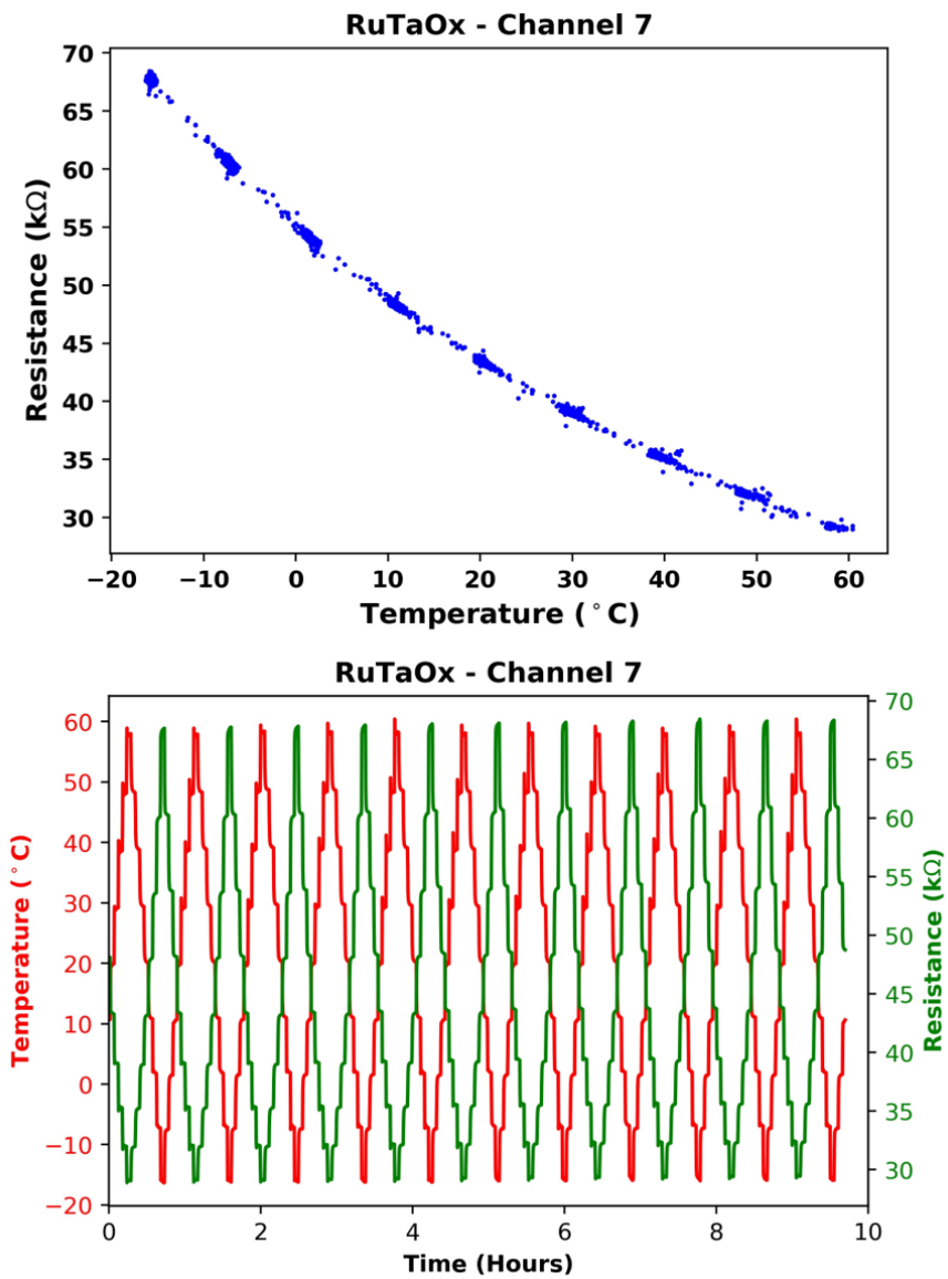
Figure 6.10 Temperature versus resistance for channel 7 and RuTaOx material from Experiment 2.
