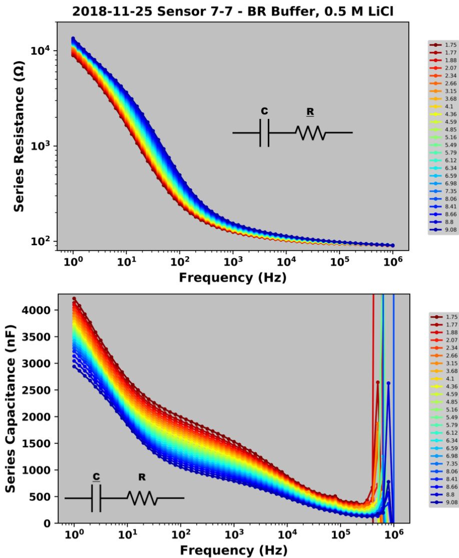
Figure E.12 Series resistance and series capacitance plots for the 0.5 M LiCl buffer, with each pH point color coded from red (acidic) to more basic (blue) (© 2022 Elsevier B.V. All rights reserved.). 220
