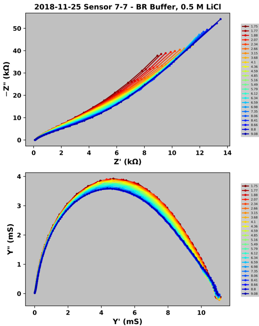
Figure E.8 Nyquist and admittance plots for the 0.5 M LiCl buffer, with each pH point color coded from red (acidic) to more basic (blue) (© 2022 Elsevier B.V. All rights reserved.). 220
