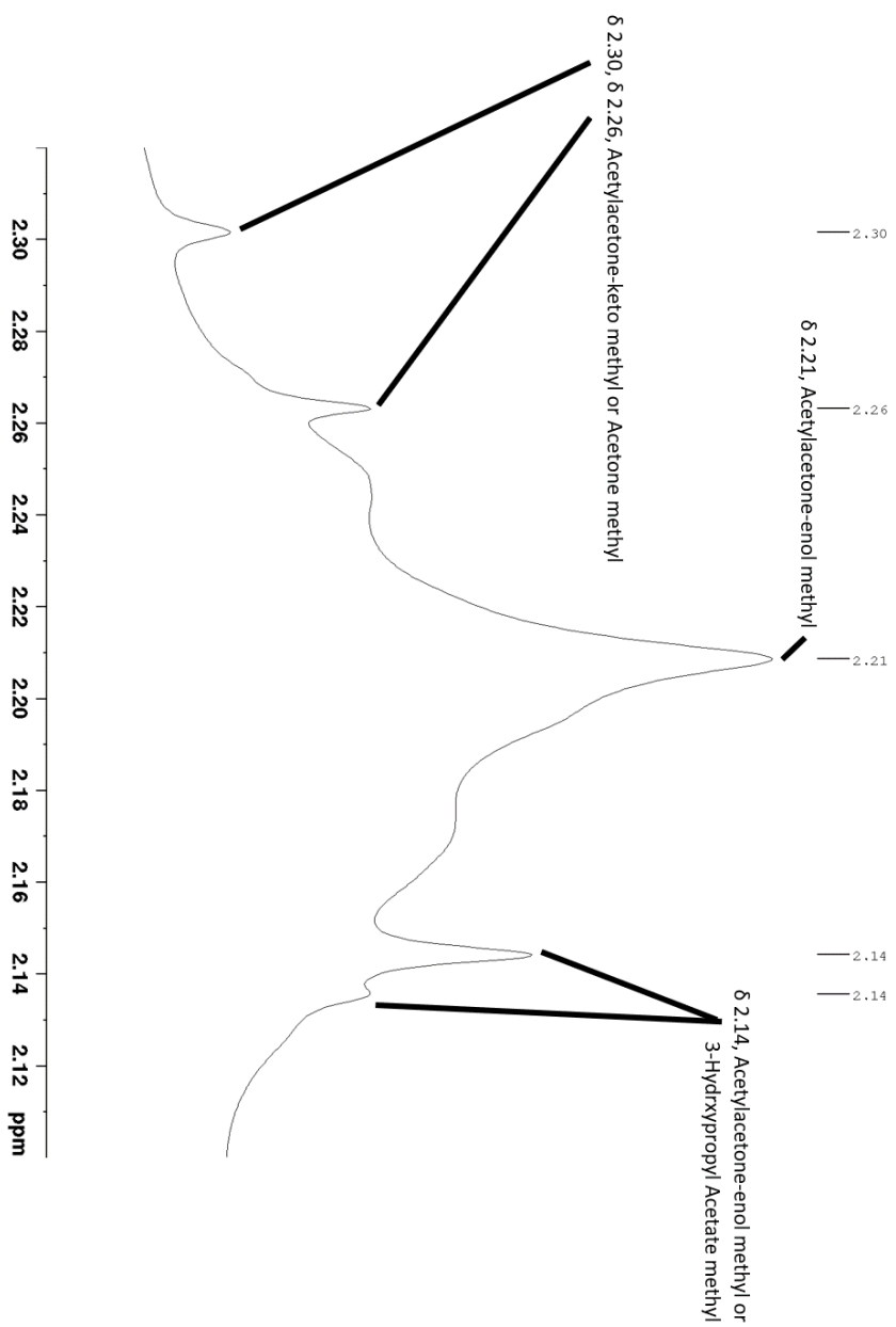
Figure 3.32 ^1\text{H} NMR [External \text{D}_2\text{O} ]: Experiment 4 – Product (( \text{C} ) The Royal Society of Chemistry 2020). 136,137
