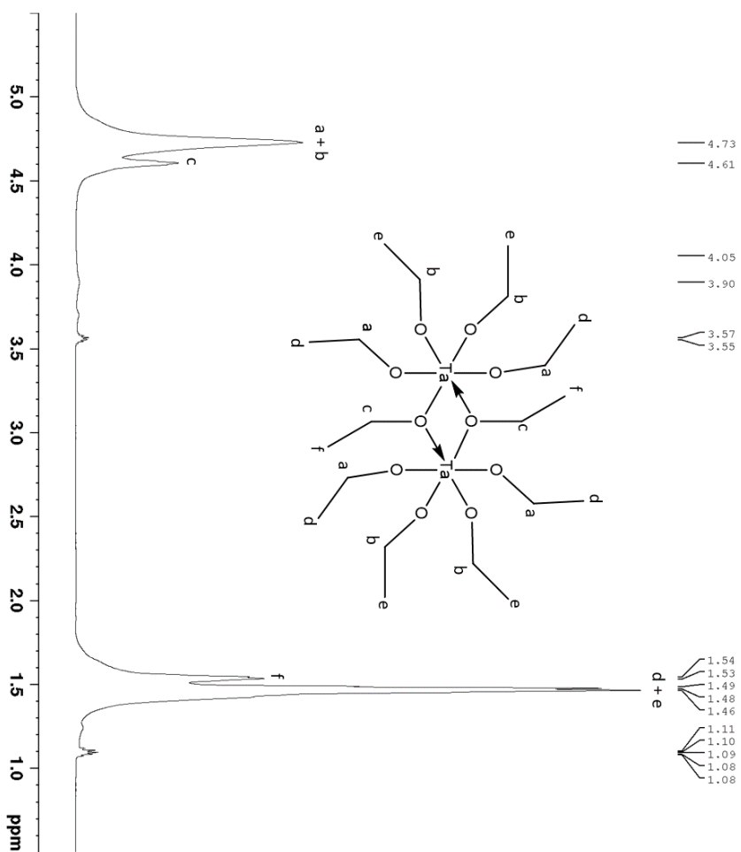
Figure 3.1 ^1\text{H} NMR [External \text{D}_2\text{O} ]: Tantalum(V) Ethoxide [Alfa Aesar, 99+%,] (© The Royal Society of Chemistry 2020). 136,137
