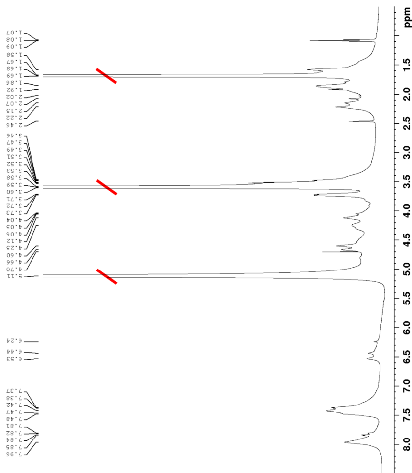
Figure 3.38 ^1\text{H} NMR [External \text{D}_2\text{O} ]: Experiment 5 – Product (© The Royal Society of Chemistry 2020). 136,137
