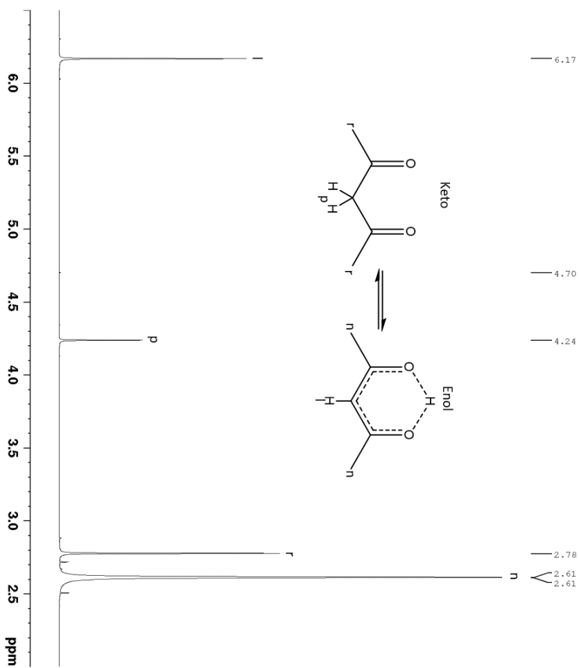
Figure 3.5 ^1\text{H} NMR [External \text{D}_2\text{O} ]: Acetylacetone [Alfa Aesar, 95%] (© The Royal Society of Chemistry 2020). 136,137
