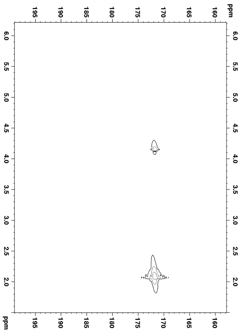
Figure 3.14 HMBC [External D 2 O]: Experiment 1 – Product.
