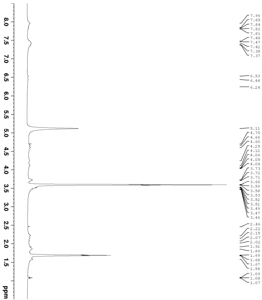
Figure 3.37 ^1\text{H} NMR [External \text{D}_2\text{O} ]: Experiment 5 – Product (© The Royal Society of Chemistry 2020). 136,137
