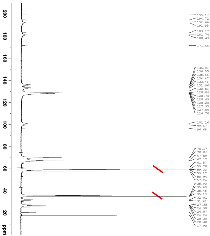
Figure 3.39 ^{13}\text{C} NMR [ \text{External D}_2\text{O} ]: Experiment 5 – Product (© The Royal Society of Chemistry 2020). ^{136,137}
