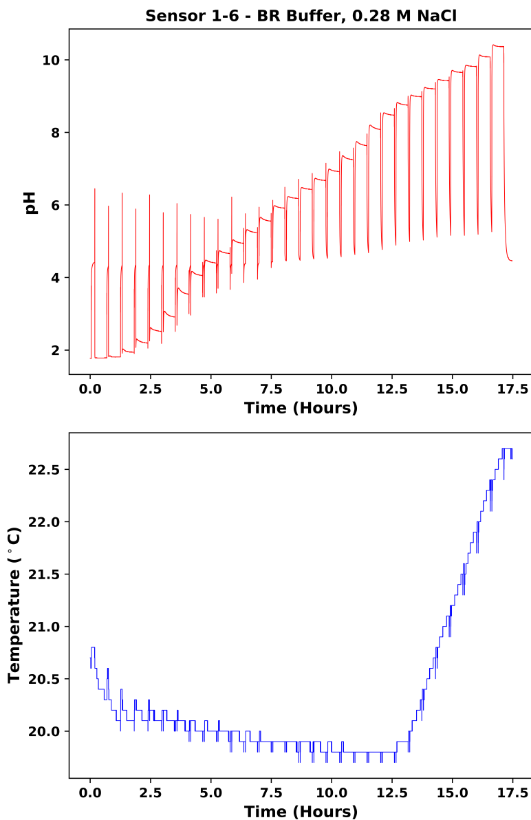
Figure F.5 pH and temperature for sensor 1-6 in 0.28 M NaCl buffer, with “spikes and dips” between the 30 minute pH measurement intervals being when the pH electrode was removed from the measurement solution.
