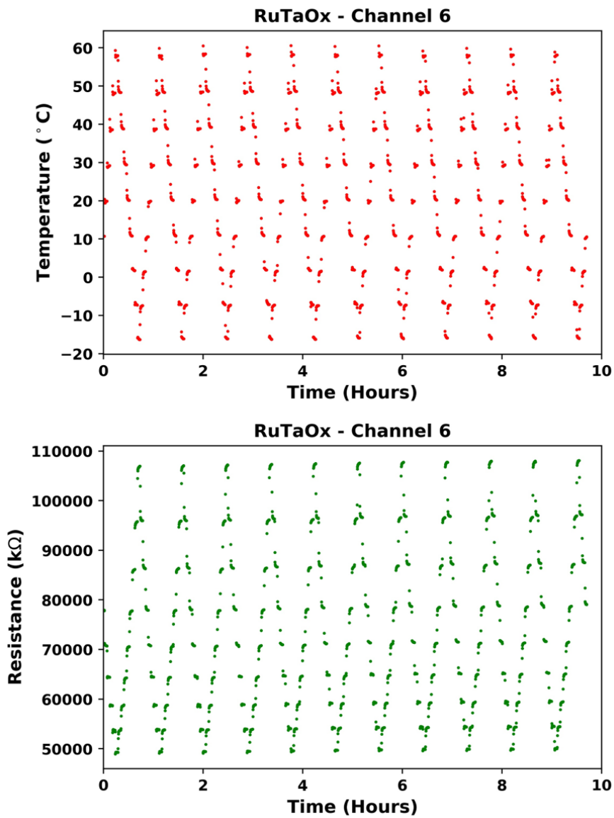
Figure 6.7 Temperature and resistance over time for channel 6 and RuTaOx material from Experiment 2.
