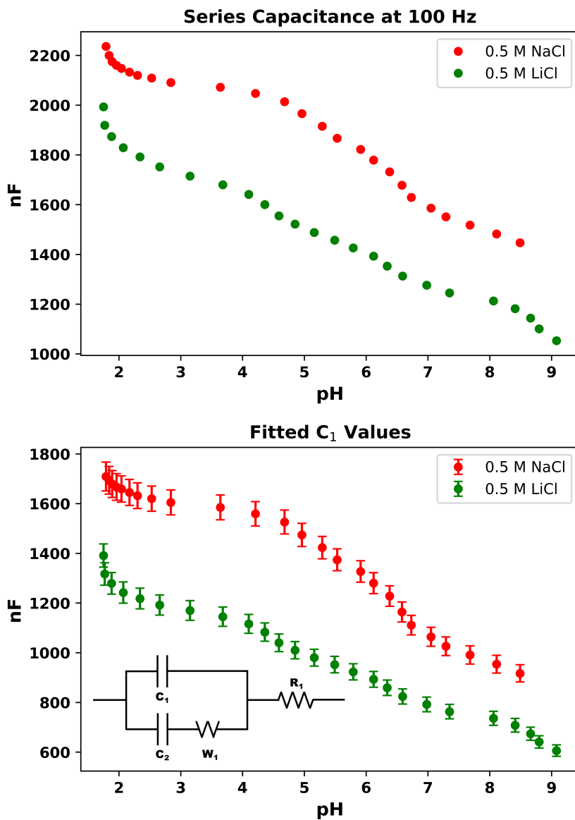
Figure 5.29 Series capacitance at 100 Hz for \text{Na}^+ and \text{Li}^+ solutions, compared with C_1 values from Figure 5.22 for \text{Na}^+ and Figure 5.23 for \text{Li}^+ , where similar behavior occurs (© 2022 Elsevier B.V. All rights reserved.). 220
