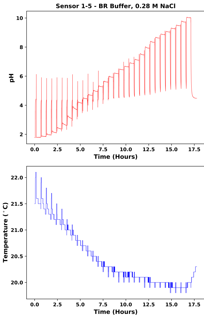
Figure F.7 pH and temperature for sensor 1-5 in 0.28 M NaCl buffer, with “spikes and dips” between the 30 minute pH measurement intervals being when the pH electrode was removed from the measurement solution.
