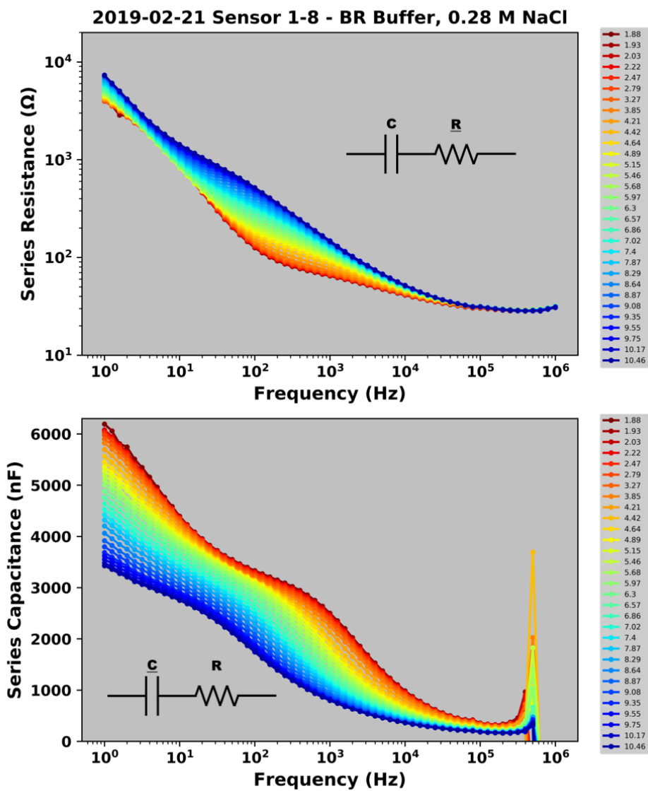
Figure F.2 Series resistance and series capacitance plots for sensor 1-8 in the 0.28 M NaCl buffer, with each pH point color coded from red (acidic) to more basic (blue).
