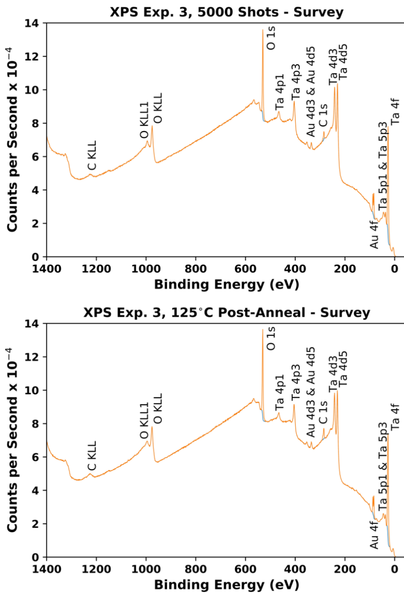
Figure 4.23 XPS survey spectra of “5000 shots with pre-anneal” and “125°C post-anneal (pre-anneal and 5000 shots before)” samples.
