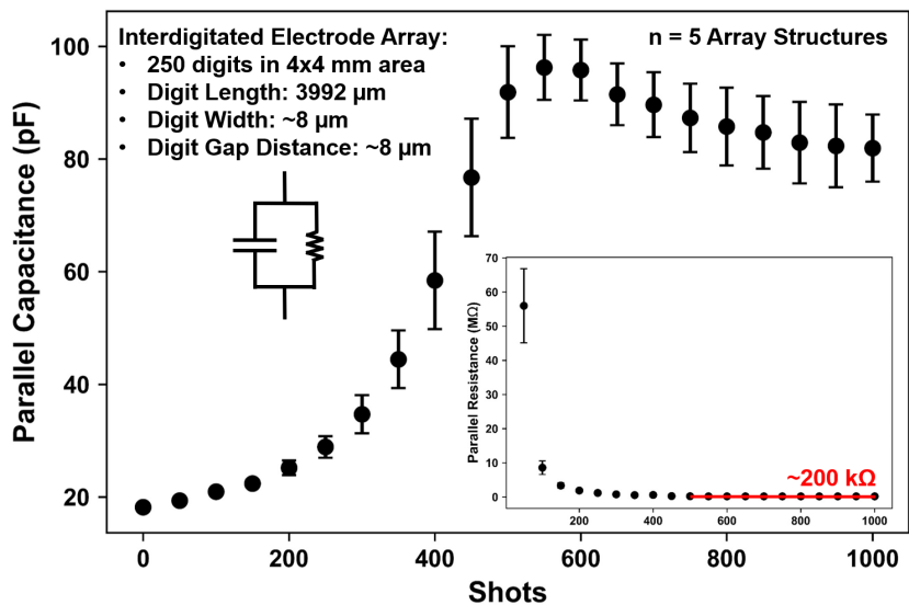
Figure 4.30 Parallel capacitance and parallel resistance measured with an LCR meter (© The Royal Society of Chemistry 2020). 136,137
