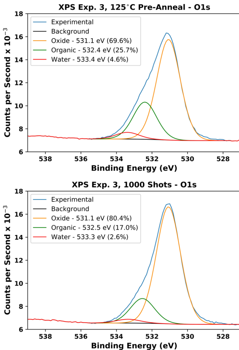
Figure 4.26 XPS O 1s spectra of “125°C pre-anneal” and “1000 shots with pre-anneal” samples (© The Royal Society of Chemistry 2020). 136,137
