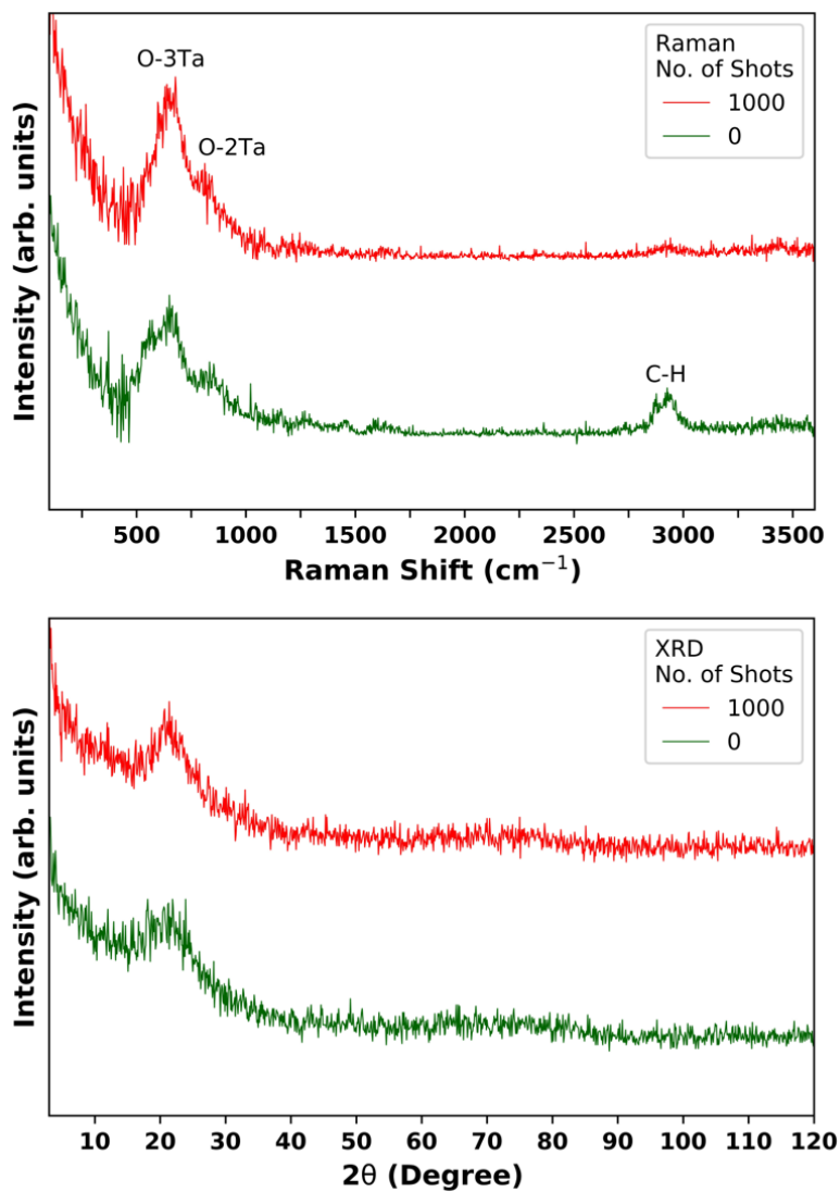
Figure 4.18 Raman and XRD spectra for the acetylacetone based film and different treatments (© The Royal Society of Chemistry 2020). 136,137
