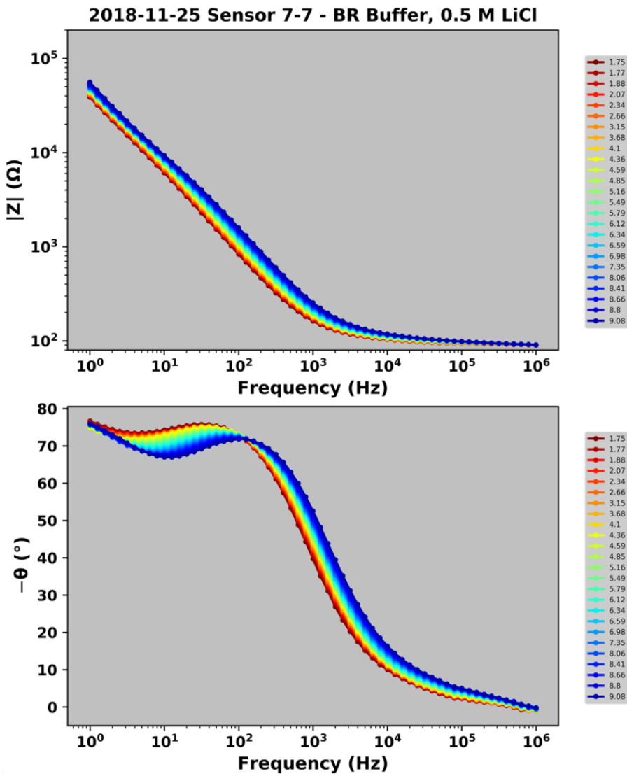
Figure E.4 Bode plot for the 0.5 M LiCl buffer, with each pH point color coded from red (acidic) to more basic (blue) (© 2022 Elsevier B.V. All rights reserved.). 220
