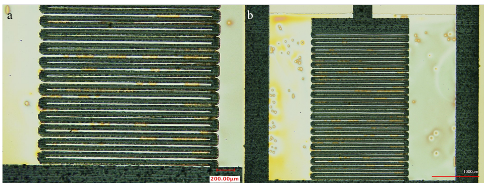
Figure C.8 Sample 8 Firing Parameters ( increase shot count ) - 120x at 2 Hz, 692 \text{ mJ cm}^{-2} , 450 V, 500 \mu\text{s} , 5 \mu\text{pulses} with 50% duty cycle, no capacitance change (a - before flash lamp, b - after flash lamp).
