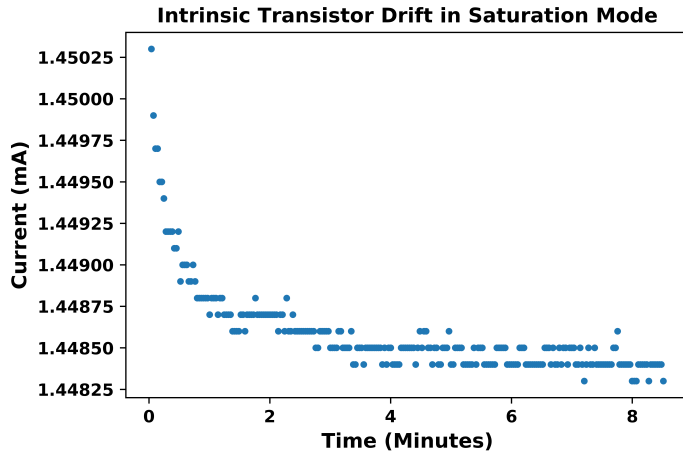
Figure D.1 I_{DS} over time in saturation mode with the gate connected directly to the analyzer, with biases of V_{GS} = 3 V and V_{DS} = 5 V. The intrinsic drift is less than 0.001 \text{ mA min}^{-1} , which is much lower than when measuring with \text{Ta}_2\text{O}_5 .
