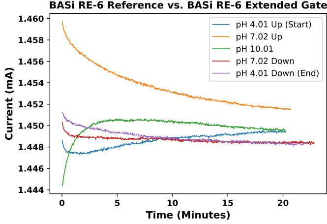
Figure D.2 I_{DS} over time in saturation mode with two BASi RE-6 reference electrodes (one as the extended-gate, and one as the reference in Britton-Robinson buffer solution), with biases of V_{GS} = 3 V and V_{DS} = 5 V. The measurement was started in pH = 4, then pH = 7, then pH = 10, then pH 7 again, then finally pH 4 again. The drift in all cases is less than 0.0004 \text{ mA min}^{-1} , which is much lower than when measuring with \text{Ta}_2\text{O}_5 .
