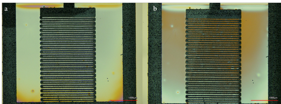
Figure C.14 (Same as Figure 4.3) Sample 14 Firing Parameters (reiteration) - 2400x at 2 Hz, 663 \text{ mJ cm}^{-2} , 450 V, 500 \mu\text{s} , 7 \mu\text{pulses} with 40% duty cycle, [3.5 pF before, 5.0 pF after, 1.2 pF parasitics] (a - before flash lamp, b - after flash lamp).
