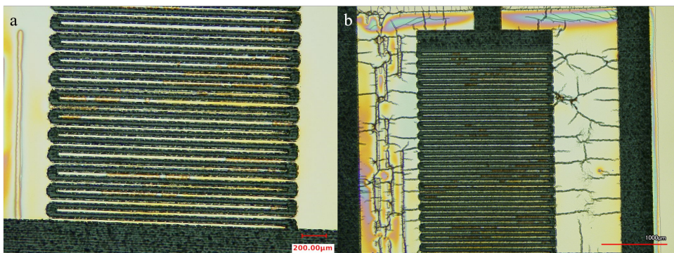
Figure 4.2 Sample 1 Firing Parameters - 1 \times 770 \text{ mJ cm}^{-2} , 350 V, 500 \mu\text{s} , 1 undivided pulse, no capacitance change (a - before flash lamp, b - after flash lamp).
