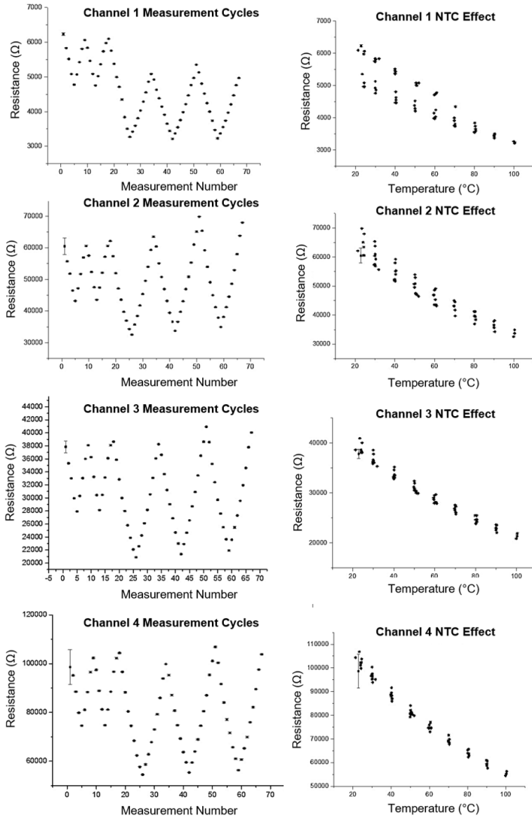
Figure 6.2 Manual temperature measurements on a hot plate for RuTaOx material from Experiment 1. Resistance taken as the impedance at 100 Hz (with a phase angle of 0^\circ ), and amplitude of 100 mV (rms). The measurement number starts at 0, and was taken once the hot plate arrived at the desired temperature. Error bars are the standard deviation of 3 impedance values.
