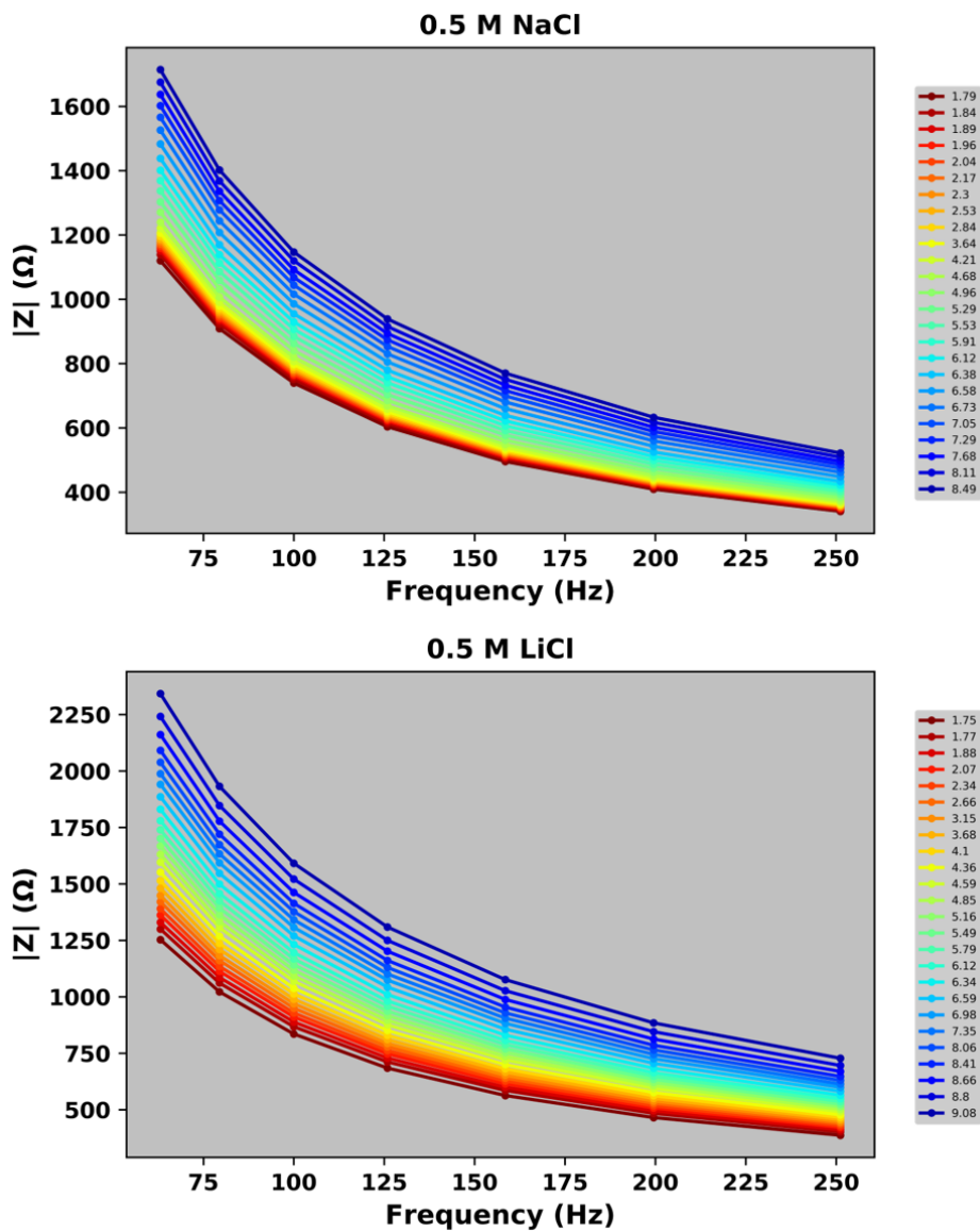
Figure 5.28 Impedance magnitude increasing with pH around 100 Hz for both the 0.5 M NaCl and 0.5 M LiCl solutions. The impedance magnitude change versus pH appears larger in the 0.5 M LiCl solution than in the 0.5 M NaCl solution (© 2022 Elsevier B.V. All rights reserved.). 220
