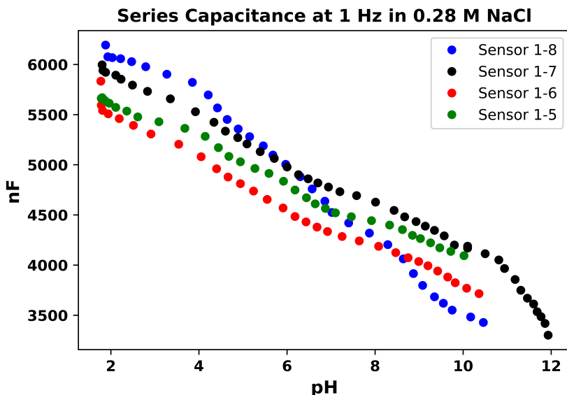
Figure 5.31 The series capacitance plotted at 1 Hz in 0.28 M NaCl.
