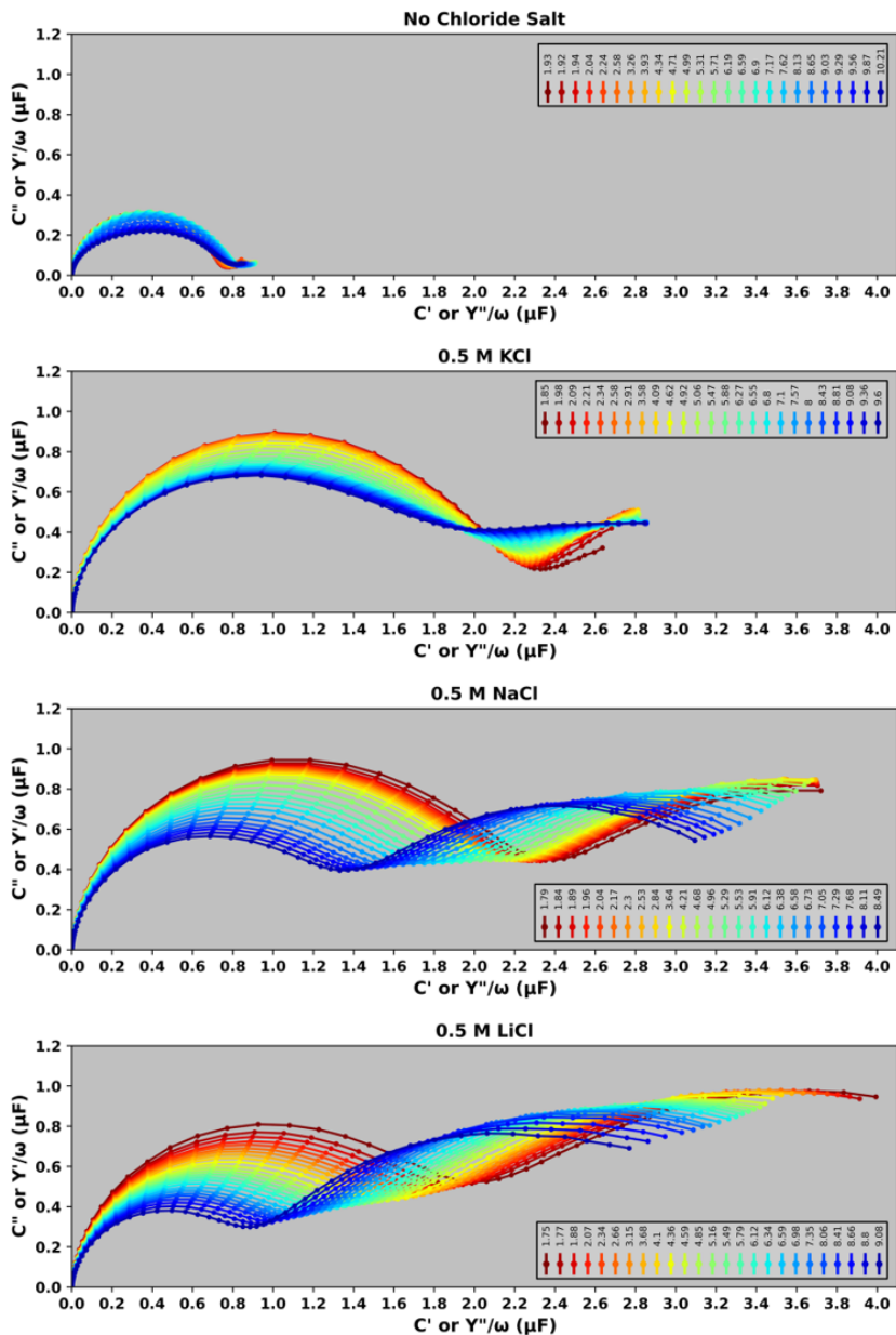
Figure 5.14 Complex capacitance plots with the measured data from 1 Hz to 1 MHz for all solutions, with each pH point color coded from red (acidic) to more basic (blue) (© 2022 Elsevier B.V. All rights reserved.). 220
