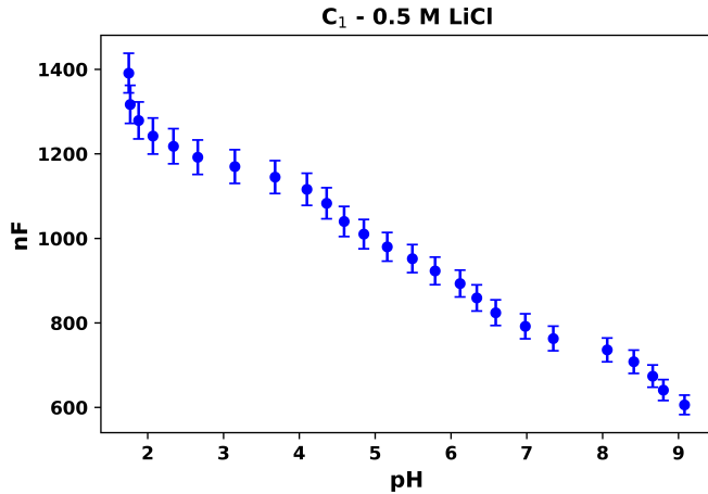
Figure 5.23 C_1 in the simplified, high ionic strength circuit for 0.5 M LiCl, where C_1 appears pH dependent. The C_1 double layer capacitance magnitude for 0.5 M LiCl here appears smaller than for 0.5 M NaCl in Figure 5.22 (the opposite is true for C_2 ) (© 2022 Elsevier B.V. All rights reserved.). 220
