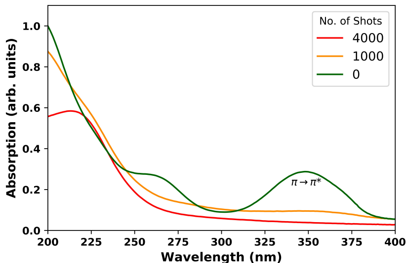
Figure 4.17 UV-Vis absorption spectrum for the benzoylacetone based film and different treatments (© The Royal Society of Chemistry 2020). 136,137
