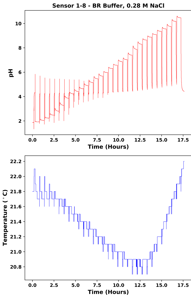
Figure F.1 pH and temperature for sensor 1-8 in 0.28 M NaCl buffer, with “spikes and dips” between the 30 minute pH measurement intervals being when the pH electrode was removed from the measurement solution.
