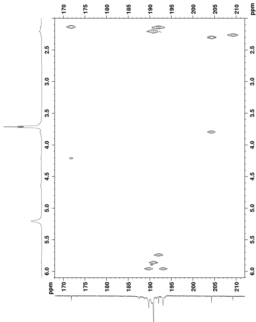
Figure 3.35 HMBC [External D 2 O]: Experiment 4 – Product (© The Royal Society of Chemistry 2020). 136,137
