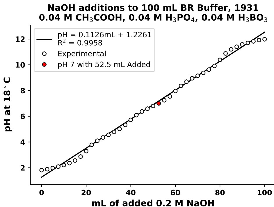
Figure G.1 Original data plotted for 0.2 M NaOH additions to 0.04 M phosphoric acid, 0.04 M acetic acid, and 0.04 M boric acid. 232
