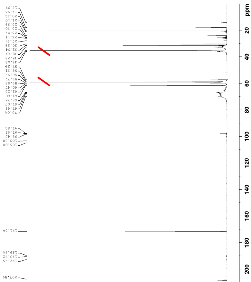
Figure 3.13 ^{13}\text{C} NMR [External \text{D}_2\text{O} ]: Experiment 1 – Product.
