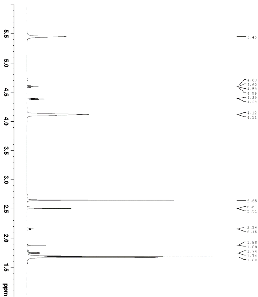
Figure 3.10 ^1\text{H} NMR [External \text{D}_2\text{O} ]: Experiment 1 – Distillate.
