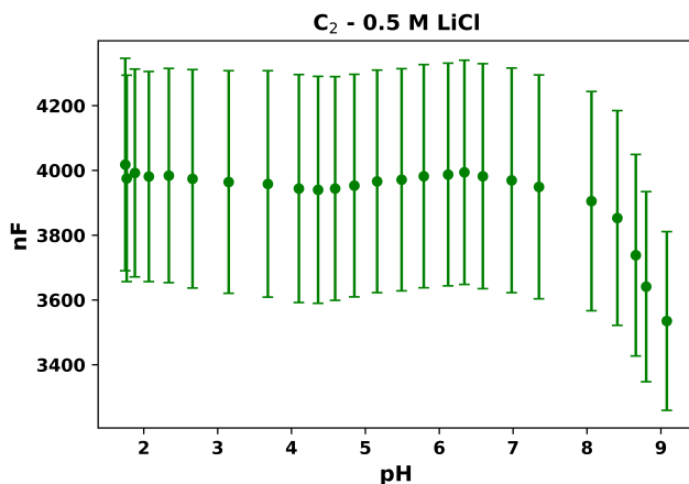
Figure 5.25 C_2 in the simplified, high ionic strength circuit for 0.5 M LiCl, which appears to decrease at high pH (and with increasing NaOH and larger \text{Na}^+ ions). The C_2 specific adsorption capacitance magnitude for 0.5 M LiCl here appears larger than for 0.5 M NaCl in Figure 5.24 (the opposite is true for C_1 ) (© 2022 Elsevier B.V. All rights reserved.). 220
