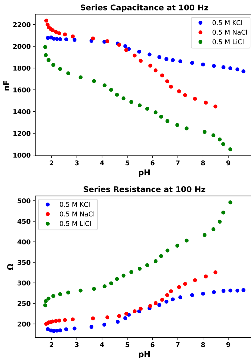
Figure 5.30 Equivalent series resistance (ESR, not to be confused with R_1 ) and series capacitance plotted versus pH at 100 Hz for K^+ (-40 nF/pH), Na^+ (-110 nF/pH), and Li^+ (-110 nF/pH) cations. The Li^+ solution has a higher ESR and a lower series capacitance than the Na^+ solution over the entire pH range (© 2022 Elsevier B.V. All rights reserved.). 220
