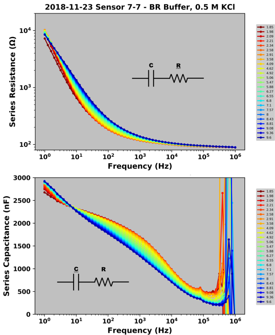
Figure E.10 Series resistance and series capacitance plots for the 0.5 M KCl buffer, with each pH point color coded from red (acidic) to more basic (blue) (© 2022 Elsevier B.V. All rights reserved.). 220
