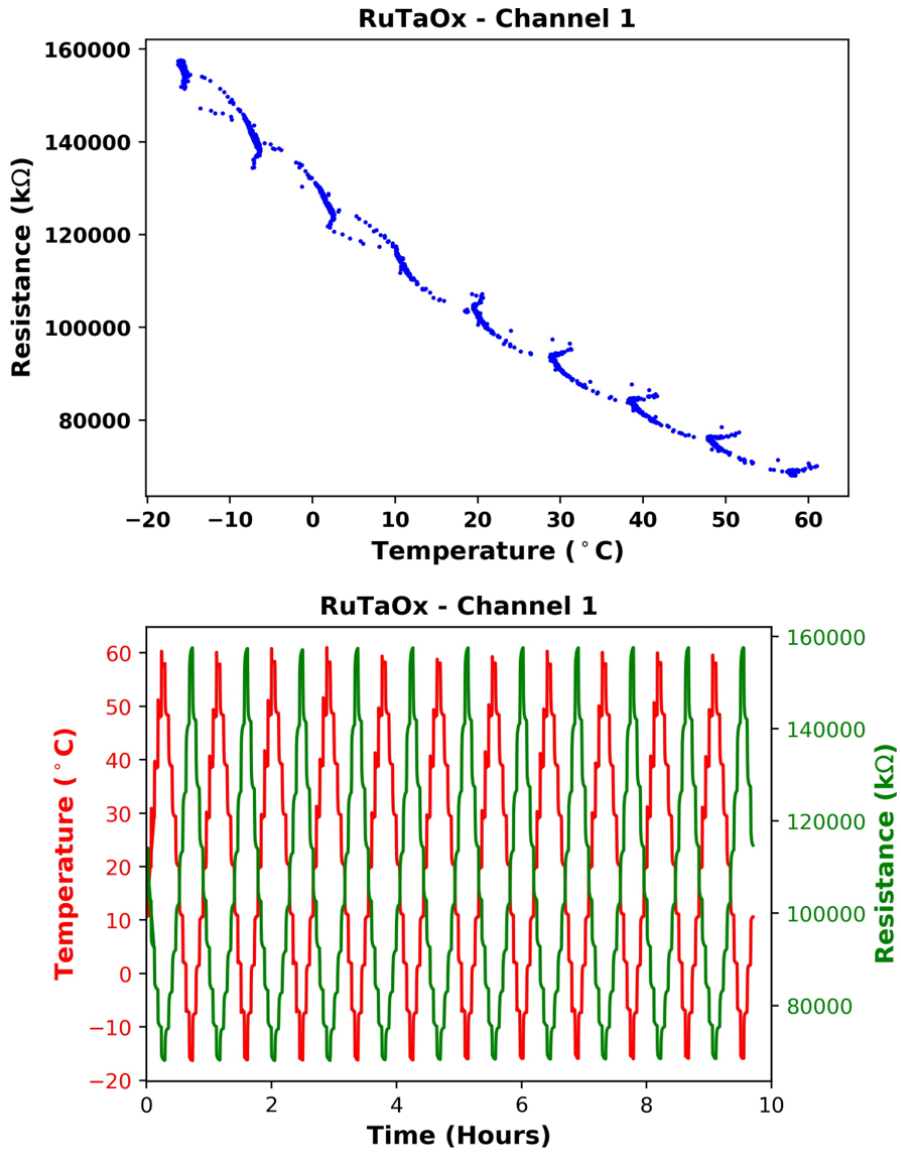
Figure 6.6 Temperature versus resistance for channel 1 and RuTaOx material from Experiment 2.
