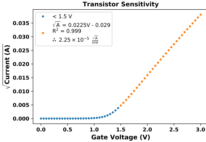
Figure D.3 Transistor V_{GS} swept from 0 V to 3 V, with a V_{DS} bias of 5 V, and plotted versus \sqrt{I_{DS}} , in order to determine the correct conversion for saturation mode where I_{DS} \propto (V_{GS} - V_T)^2 . The linear portion from 1.5 V to 3.0 V is used for the calculation.
