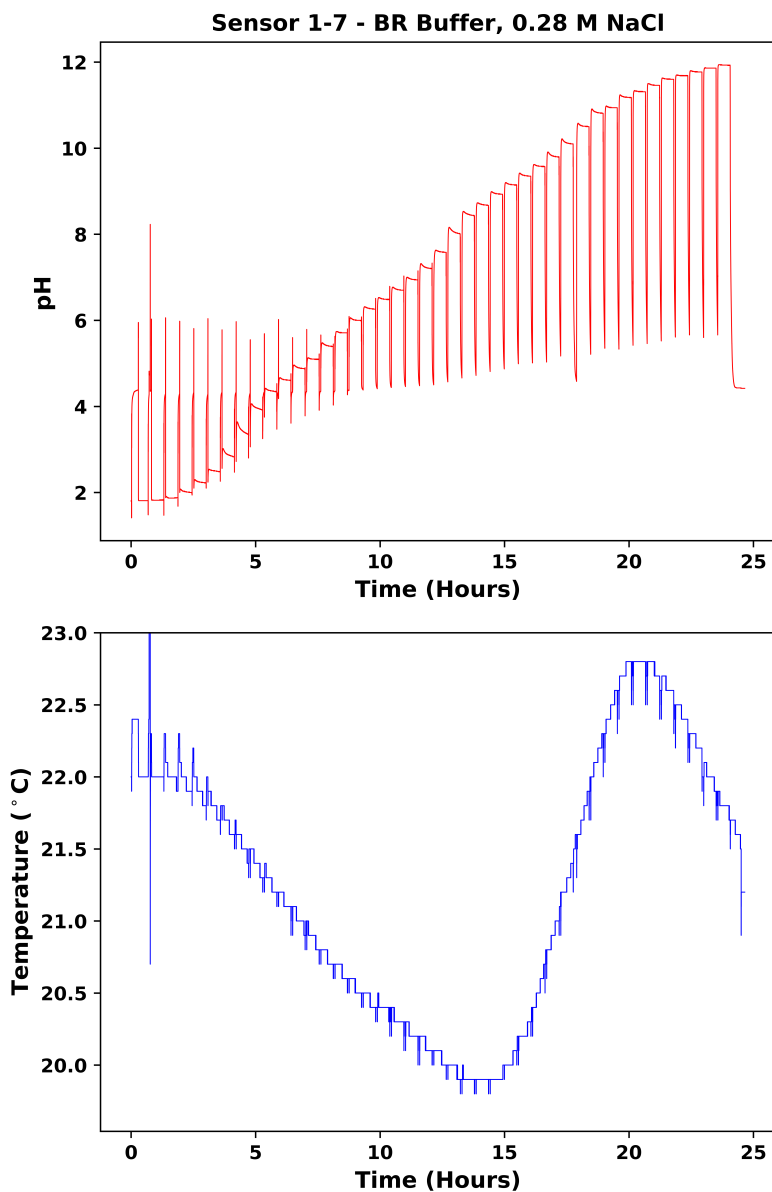
Figure F.3 pH and temperature for sensor 1-7 in 0.28 M NaCl buffer, with “spikes and dips” between the 30 minute pH measurement intervals being when the pH electrode was removed from the measurement solution.
