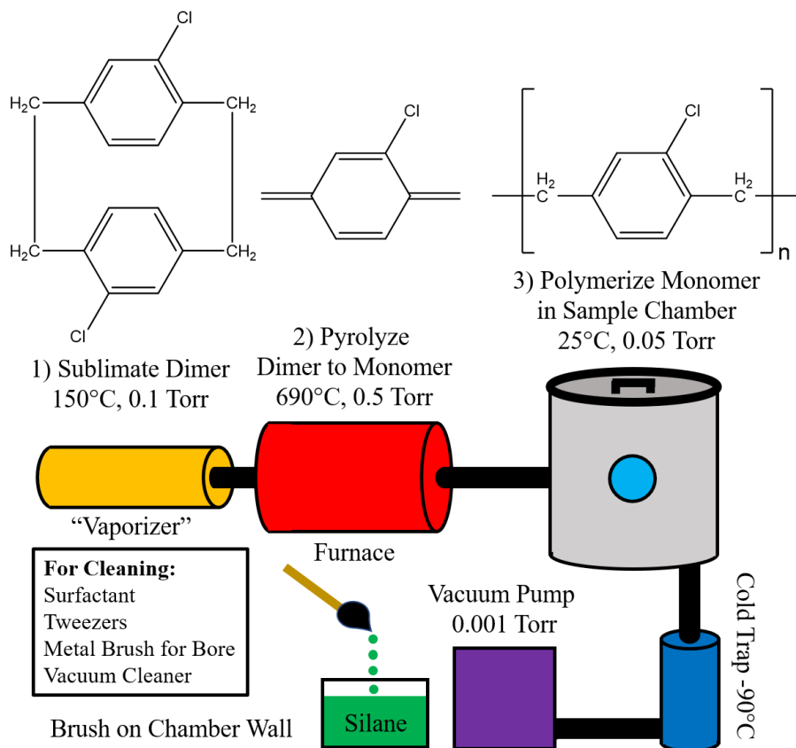
Figure B.2 Parylene deposition as described by the manufacturer 231 for the SCS Labcoter 2 - Parylene Deposition System 2010 (Specialty Coating Systems, Inc. USA) for depositing a parylene C passivation layer with the dichloro-p-cyclophane dimer (DPX-C, Specialty Coating Systems, Inc.), and \gamma -methacryloxypropyl-trimethoxysilane as silane for adhesion (A-174 Silane, Specialty Coating Systems, Inc.). As the pressure decreases upon pumping down, the silane evaporates off the wall and deposits on the sample at \sim 40 Torr. A 2 v/v % Micro-90 surfactant solution (International Products Corporation, USA) in deionized water was used for cleaning the device.
