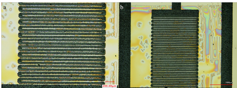
Figure C.2 Sample 2 Firing Parameters ( increase voltage, decrease envelope, divide pulse ) - 1 \times 558 \text{ mJ cm}^{-2} , 450 V, 400 \mu\text{s} , 5 \mu\text{pulses} with 50% duty cycle, no capacitance change (a - before flash lamp, b - after flash lamp).
