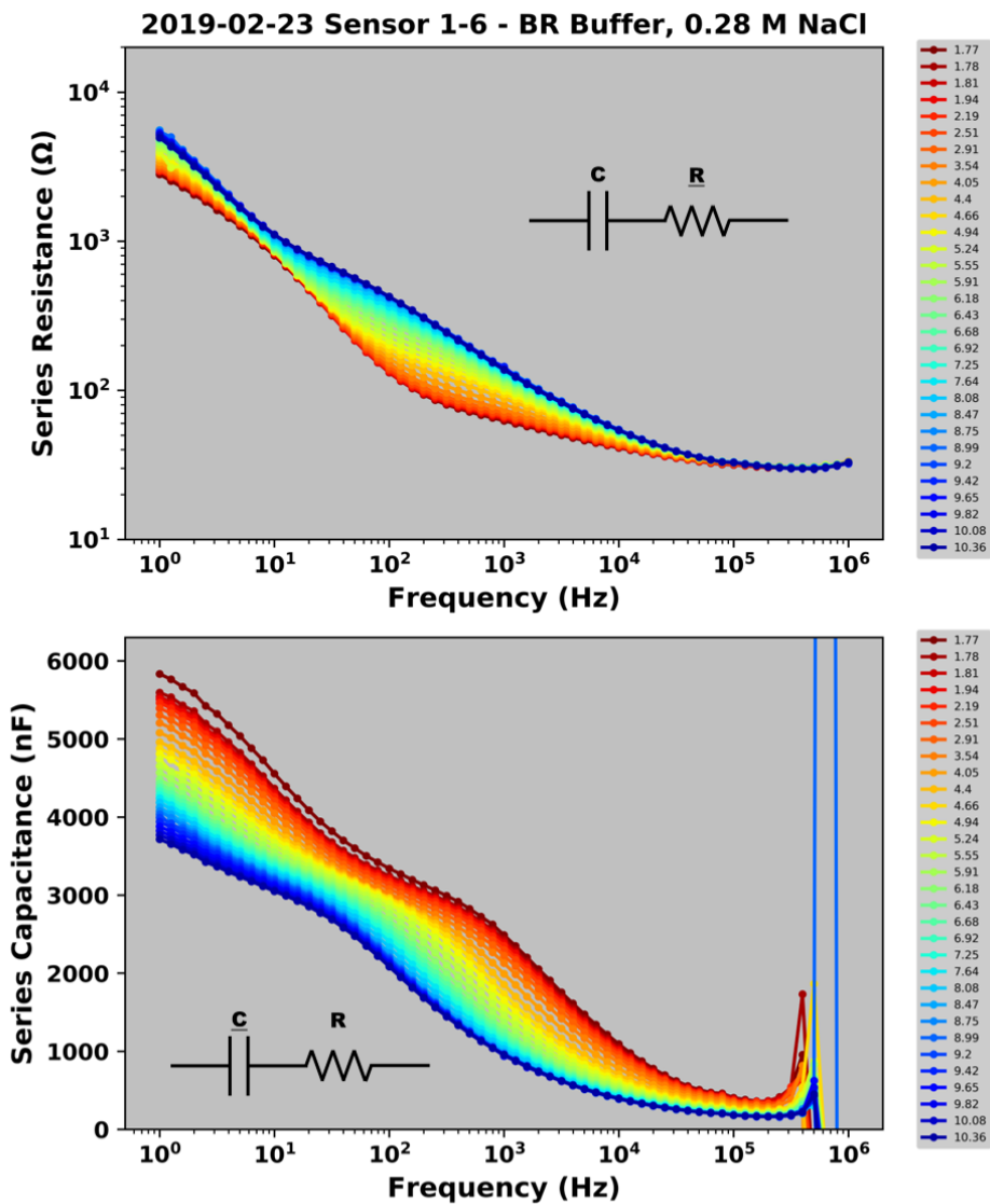
Figure F.6 Series resistance and series capacitance plots for sensor 1-6 in the 0.28 M NaCl buffer, with each pH point color coded from red (acidic) to more basic (blue).
