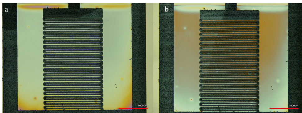
Figure 4.3 Sample 14 Firing Parameters - 2400 \times at 2 Hz, 663 \text{ mJ cm}^{-2} , 450 V, 500 \mu\text{s} , 7 \mu\text{pulses} with 40% duty cycle, [3.5 pF before, 5.0 pF after, 1.2 pF parasitics] (a - before flash lamp, b - after flash lamp). The estimated surface temperature of the substrate, according to the SimPulse 2.5 software, plateaus at the following temperatures (with an operating temperature of 25^\circ\text{C} ): 80 \mu\text{m} thick PET, \sim 30^\circ\text{C} ; 80 \mu\text{m} thick PET with 5 nm Ti adhesion layer and 50 nm Au layer, \sim 390^\circ\text{C} .
