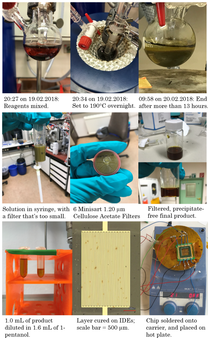
Figure 6.1 Synthesis and fabrication of temperature sensors for Experiment 1.
