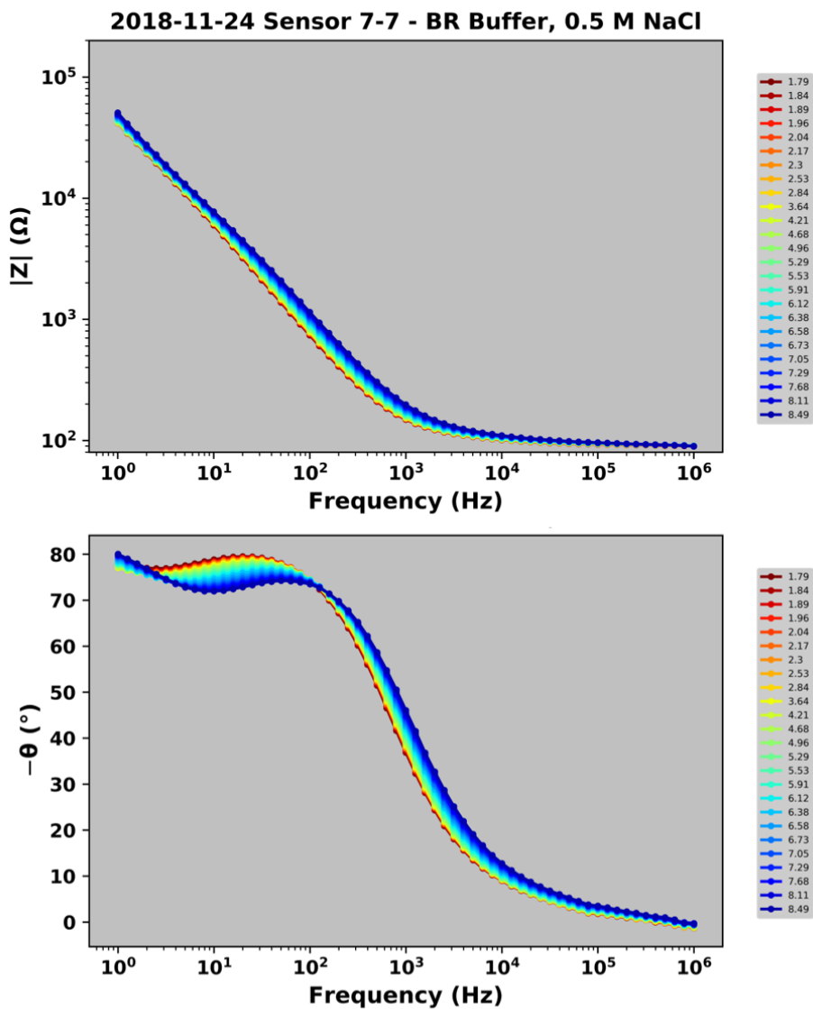
Figure E.3 Bode plot for the 0.5 M NaCl buffer, with each pH point color coded from red (acidic) to more basic (blue) ((© 2022 Elsevier B.V. All rights reserved.). 220
