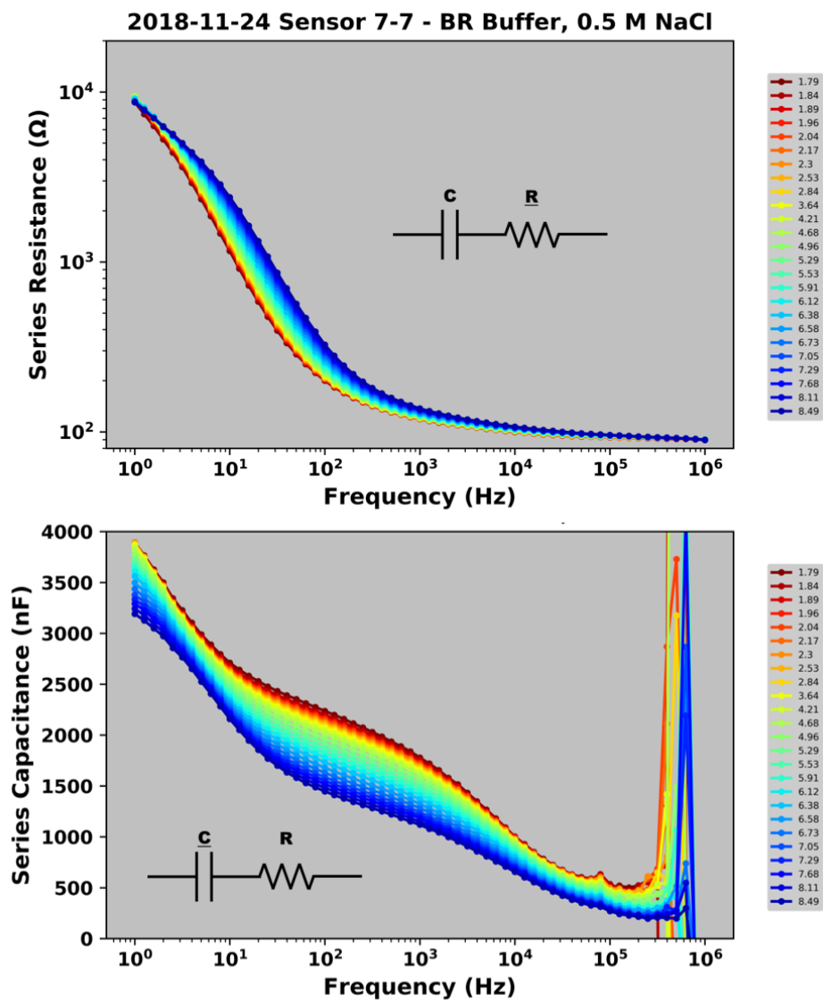
Figure E.11 Series resistance and series capacitance plots for the 0.5 M NaCl buffer, with each pH point color coded from red (acidic) to more basic (blue) ((© 2022 Elsevier B.V. All rights reserved.)). 220
