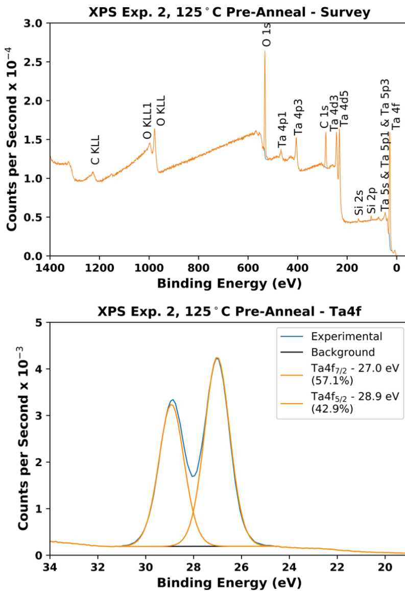
Figure 4.13 XPS after initial thermal anneal at 125°C.
