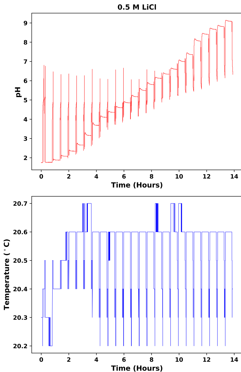
Figure 5.11 pH and temperature for the 0.5 M LiCl buffer, with “spikes and dips” between the 30 minute pH measurement intervals being when the pH electrode was removed from the measurement solution (© 2022 Elsevier B.V. All rights reserved.). 220
