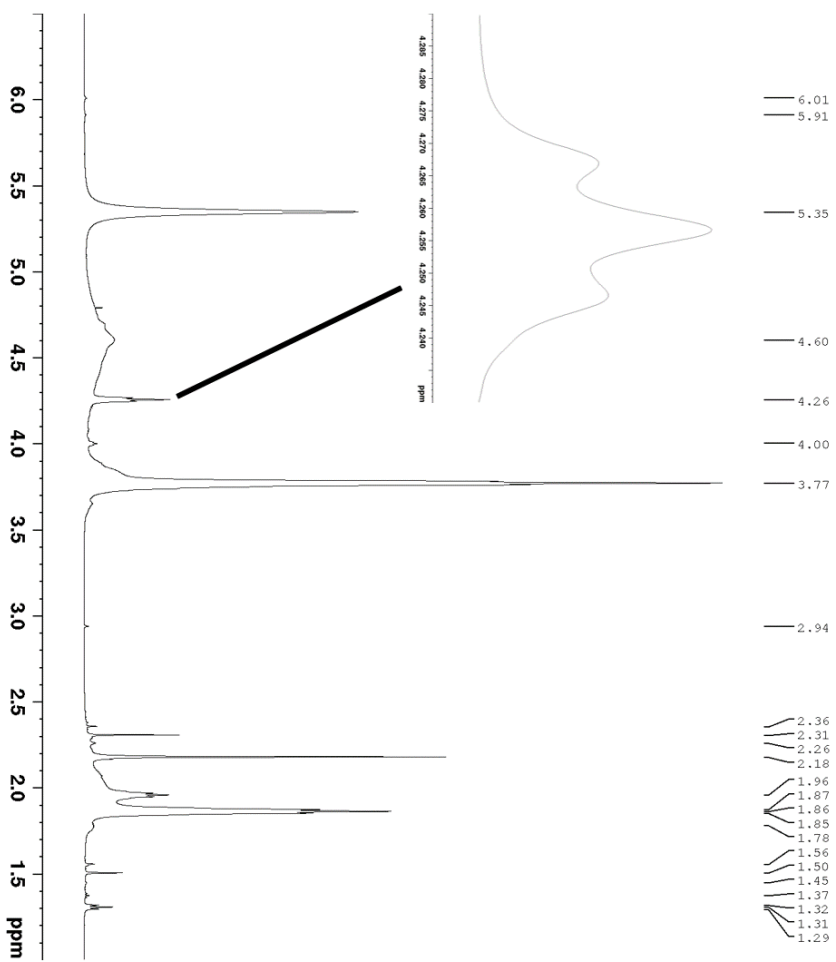
Figure 3.12 ^1\text{H} NMR [External \text{D}_2\text{O} ]: Experiment 1 – Product.
