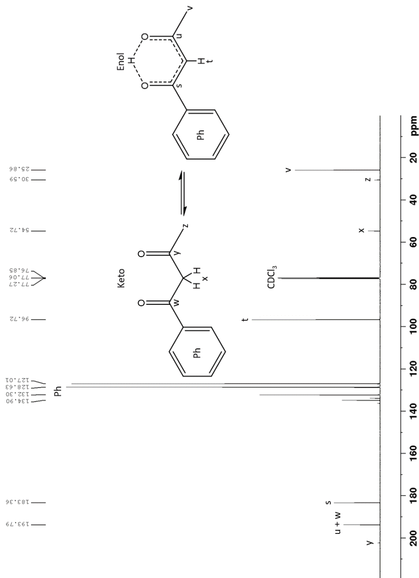
Figure 3.8 ^{13}\text{C} NMR [ \text{CDCl}_3 ]: Benzoylacetone [Sigma Aldrich, 99%] (© The Royal Society of Chemistry 2020). 136,137
