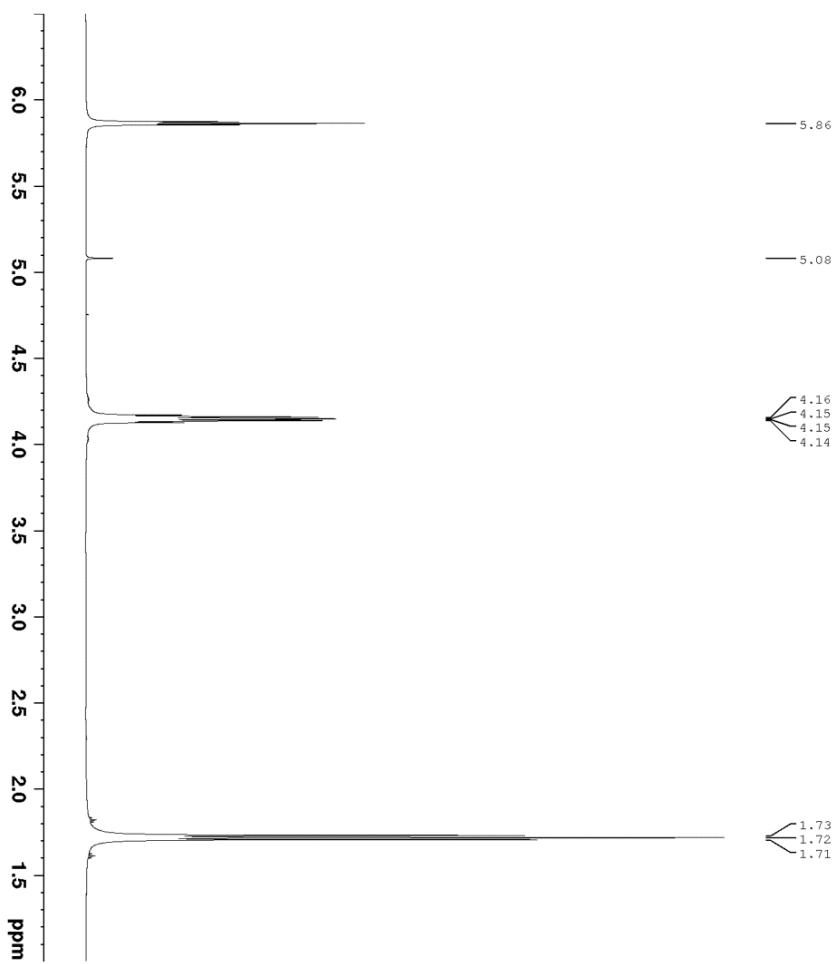
Figure 3.20 ^1\text{H} NMR [External \text{D}_2\text{O} ]: Experiment 3 – Distillate (© The Royal Society of Chemistry 2020). 136,137
