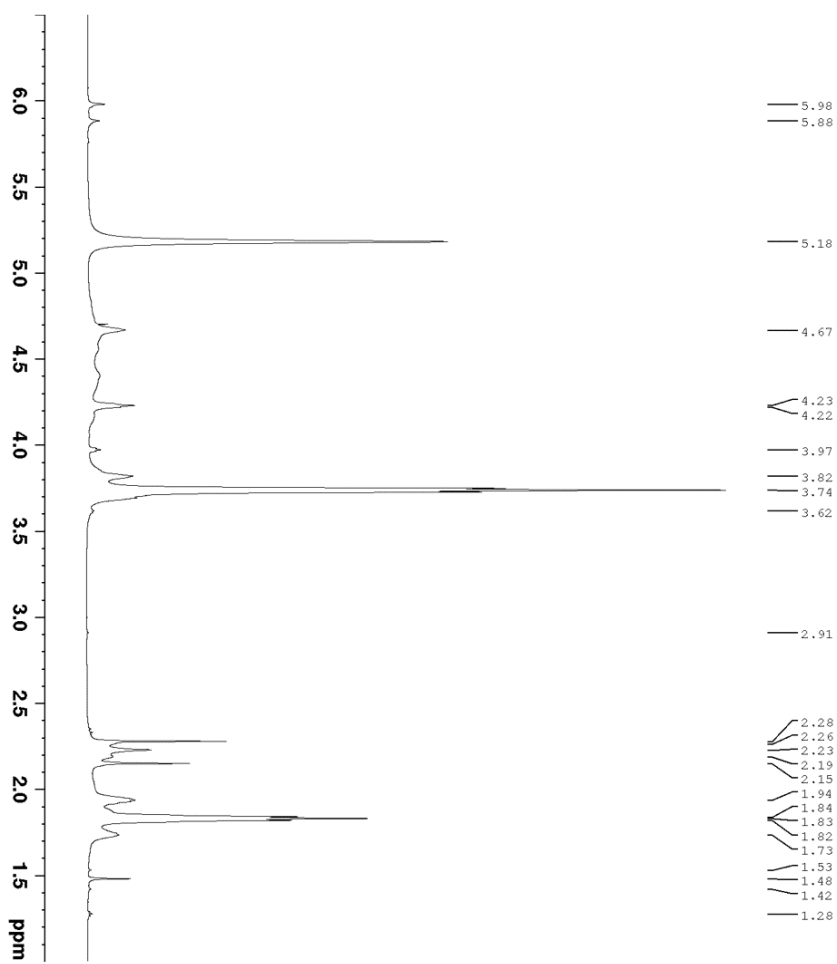
Figure 3.24 ^1\text{H} NMR [External \text{D}_2\text{O} ]: Experiment 3 – Product ((© The Royal Society of Chemistry 2020). 136,137
