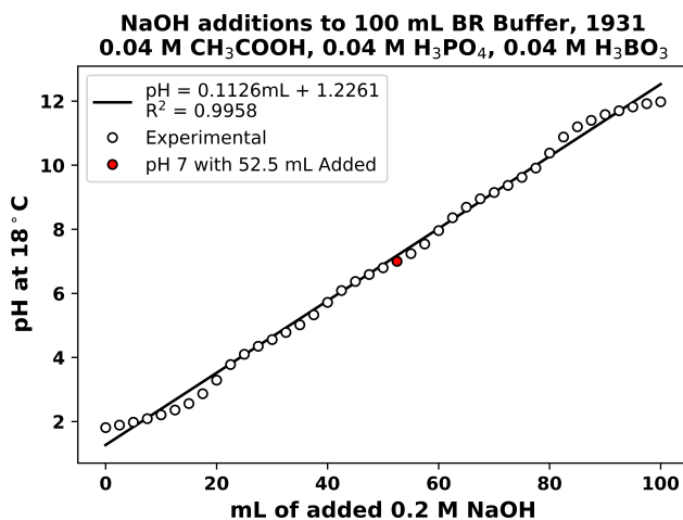
Figure 5.7 Original data plotted for 0.2 M NaOH additions to 0.04 M phosphoric acid, 0.04 M acetic acid, and 0.04 M boric acid. 232
