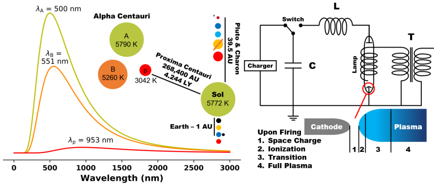
Figure 4.1 Left: spectral output of stars in the Alpha Centauri system, assuming they are black bodies where an increase in surface temperature leads to a blueshift in the peak wavelength - Sol and Alpha Centauri A have a similar spectral output. 223,227 Right: simplified LC circuit with external triggering (via a transformer) and a grounded cathode, with a reference coil wrapped around the lamp to ensure reliable triggering. The optional switch is to protect the charger during discharge. 221
