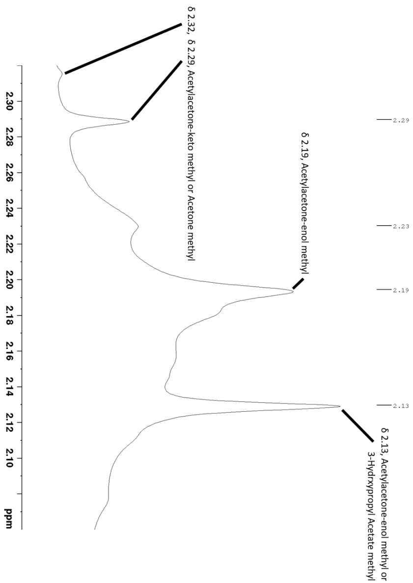
Figure 3.46 ^1\text{H} NMR [External \text{D}_2\text{O} ]: Experiment 12 – Product.
