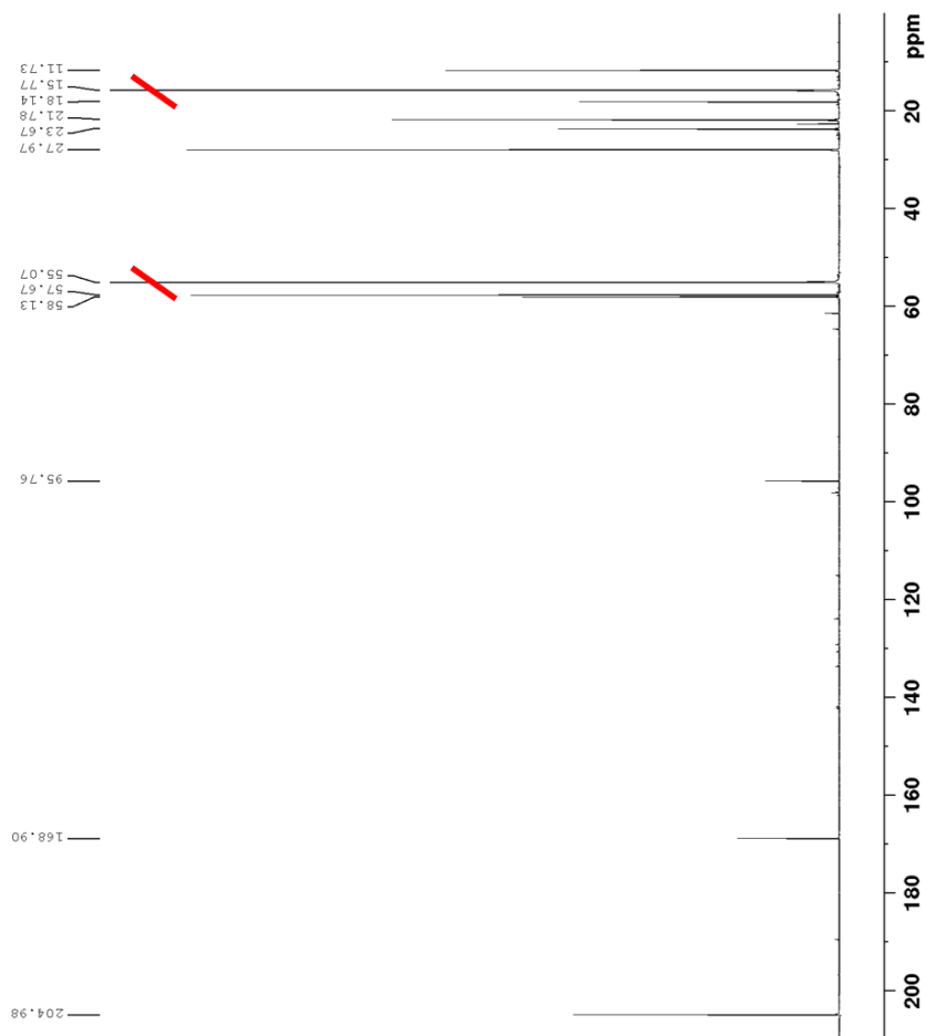
Figure 3.11 ^{13}\text{C} NMR [External \text{D}_2\text{O} ]: Experiment 1 – Distillate.
