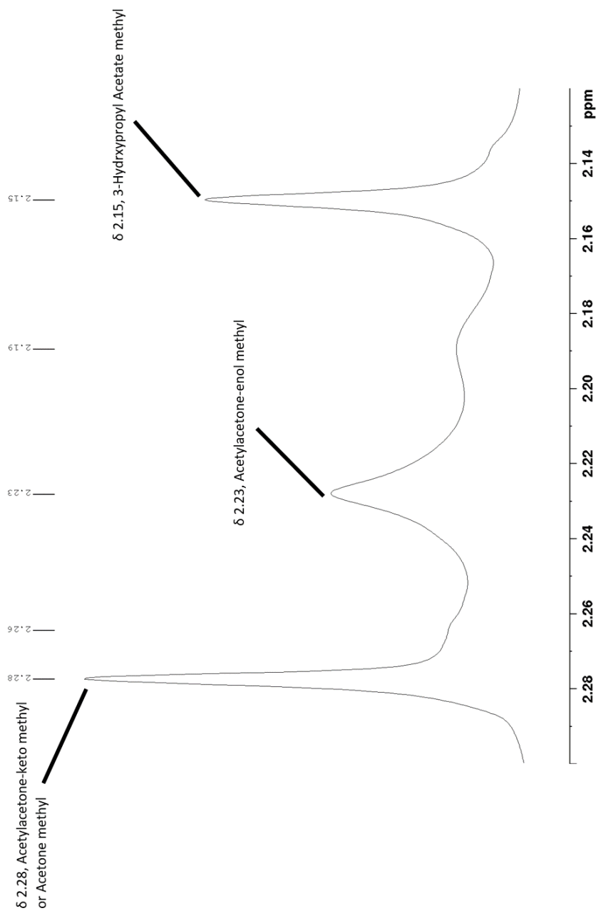
Figure 3.25 ^1\text{H} NMR [External \text{D}_2\text{O} ]: Experiment 3 - Product (© The Royal Society of Chemistry 2020). 136,137
