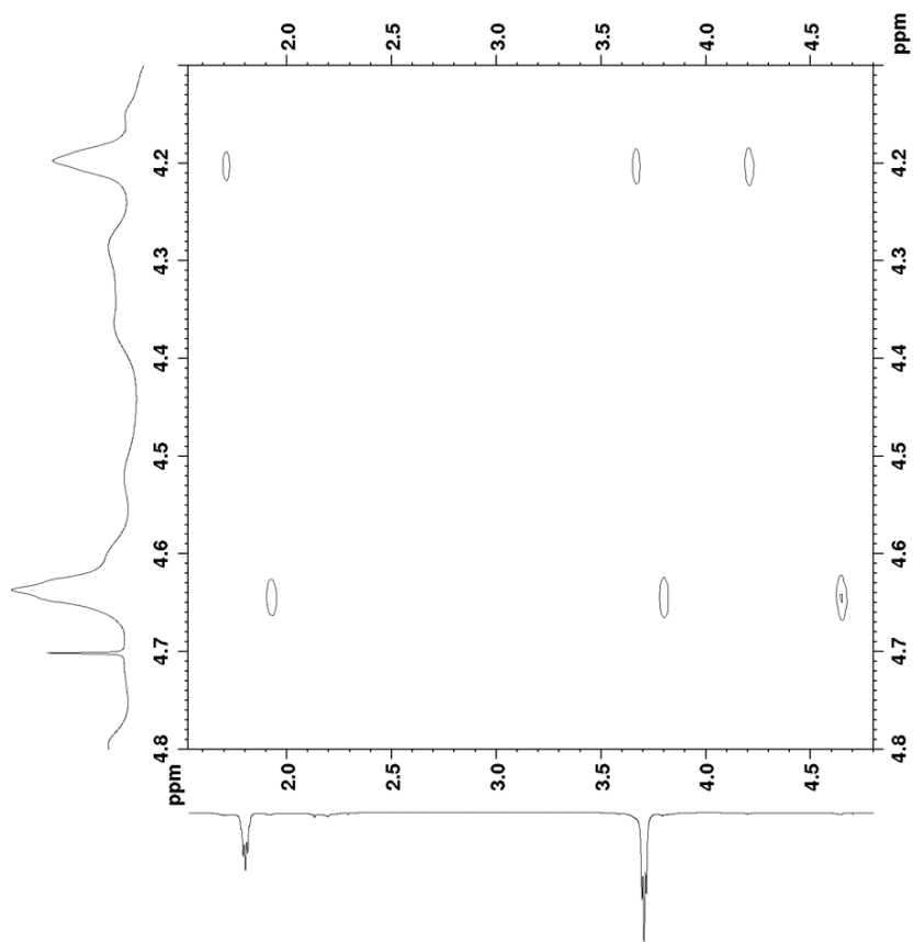
Figure 3.47 TOCSY [External D 2 O]: Experiment 12 – Product.
