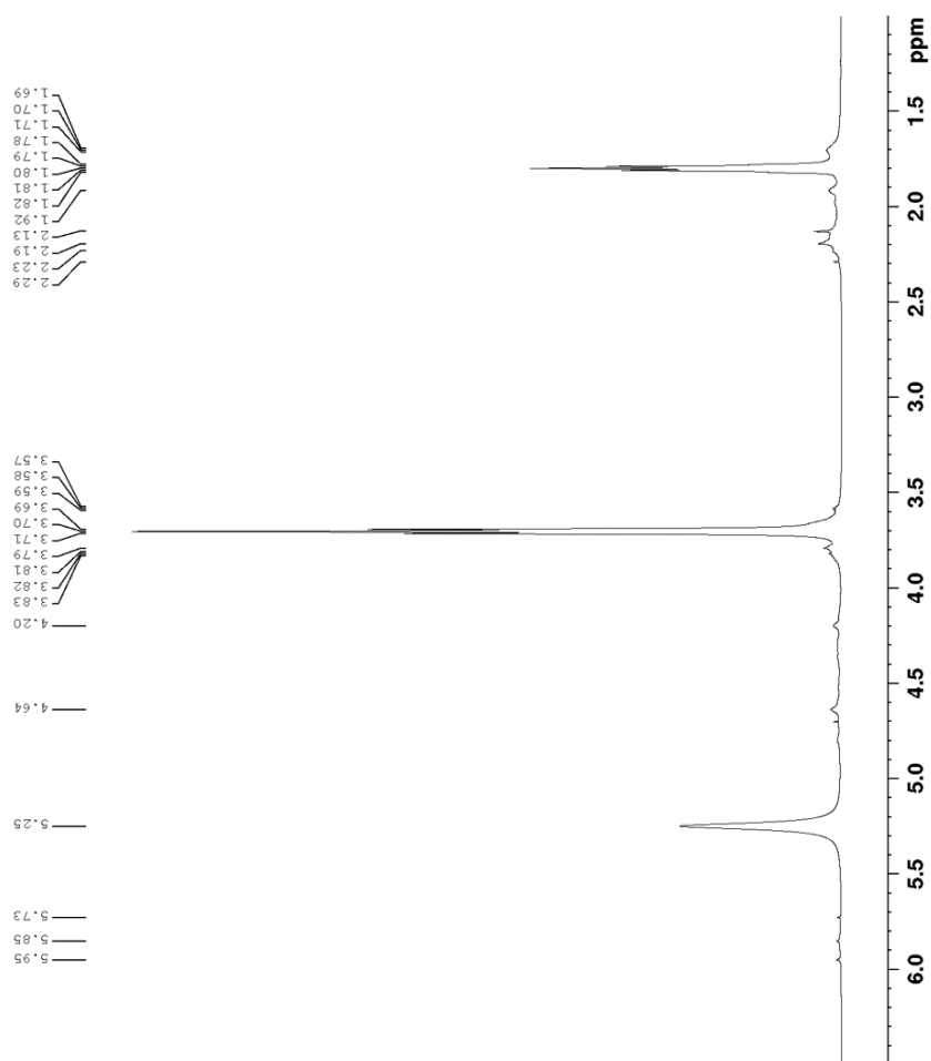
Figure 3.45 ^1\text{H} NMR [External \text{D}_2\text{O} ]: Experiment 12 – Product.
