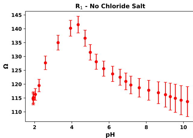
Figure 5.16 C_1 in series with R_1 for “no added alkali chloride salt” solution, where R_1 peaks around pH 4.5.
