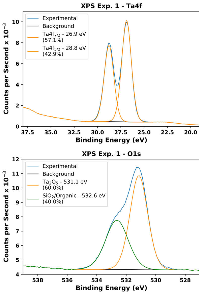
Figure 4.7 XPS Ta 4f and O 1s spectra of Sample 15 (© 2022 Elsevier B.V. All rights reserved.). 220
