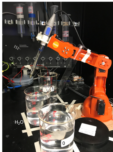
Figure 5.6 Diagram of the arm holding the pH electrode perpendicular to Earth in solution (upper left), along with the arm position for removing the electrode (upper right) and the beaker positions (lower left). The image of the automated setup in the Faraday cage (lower right) shows the arm moving the pH electrode from beaker to beaker (© 2022 Elsevier B.V. All rights reserved.). 220
