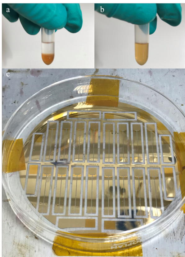
Figure 4.8 Ink before vortexing with phase separation, with DEGEE above as clear and the product below as amber (a), ink after vortexing (b), and ink printed on gold PET foil (c) annealing on the hot plate, with the darker areas being the printed layer.
