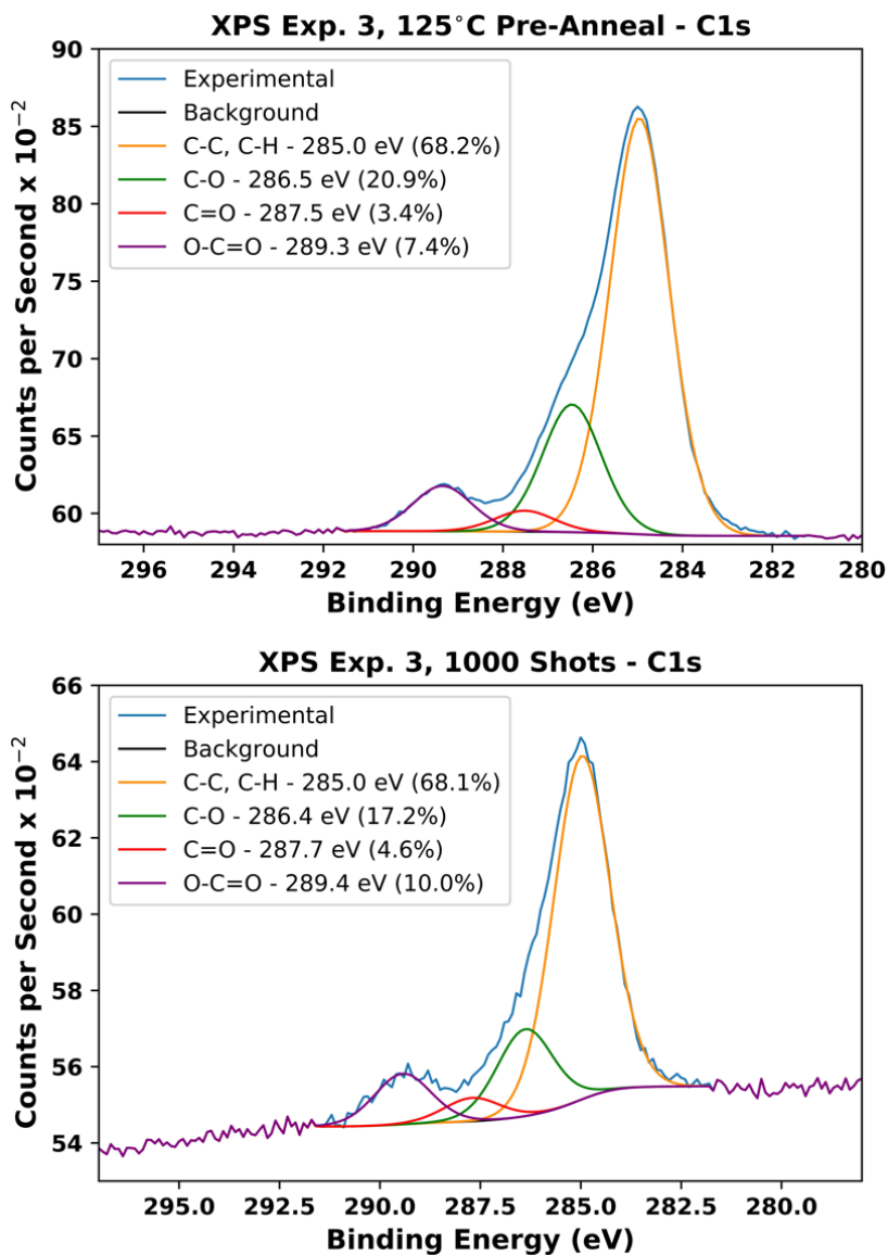
Figure 4.28 XPS C 1s spectra of “125°C pre-anneal” and “1000 shots with pre-anneal” samples (© The Royal Society of Chemistry 2020). 136,137
