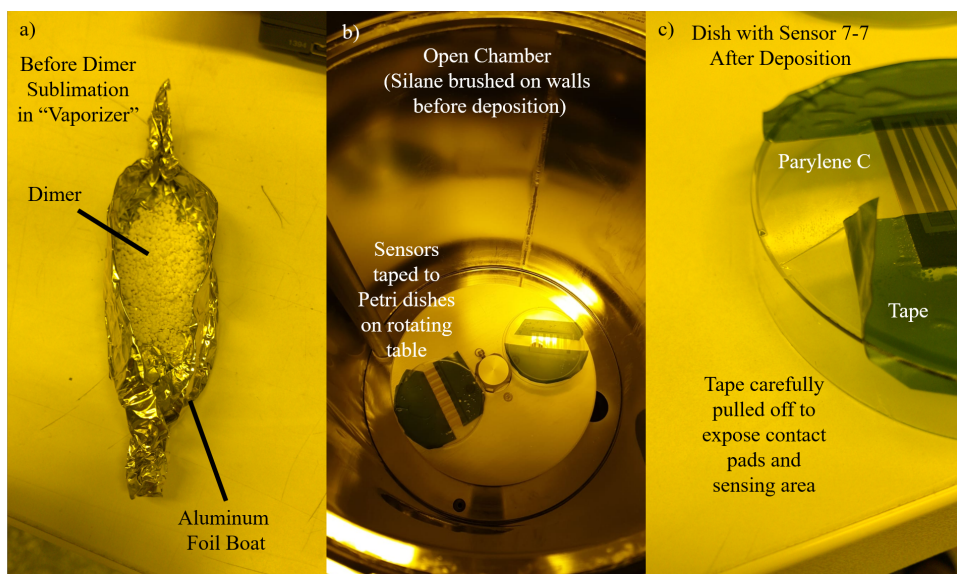
Figure B.1 Dimer in the boat before being placed in the “vaporizer” (as named in industry 231 where “vaporization” occurs, but technically incorrect as the dimer sublimates) (a), open chamber where sensors on Petri dishes are set on the rotating table at the bottom of the chamber, with a few brush strokes of silane on the wall before starting the deposition process (b), and careful peeling off of the clean room dicing tape (1008R-11.5, Ultron Systems, Inc.) to expose the sensor and contact pads while leaving the feed lines passivated (c).
