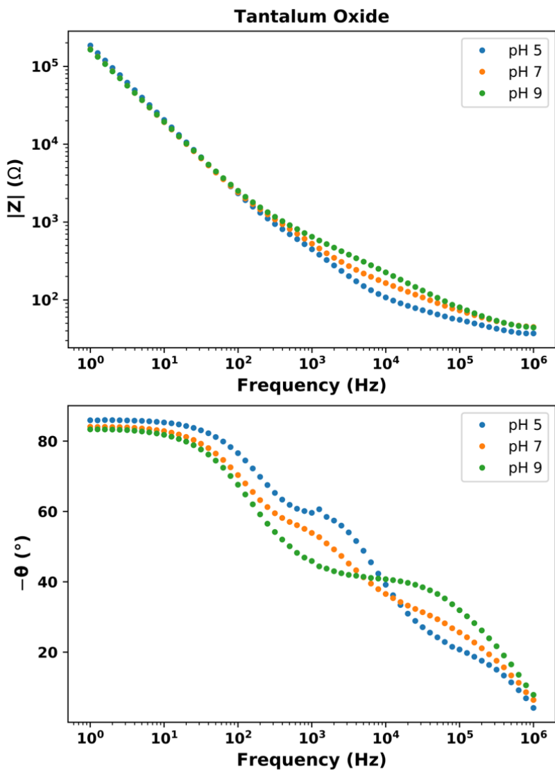
Figure 4.5 Average spectra ( n = 5 ) for pH buffer solution dropped on tantalum oxide covered electrodes for Sample 14.
