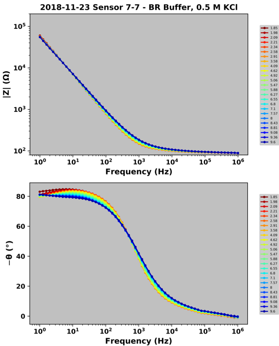
Figure E.2 Bode plot for the 0.5 M KCl buffer, with each pH point color coded from red (acidic) to more basic (blue) (© 2022 Elsevier B.V. All rights reserved.). 220
