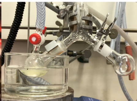
09:46 on 25.02.2019: Start under argon, finger towards reactor (left).
