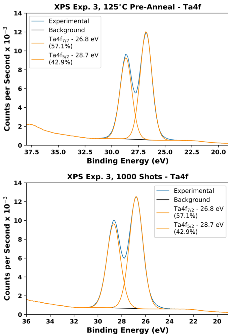
Figure 4.24 XPS Ta 4f spectra of “125°C pre-anneal” and “1000 shots with pre-anneal” samples (© The Royal Society of Chemistry 2020). 136,137
