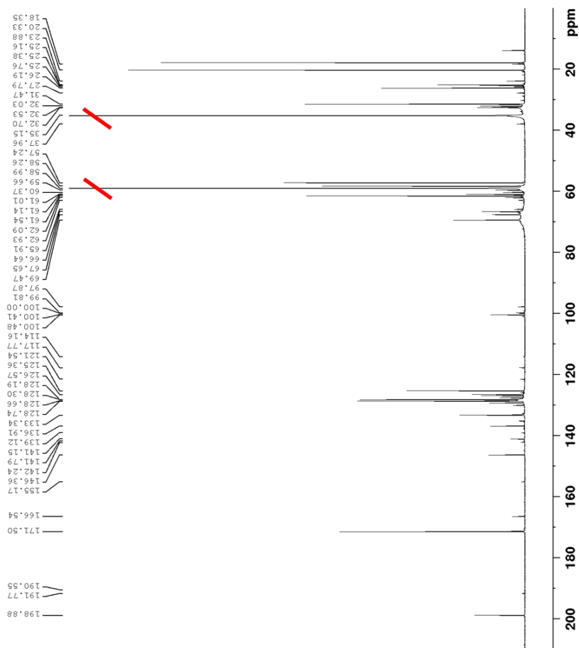
Figure 3.17 ^{13}\text{C} NMR [External \text{D}_2\text{O} ]: Experiment 2 – Product.
