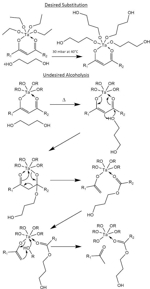
Figure 3.42 Desired substitution (above) and the undesired mechanism of alcoholysis (below), the latter of which results in the formation of acetone and 3-hydroxypropyl acetate through the alcoholysis of acetylacetone. R_1 and R_2 are both methyl groups for acetylacetone, and would change for other \beta -diketones/ \beta -ketoesters (© The Royal Society of Chemistry 2020). 136,137
