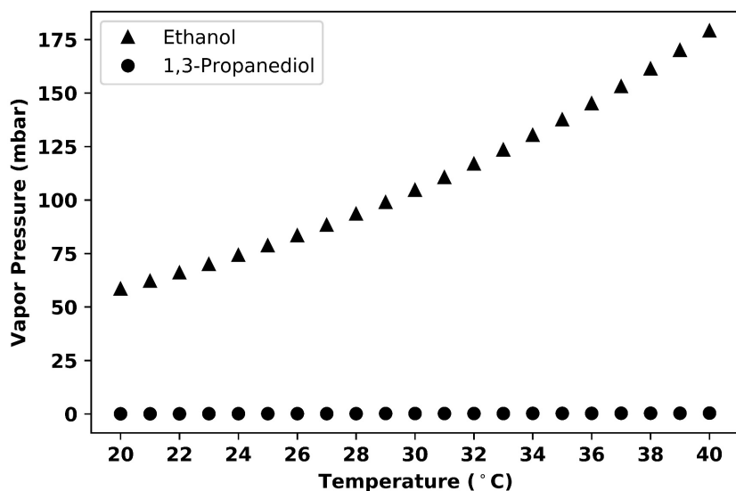
Figure 3.29 Temperature vs. vapor pressure as per the National Institute of Standards and Technology, U.S. Department of Commerce (© The Royal Society of Chemistry 2020).
