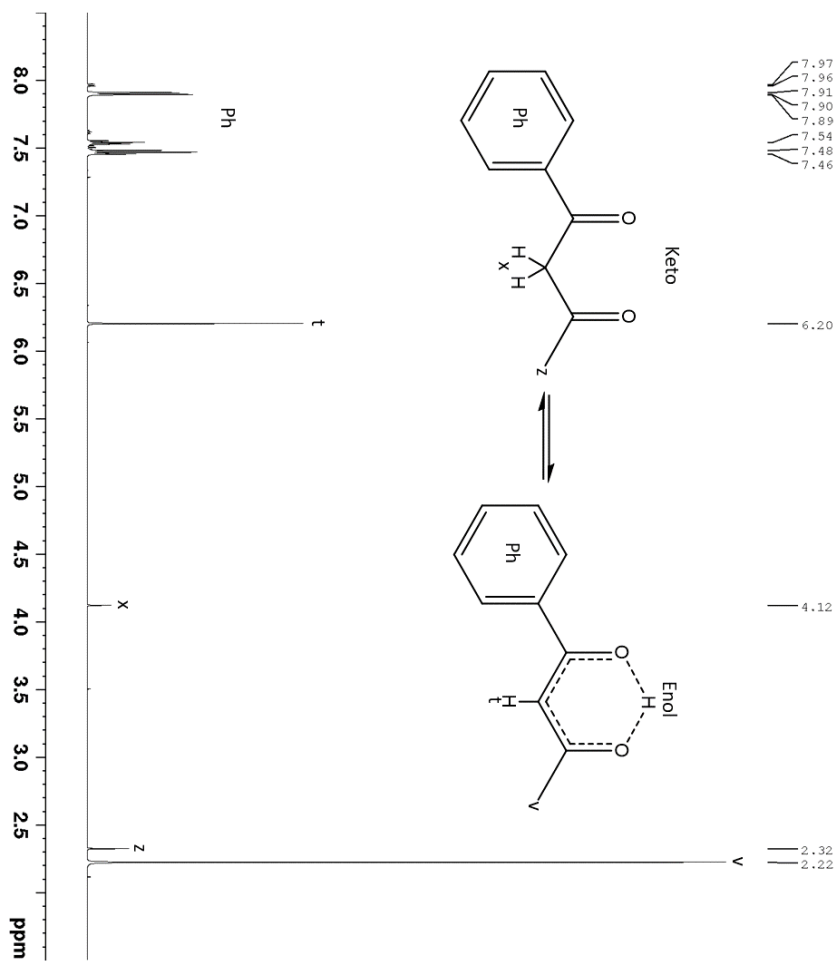
Figure 3.7 ^1\text{H} NMR [ \text{CDCl}_3 ]: Benzoylacetone [Sigma Aldrich, 99%] (© The Royal Society of Chemistry 2020). 136,137
