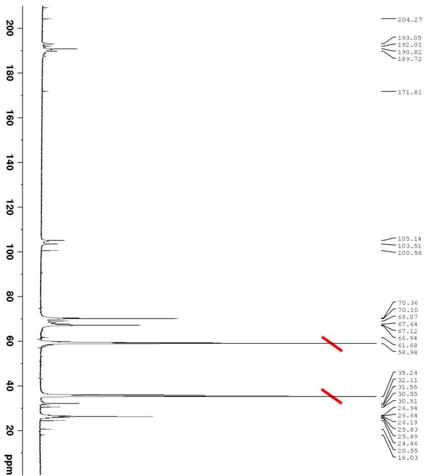
Figure 3.34 ^{13}\text{C} NMR [ \text{External D}_2\text{O} ]: Experiment 4 – Product (© The Royal Society of Chemistry 2020). 136,137
