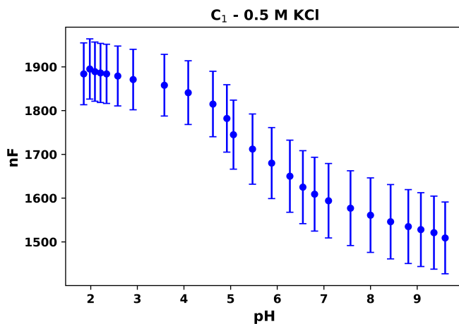
Figure 5.21 C 1 in series with R 1 from 100 Hz to 1 MHz for 0.5 M KCl, where C 1 appears pH dependent but with significant error.
