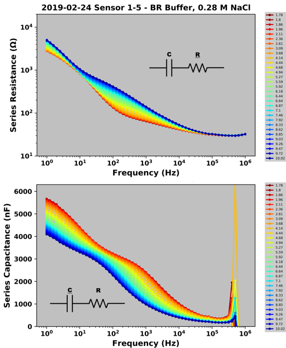
Figure F.8 Series resistance and series capacitance plots for sensor 1-5 in the 0.28 M NaCl buffer, with each pH point color coded from red (acidic) to more basic (blue).
