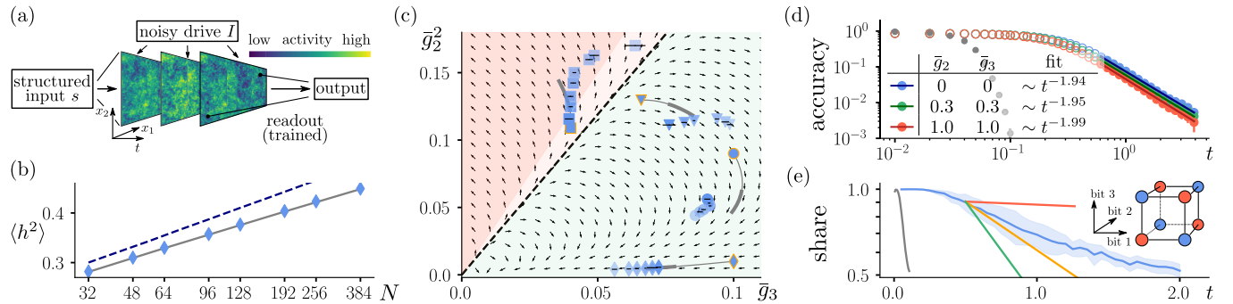
FIG. 1. (a) Model schematics. (b) Variance. Variance as a function of N for \bar{g}_3 = 0.1 and \bar{g}_2^2 = 0.01 ( \bar{g}_2^2 \ll \bar{g}_3 regime); blue diamonds: simulation; dashed dark blue line: linear system; gray solid line: renormalized theory. (c) Flow of couplings. Direction of flow (arrows) theoretically predicted by Eqs. (5) and (6). The transition line (black, dashed) separates the converging region (green) from the diverging region (red). Region of nonphysical bistable regime in darker red. Simulated flow of couplings at \ell = (N/2) , with N \in \{32, 48, 64, 96, 128, 192\} (dark to light shading of blue markers; squares include N = 256, 384 ) for different initial conditions (yellow edge). Predicted flow by Eqs. (5) and (6) (gray solid curves, thicker within the range of simulated \ell ). (d) Memory. Reconstruction accuracy (0: complete forgetting; 1: perfect reconstruction) over time of a Gaussian input for different strengths of the nonlinearities (legend). (e) Classification. Share of correctly assigned parity to 3-bit strings (blue curve) and standard deviation across repeated trainings (shaded area), for \bar{g}_2 = \bar{g}_3 = 0.3 . Decay timescales of the slowest (red), middle (orange), and fastest (green) modes available at readout. Inset: spatial visualization of all 3-bit strings, colored by their parity. In (d) and (e): Gray dots or curve show performance away from criticality with a nonvanishing mass m_1 , corresponding to a correlation length of a single lattice spacing.
