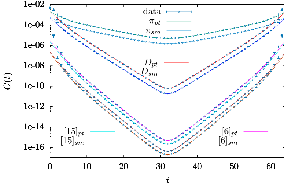
Figure 4: Eight hadron correlators used for simultaneous 2-state fits with t_{\min} = 5 (see text). From top to bottom, the correlators represent: \pi_{pt} , \pi_{sm} , D_{pt} , D_{sm} , [6]_{pt} , [15]_{pt} , [6]_{sm} , and [15]_{sm} , with the subscripts “pt” and “sm” referring to point and smeared sink operators. Lattice data error bars are too small to be seen.
