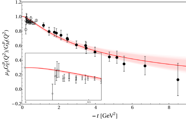
FIG. 2. Complete fit to space- and timelike data with bootstrap error (shaded band) compared to JLab data for \mu_p G_E^p / G_M^p at spacelike momentum transfer. Fitted data are depicted by closed symbols. The data for |t| < 1 \text{ GeV}^2 (open symbols, see also the inset) are shown for comparison only. For references to the data, see Supplemental Material [15].
