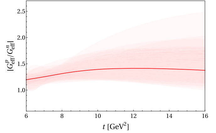
FIG. 3. Form factor ratio |G_{\text{eff}}^p(t)/G_{\text{eff}}^n(t)| in the timelike region for the best fit, with the bootstrap uncertainties indicated by the shaded band.
