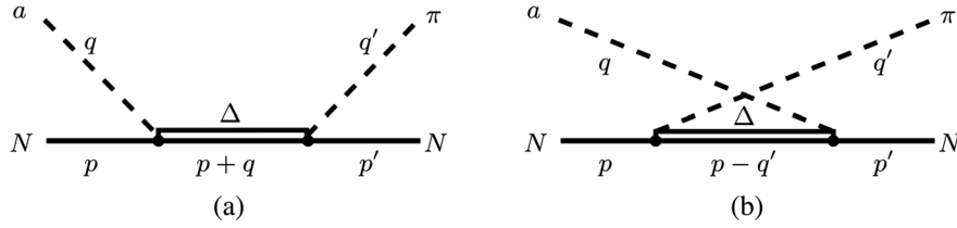
FIG. 2. Tree-level contributions to aN \rightarrow \pi N with an intermediate \Delta state. (a) s channel and (b) crossed channel.
