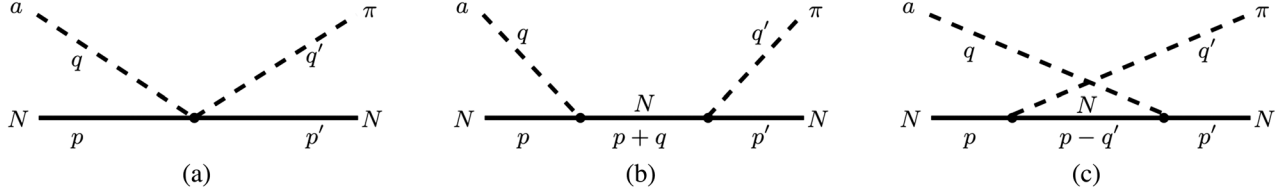
FIG. 1. Tree-level contributions to aN \rightarrow \pi N without the \Delta intermediate state. (a) contact interaction, (b) s channel, and (c) crossed channel.
