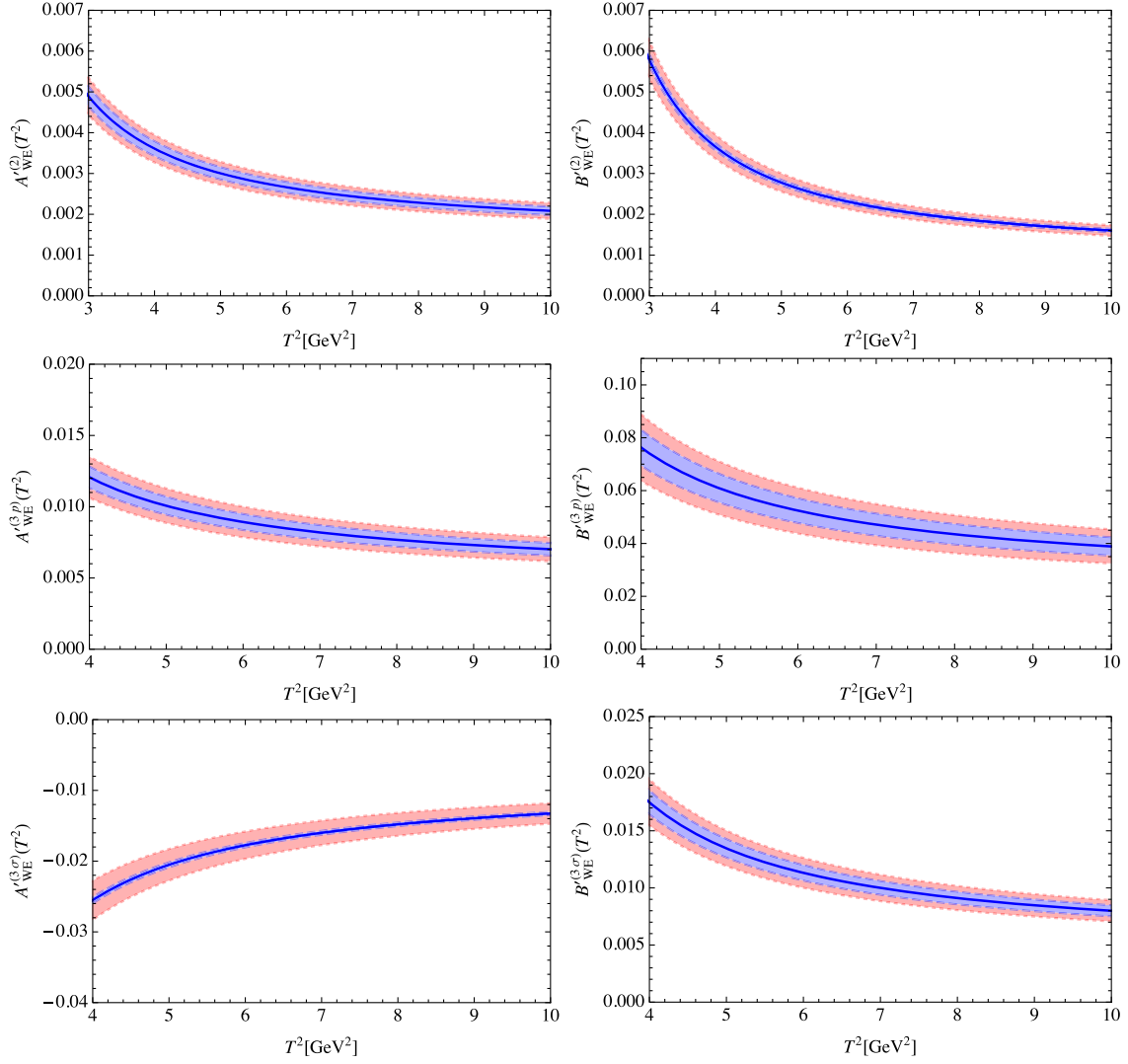
FIG. 4. The Borel parameter dependence of the \Xi_{cc}^{++} \rightarrow \Xi_c^{+'} \pi^+ decay amplitudes A'^{(2)}(B'^{(2)}) , A'^{(3p)}(B'^{(3p)}) , and A'^{(3\sigma)}(B'^{(3\sigma)}) from the twist-2, twist-3p, and twist-3 \sigma LCDAs, respectively. In each diagram, the blue band denotes the uncertainty from the error of the threshold: s_{\Xi_{cc}} = (4.1 \pm 0.1)^2 \text{ GeV}^2 and s_{\Xi_c} = (3.3 \pm 0.1)^2 \text{ GeV}^2 . The upper and lower red bands denote the uncertainty from the error of Monte Carlo integrations.
