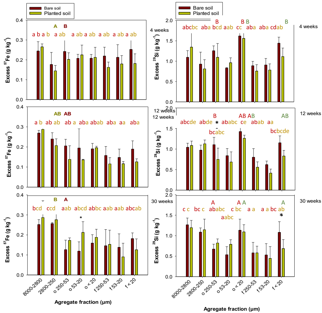
Fig. 5. Excess ^{57}\text{Fe} -goethite (left) and ^{29}\text{Si} -montmorillonite (right) in different soil aggregate fractions 4, 12, and 30 weeks after experiment start. Different lowercase letters indicate significant differences between fractions within a given treatment and sampling date. Different capital letters indicate significant differences between sampling dates within a given treatment and size fraction. An asterisk indicates a significant difference between treatments ( Festuca planted vs bare soil) within a given fraction and sampling date. Lacking letters point to lacking statistical differences in all instances.
