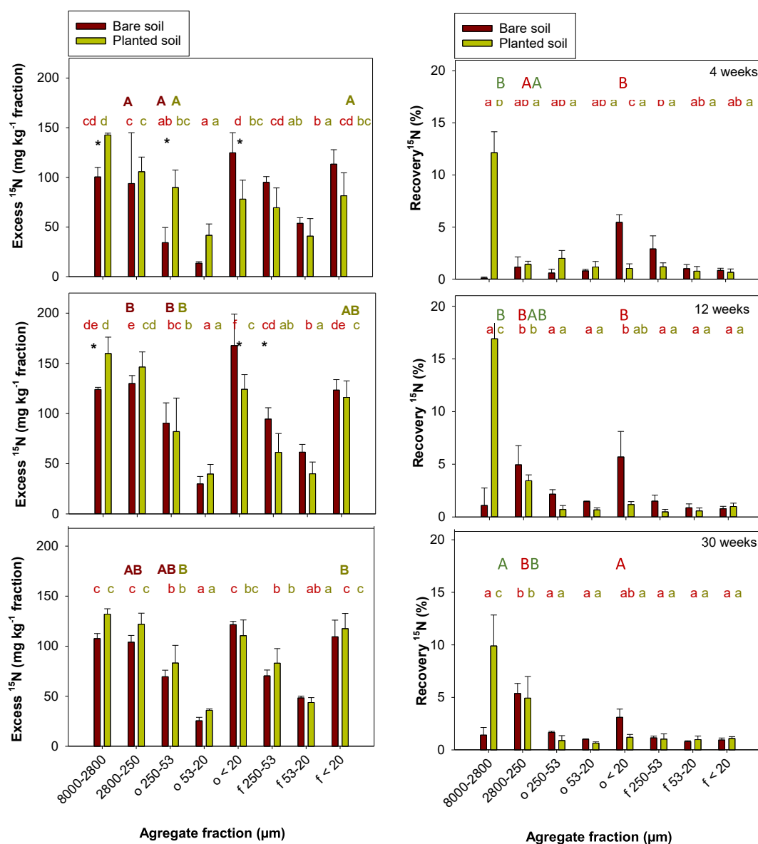
Fig. 3. Excess bacteria-derived 15 N (left) and its recovery relative to the added amount (right) in different soil aggregate fractions 4, 12, and 30 weeks after experiment start. Different lowercase letters indicate significant differences between fractions within a given treatment and sampling time. Different capital letters indicate significant differences between sampling dates within a given treatment and size fraction. An asterisk indicates a significant difference between treatments ( Festuca planted vs bare soil) within a given fraction and sampling date. Comparisons where no letters or asterisks are indicated did not show a significant difference ( p > 0.05 ).
