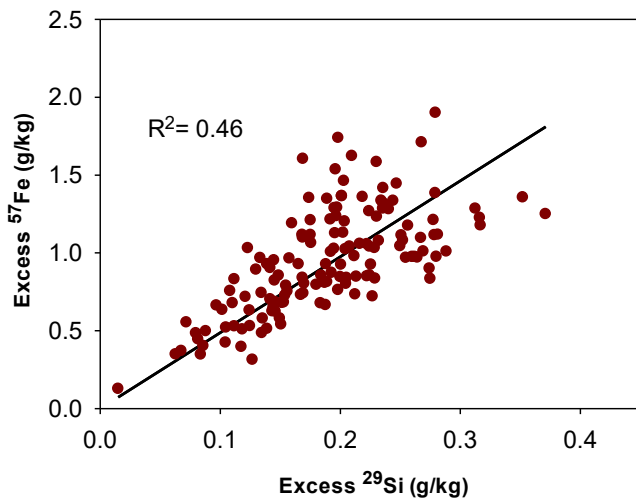
Fig. 6. Correlation between ^{57}\text{Fe} -labelled goethite and ^{29}\text{Si} -labelled montmorillonite in different soil aggregate fractions and across different sampling times (4, 12, 30 weeks).
