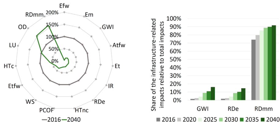
FIGURE 6 | Environmental impacts of the production processes in case study 3 for year 2040, relative to the base year 2016 (left). Share of infrastructure-related impacts on the total impacts for selected impact categories (right). Shown impact categories: freshwater eutrophication (Efw), marine eutrophication (Em), global warming impact (GWI), freshwater and terrestrial acidification (Atfw), terrestrial eutrophication (Et), ionizing radiation (IR), resource depletion, energy (RDe), human toxicity, non-carcinogenic (HTnc), photochemical ozone formation (PCOF), water scarcity (WS), freshwater ecotoxicity (Etfw), human toxicity, carcinogenic (HTc), land use (LU), ozone depletion (OD), resource depletion, mineral and metal (RDmm).
