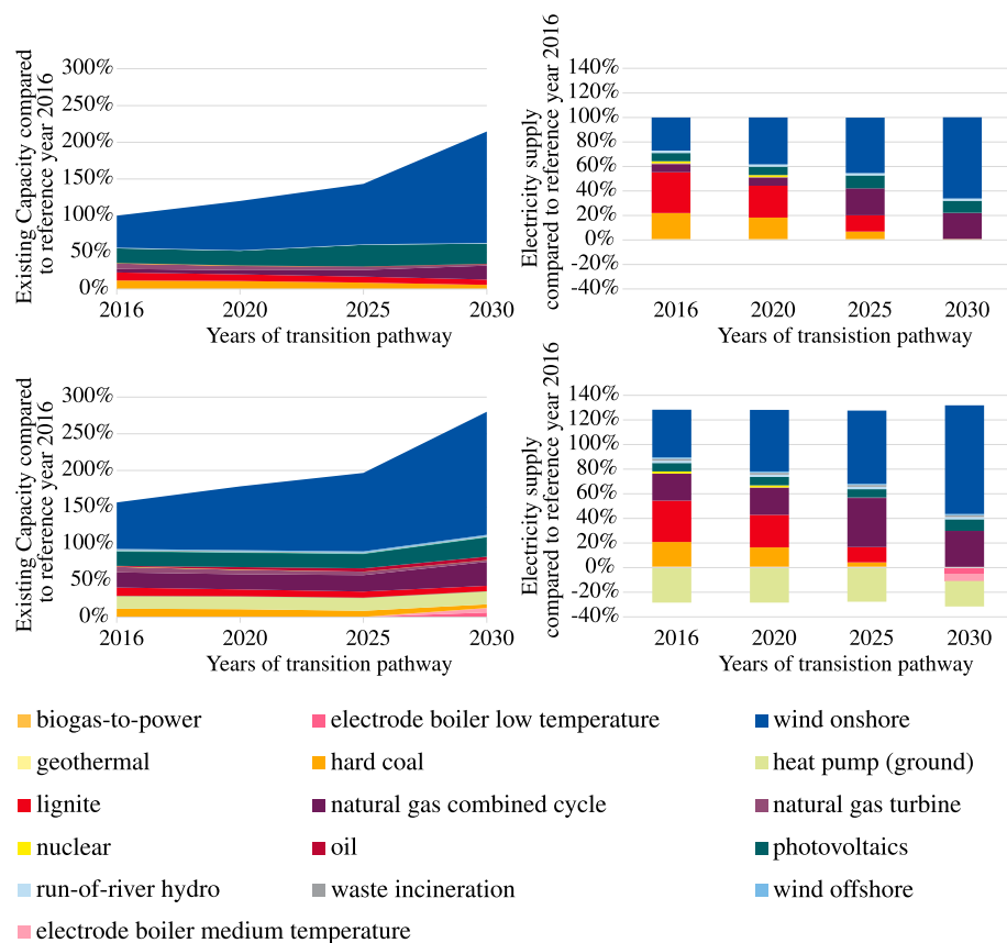
FIGURE 8 | Case studies considering the electricity, heat and transport sector without sector-coupling (top) and with sector-coupling (bottom). The left column shows the optimized production processes for electricity generation compared to the reference year of 2016 without sector coupling (Case 4). The right column shows the electricity production shares of the different production processes.
