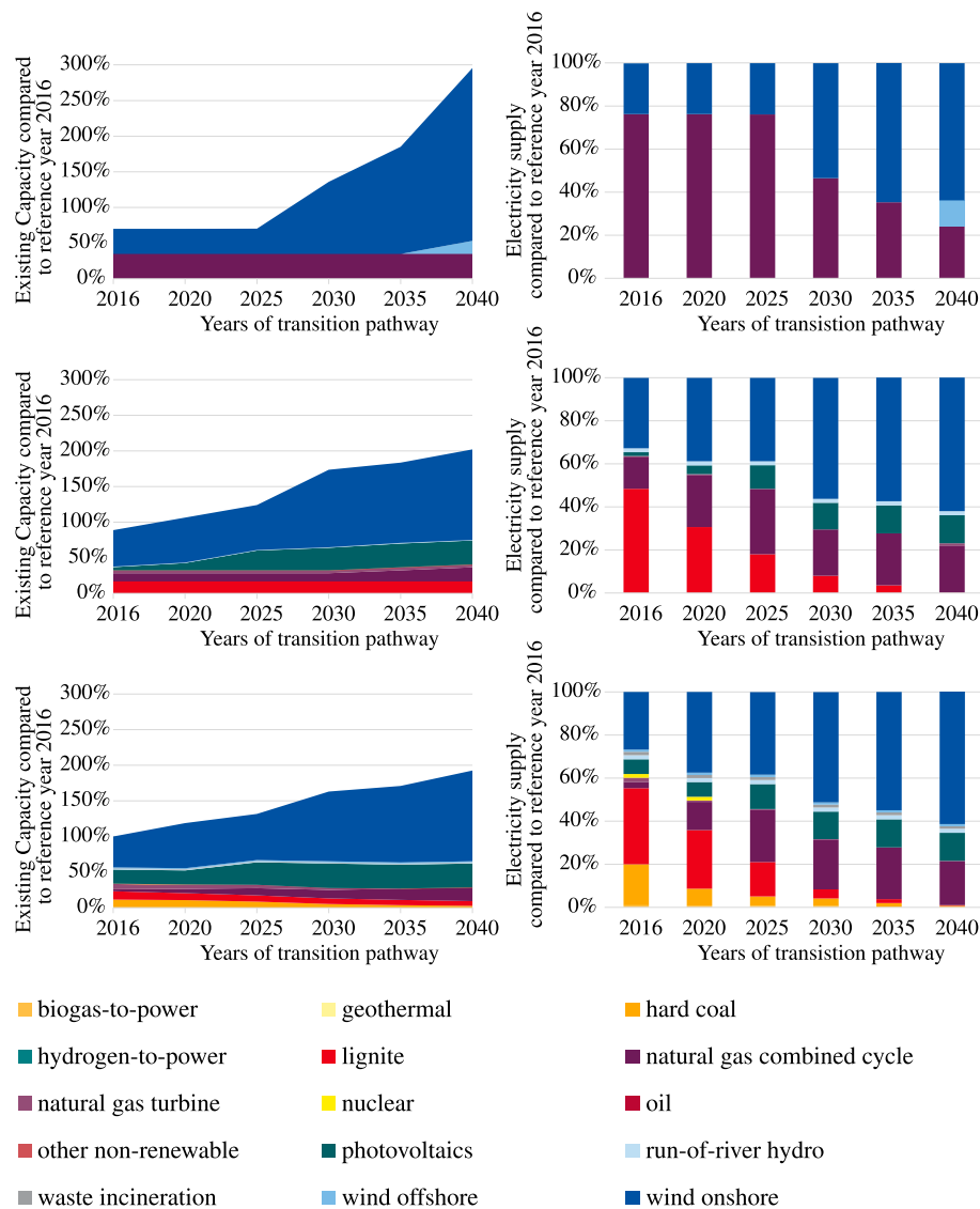
FIGURE 5 | Transition pathway of the German electricity sector until the year 2040 for three cases (Cases 1–3 in Table 3 from top to bottom). The left column shows the optimized production process capacity for electricity generation compared to the overall production process capacity in the reference case (Case 3, year 2016, as defined in Table 3 ). The right column shows the electricity production shares of the different production processes.
