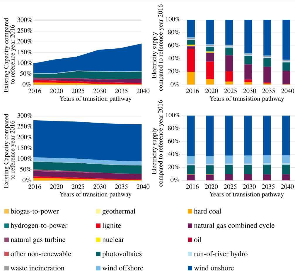
FIGURE 7 | Extended brownfield case with different objective functions: The upper figures show the cost minimal case, whereas the figures on the bottom show an environmental objective, where the global warming impact (GWI) of the system is minimized. The left column shows the optimized production processes for electricity generation compared to the reference year of 2016 in case study 3 (Table 3). The right column shows the electricity production shares of the different production processes.
