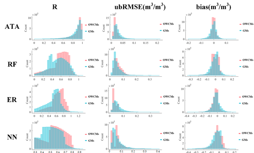
Figure 7. Frequency distributions of the statistical metrics R (1st column), ubRMSE (2nd column), and bias (3rd column) between the ATA (1st row)/RF (2nd row)/ER (3rd row)/NN (4th row)-based OWCM-/GM SM and the original RFSM over the QTP.
