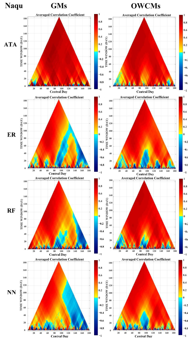
Figure 8. EDA-based average correlation coefficient R plots between GM-/OWCM-derived SM and the original RFSM in Naqu.
