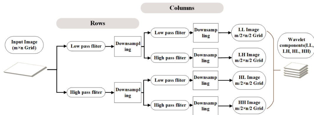
Figure 2. The block diagrams of the wavelet transformation in decomposing an n \times m image into four decomposed images.
