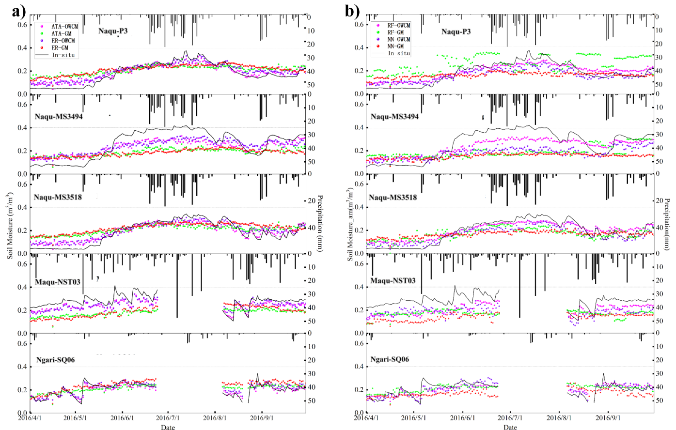
Figure 4. Time-series comparisons of daily GM-/OWCM-derived fine-RES SM with in situ SM measurements: (a) GM and OWCm results based on ATA and ER; (b) GM and OWCm results based on RF and NN.
