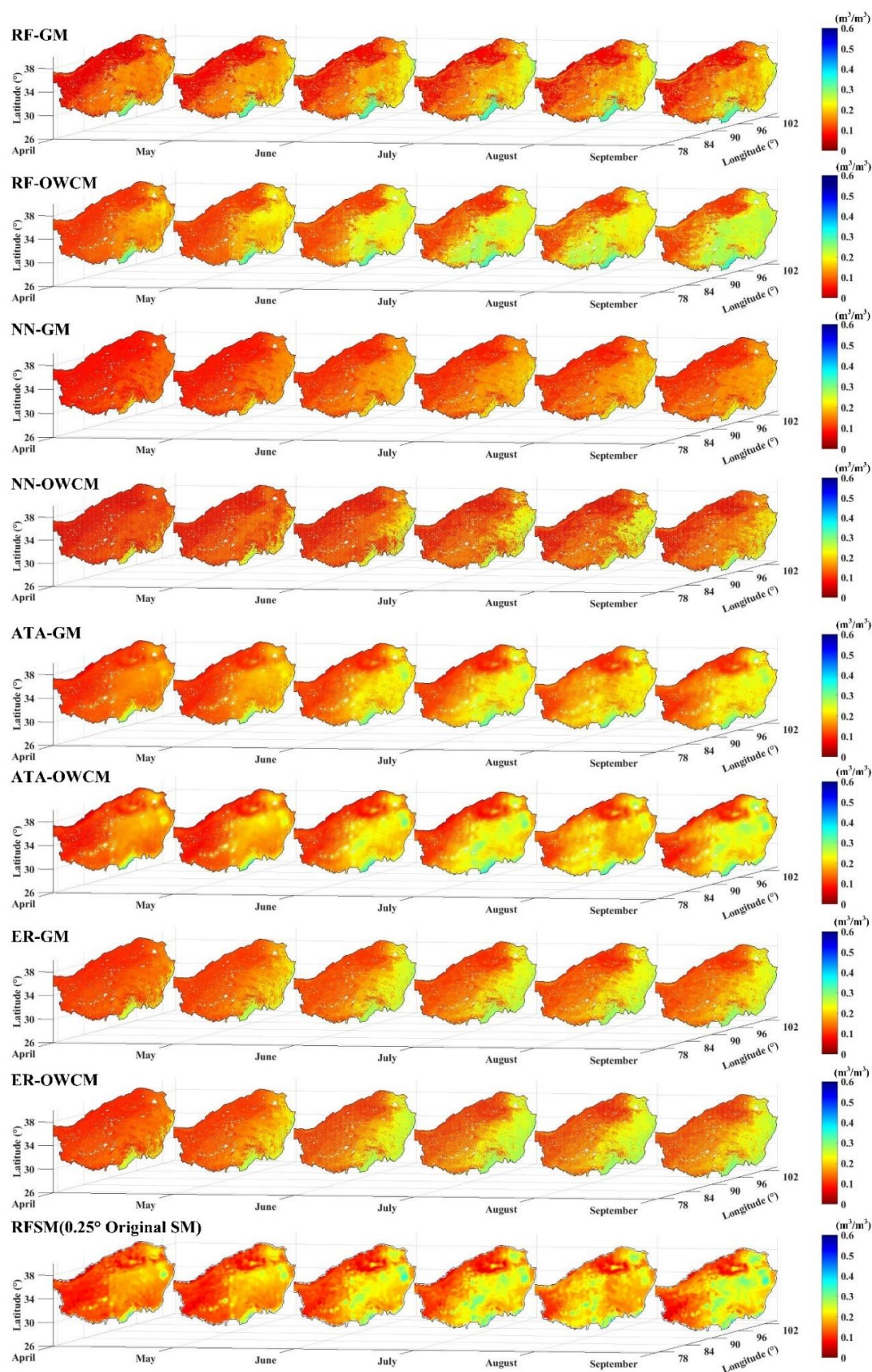
Figure 5. The spatial distribution of the monthly averaged SM products over the QTP during the 2016 unfrozen season, calculated from the corresponding GM-/OWCM-derived fine-RES SM, along with the original RFSM.
