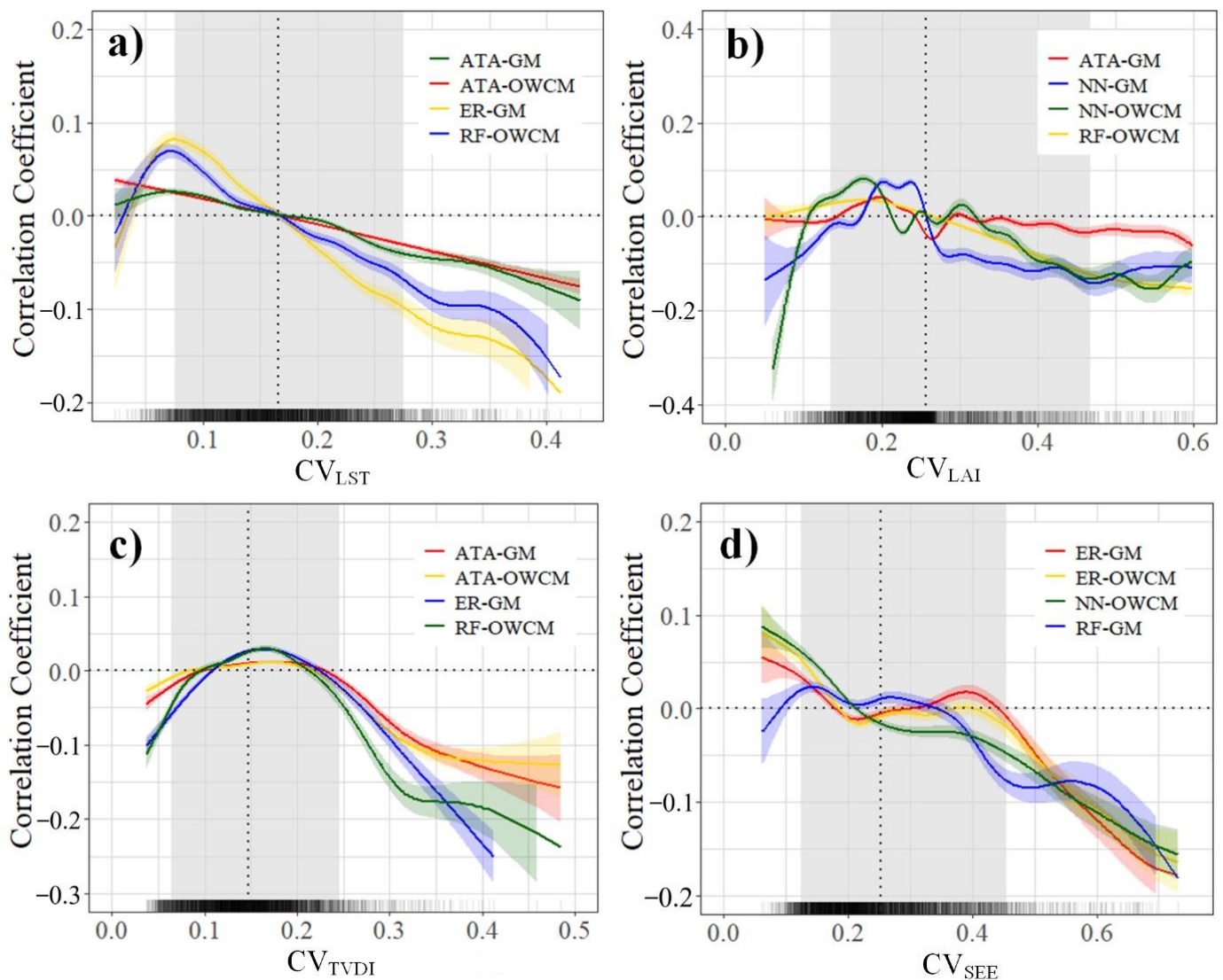
Figure 9. GAM partial effect splines presenting the dynamic changes in the fitting accuracy R with (a) CV_{LST} , (b) CV_{LAI} , (c) CV_{TVDI} , and (d) CV_{SEE} . In (a–d), the dotted lines indicate the zero value ( y -axis) and the means of explanatory variables ( x -axis), while the shaded areas are the 90% confidence intervals. Moreover, the small vertical lines at the bottoms of the figures represent data points.
