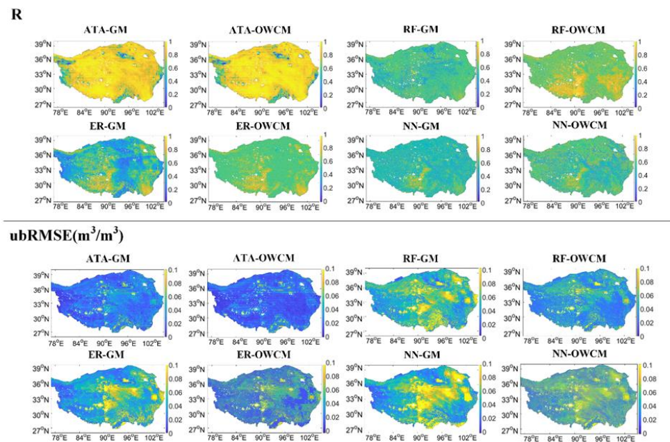
Figure 6. Spatial distributions of the statistical metrics R and ubRMSE between the aggregated OWCM-/GM-derived SM and the original RFSM.
