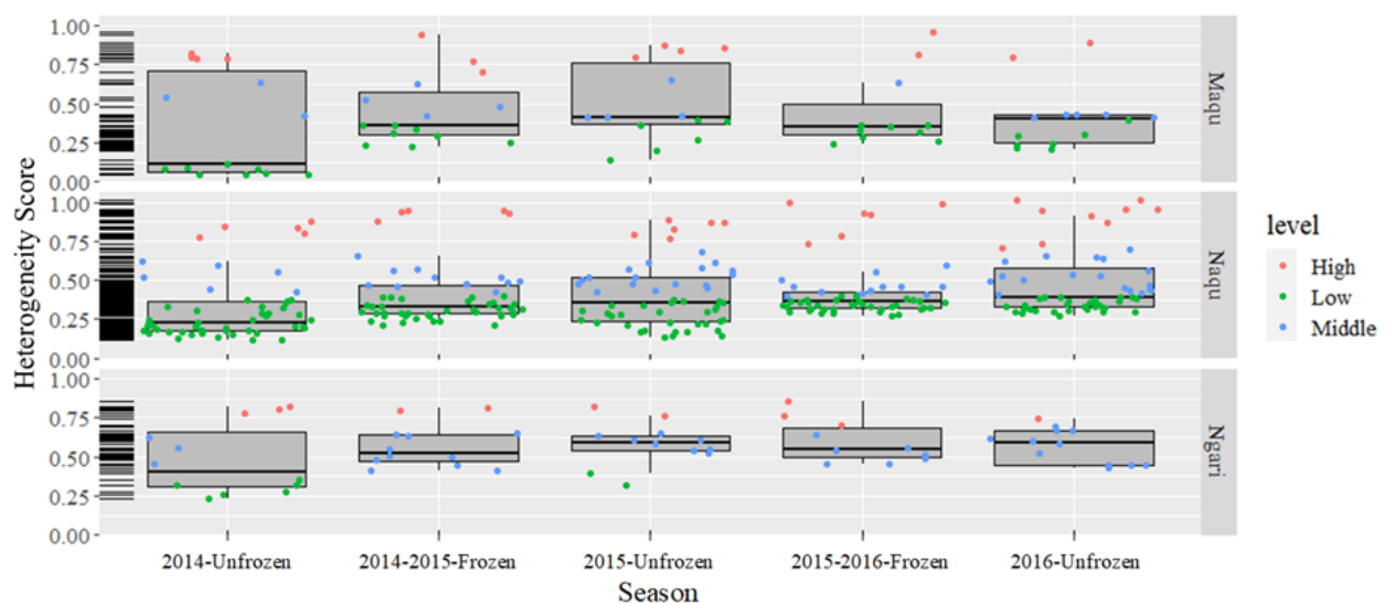
Figure 3. The heterogeneity distributions of all grid cells containing in situ measurement sites within the Naqu, Maqu, and Ngari networks. Green dots indicate low heterogeneity (score \leq 0.4 ), blue dots indicate moderate heterogeneity ( 0.4 < \text{score} \leq 0.7 ), and red dots indicate high heterogeneity ( 0.7 < \text{score} \leq 1 ).
