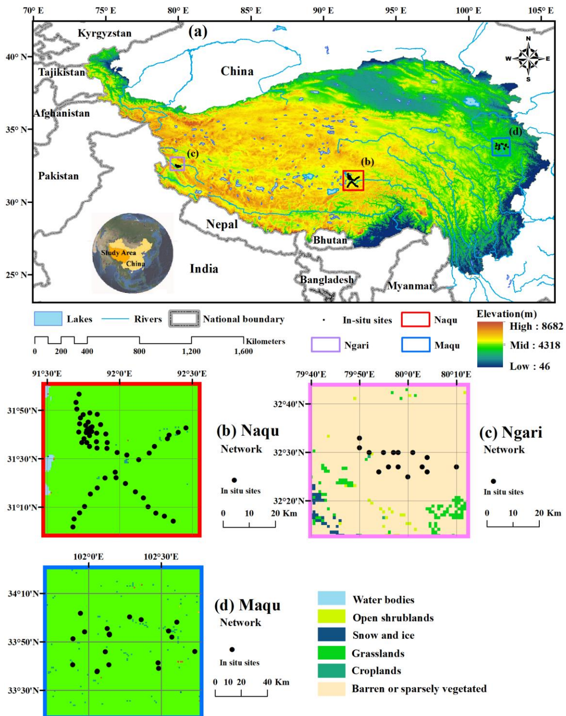
Figure 1. (a) The QTP study area and the (b) Naqu, (c) Ngari, and (d) Maqu in situ SM networks.
