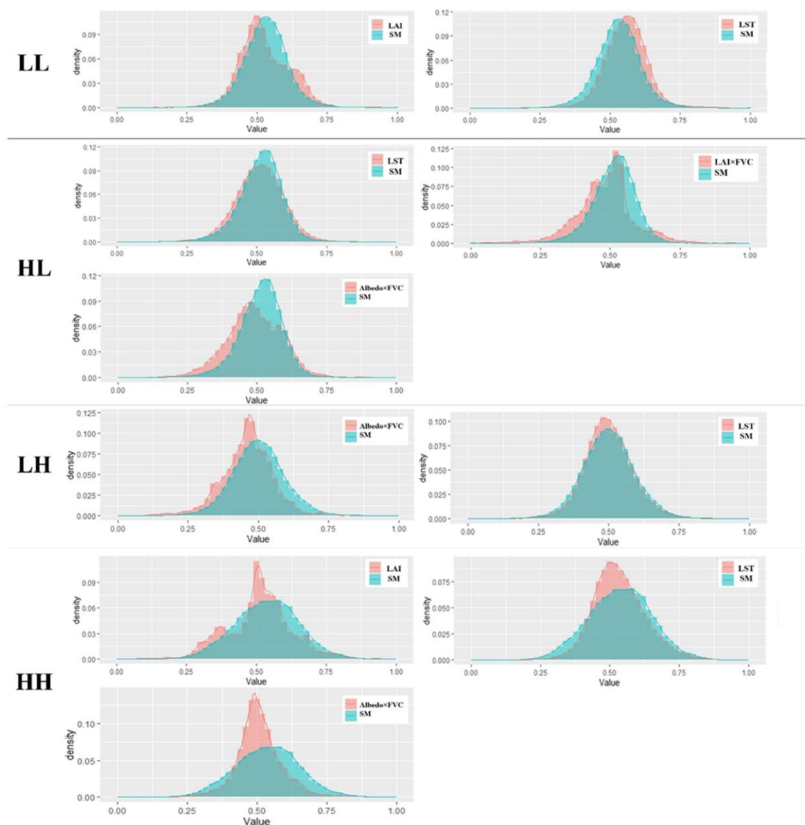
Figure A1. Frequency distributions in the probability density of the final selected fitting factors, with relatively good consistency with the frequency distribution of the original RFSM in the four WT components (LL, LH, HL, HH) over grassland.
