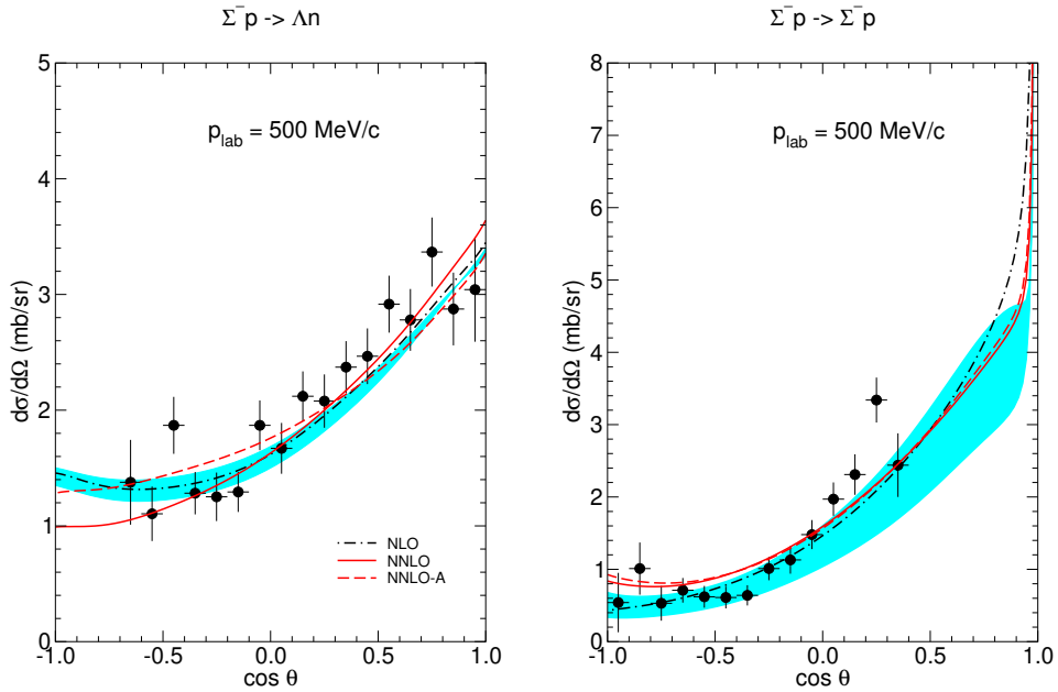
Figure 3. Differential cross sections for \Sigma^- p \rightarrow \Lambda n and \Sigma^- p \rightarrow \Sigma^- p . Same description of curves as in Fig. 1. Data are from the E40 Collaboration [21, 22] (momentum region 470-550 MeV/c).
