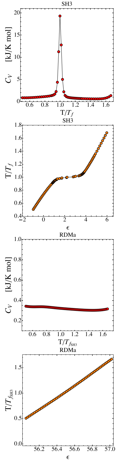
FIG. 3. The specific heat and the caloric curve for the SH3 protein show patterns typical of a phase transition (upper panels). These features are lost in the case of the randomized version of the correct sequence of the SH3 protein (lower panels).
