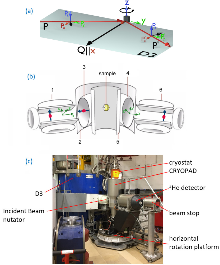
Figure 3.11: (a) Scattering geometry for the spherical neutron polarimetry measurement. P_i, P'_i denote i^{\text{th}} component ( i = x, y, z ) of the polarization of incident and diffracted beam, respectively. \mathbf{Q} is the scattering vector, which defines the x axis. (b) Pictorial representation of the different components of the CRYOPAD instrument (modified from Ref. [76]). 1: Incident beam nutator (magnetic path containing longitudinal static guide field). 2: Outer superconducting shield (Niobium) 3: Precession coil (rotates the incident beam polarization around a horizontal axis perpendicular to the incident beam). 4: Precession coil for diffracted beam (aligns the chosen polarization component to the axis of the diffracted beam). 5: Inner superconducting shield (protects magnetic field due to precession coils, and maintains a zero-field environment in the sample chamber). 6: Nutator of the diffracted beam (c) A picture of the CRYOPAD setup installed with the D3 setup. A few parts are also shown (taken from [77]).
