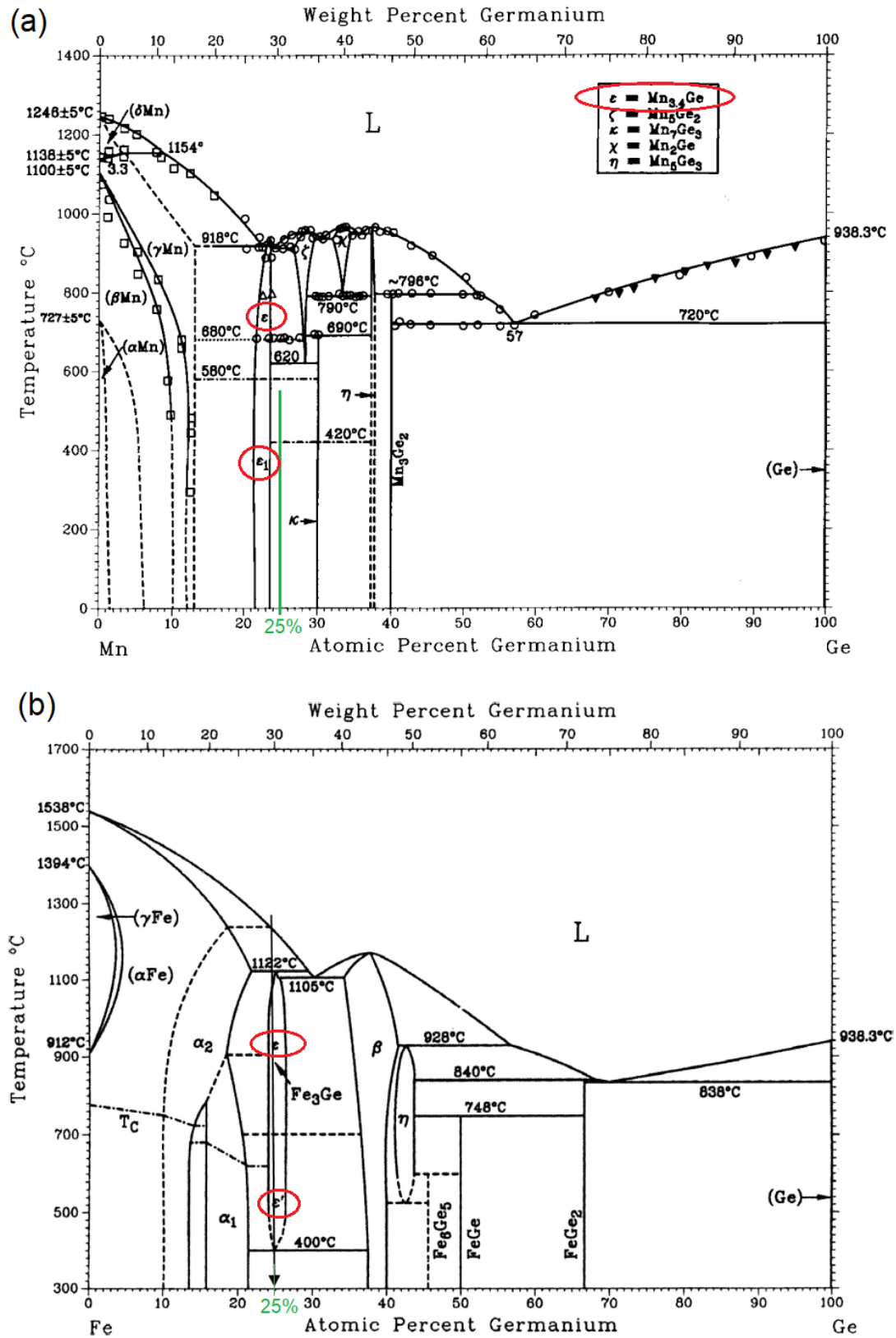
Figure 4.1: (a) Binary phase diagram of Mn - Ge[79]. (b) Binary phase diagram of Fe - Ge [81]. In both cases, \varepsilon and \varepsilon_1 phases (encircled by red) denote hexagonal and tetragonal phases.
