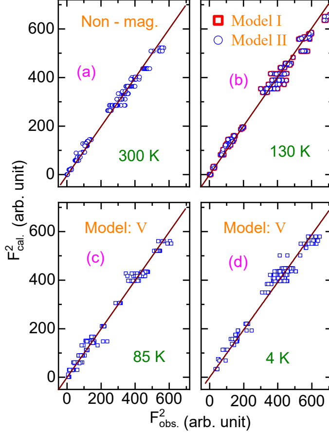
Figure 6.5: (a-d) Calculated (cal.) vs. observed (obs.) intensity at 300 K, 130 K, 85 K, and 4 K, respectively. Except at 300 K, the intensities at 4 K, 85 K, and 130 K correspond to the magnetic and nuclear contributions. The fitted models are mentioned in each plot and shown in the Fig. 6.6.
