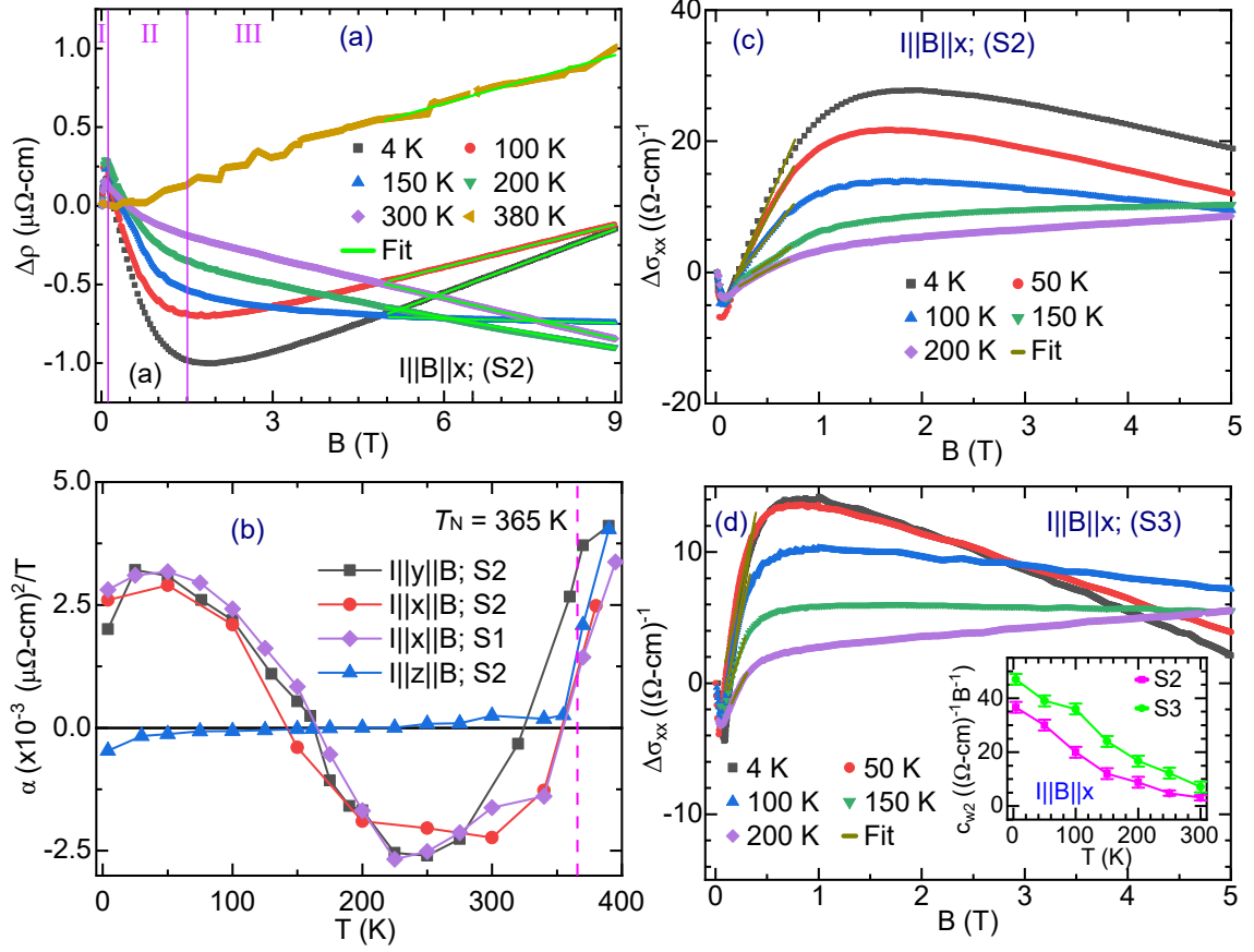
Figure 5.4: (a) shows LMR along the x axis, corresponding to the \text{Mn}_3\text{Ge} . Here, \Delta\rho = \rho(B) - \rho(0) . At high field ( B > 5 T), the data is fitted with \rho_{[\text{high } B]} = \alpha(B/\rho_0) , and fitting is denoted as ‘Fit’. I, II, and III denote three different field regimes where the nature of LMR is different. (b) Temperature dependence of \alpha (high field slope) corresponding to different samples. (c), and (d) show LMC along the x axis, for S2 and S3 samples, respectively. Here, \Delta\sigma_{ii} = \sigma_{ii}(B) - \sigma_{ii}(0) . In the case of S2 and S3 samples, LMC below 0.8 T and 0.4 T, respectively, is fitted with \sigma_{[\text{low } B]} = c_{w2}B . The evolution of c_{w2} with temperature is shown in (d) inset.
