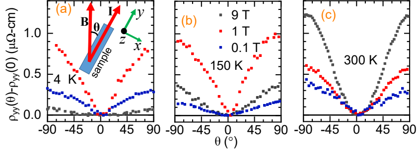
Figure 5.11: (a-c) denote \theta\text{MR} corresponding to the I\|B\|y ; B rotated from y to the x axis. The experimental setup is illustrated in (a).
