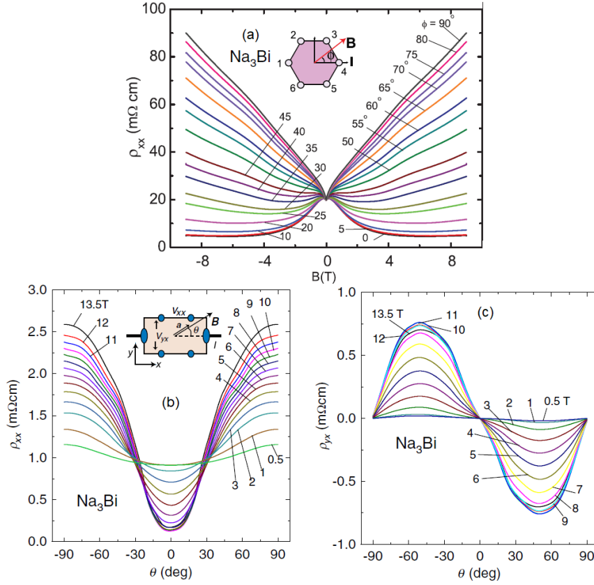
Figure 2.10: (Ref. [39, 40]) Chiral anomaly in Dirac semimetal - \text{Na}_3\text{Bi} . \text{Na}_3\text{Bi} becomes Weyl semimetal under the application of the external magnetic field, because of the broken TR symmetry. The Dirac cones split into Weyl cones in the same direction as the field is applied. When the magnetic field is applied parallel to the electric current, chiral anomaly-induced negative magneto-resistance (MR) is observed, as shown in (a), corresponding to the \text{Na}_3\text{Bi} Dirac semimetal. Angular MR and planar Hall effect for the \text{Na}_3\text{Bi} is shown in (b, c), respectively. Sample contacts and measurement setup for (b, c) are shown in the (b) inset.
