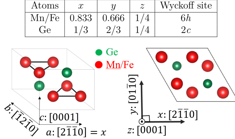
Figure 4.2: The table on the top shows the position of atoms corresponding to space group P6_3/mmc . The figure below shows nuclear structure of (\text{Mn}_{1-\alpha}\text{Fe}_{\alpha})_3\text{Ge} in two different orientations.
