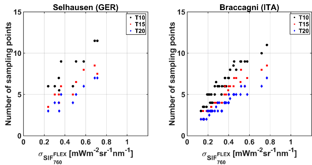
Figure 4. The 95th percentile of the number of sampling points needed to meet the thresholds for the FLEX pixels in Selhausen (Germany) and Braccagni (Italy) experimental sites using a random sampling approach.
