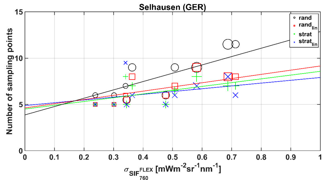
Figure 6. The 95th percentile of the number of sampling points needed to meet the T10 thresholds for the FLEX pixels in Selhausen (Germany) experimental site using a random sampling, a random sampling with a linear combination model, a stratified random sampling and a stratified random sampling with a linear combination model. The number of sampling points is shown in relation to \sigma_{SIF_{760}^{FLEX}} . The pointer size is related to the number of components within each FLEX pixel (2–4). The solid lines show the linear OLS regressions for each sampling strategy.
