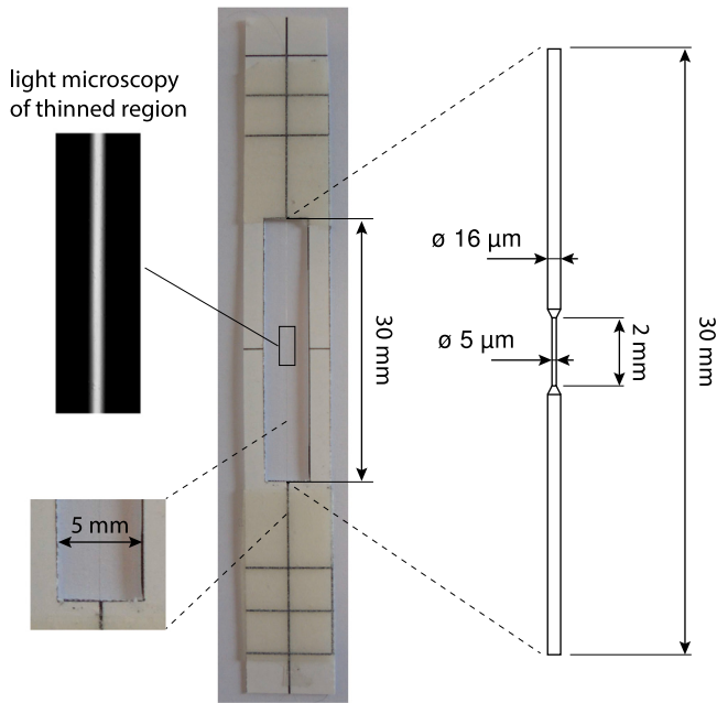
Fig. 2. Photo of a paper frame containing a 16 µm W wire attached by a two component epoxy (UHU Plus endfest 300). Extract shows schematically the geometry of the testing area where the centre part is thinned to a diameter of 5 µm over a length of 2 mm. On the left side an optical microscopy image of the thinned region is shown.
