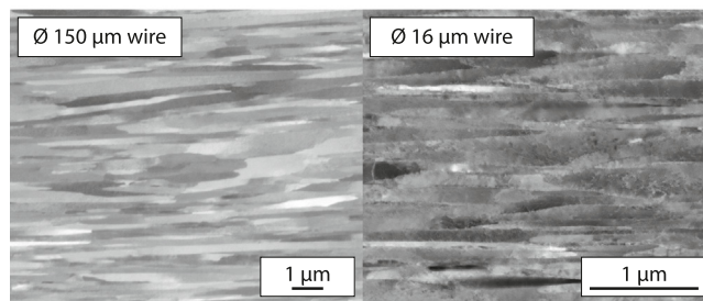
Fig. 1. Scanning electron microscopy (SEM) pictures of the longitudinal section of tungsten wire with a diameter of 150 µm (left) and 16 µm (right) (Z contrast using the circular backscatter detector (CBS)). Both sections were prepared by a focussed ion beam polishing within the SEM. The magnifications are chosen to show similar sizes for the grains but note the differences in the scale bars (ratio 1:3.5).
