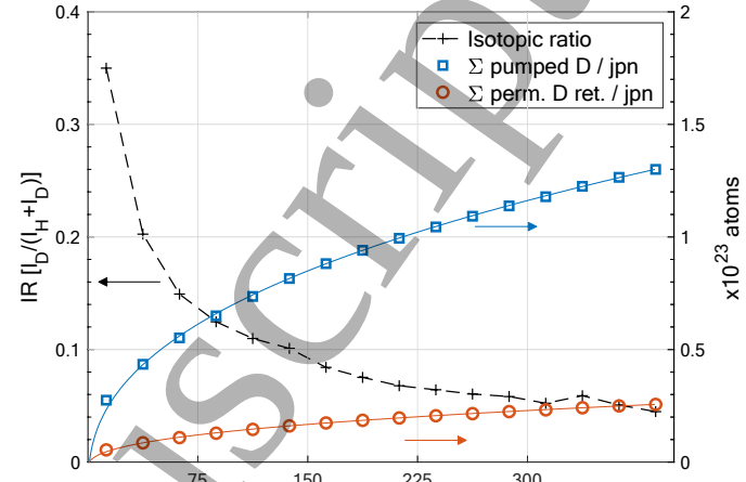
Figure 7 : Isotopic exchange from D to H by tokamak plasma on JET-ILW (2014 experiment [6]) with I_p = 2.0 MA, B_T = 2.4 T, \langle n_e \rangle = 4.5 \times 10^{19} \text{ m}^{-3} , constant gas injection of 3.0 \times 10^{21} \text{ D.s}^{-1} and 0.5MW of ICRH heating in L-mode. Left: Isotopic ratio by subdivertor penning gauge spectroscopy. Right: integral of removal by pumps and redeposition of atoms as function of the total discharge time; blue and red trend line follow envelope curve \Sigma t^{-0.6} \Delta t .
