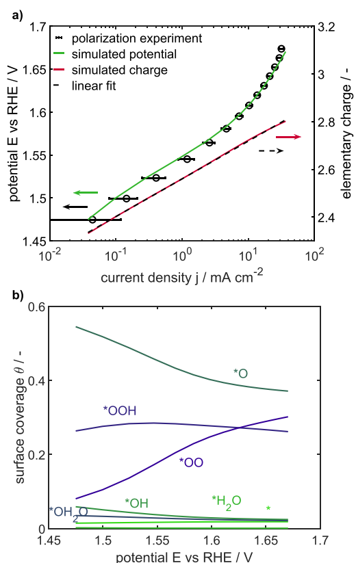
Figure 6. a) Experimental and simulated polarization curves for technically relevant potentials and the simulated change in elementary charge per active site. Experiments were repeated three times. (b) Corresponding surface coverages of the steady-state simulation.
