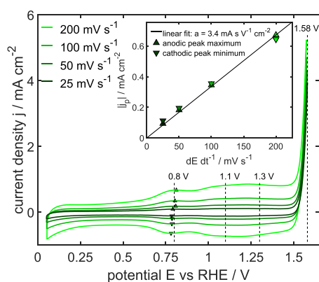
Figure 1. Cyclic voltammograms of pristine rutile \text{IrO}_2 nanoparticles in 0.1 M \text{H}_2\text{SO}_4 at different scan rates. The inset shows the linear current behavior of the absolute peak maximum at around 0.8 V. All potentials are referred to RHE and are iR -corrected.
