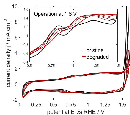
Figure 2. Changes in experimental CV curves with a scan rate of 200 \text{ mV s}^{-1} during 15 h of OER operation at a constant potential of 1.6 V versus RHE. The third CV curve recorded after every 150 min is displayed, with colors changing from pristine (black) to the degraded state (red); changes are indicated by arrows. The inset magnifies the shift in anodic redox transitions.
