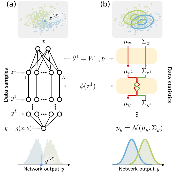
FIG. 1. (a) Network analysis based on data samples considers each data sample x^{(d)} separately as it passes through the network, producing a single corresponding output y^{(d)} . Each layer consists of an affine transformation (W^l, b^l) followed by a non-linearity \phi applied componentwise. (b) Network analysis based on data statistics considers how the entire data distribution p(x) is transformed by the network. At each step, the intermediate distribution is parameterized by its cumulants, the most important of which are the mean \mu and the covariance \Sigma . The affine step transforms \mu and \Sigma independently, while the non-linearity \phi causes a non-trivial interaction of the two.
