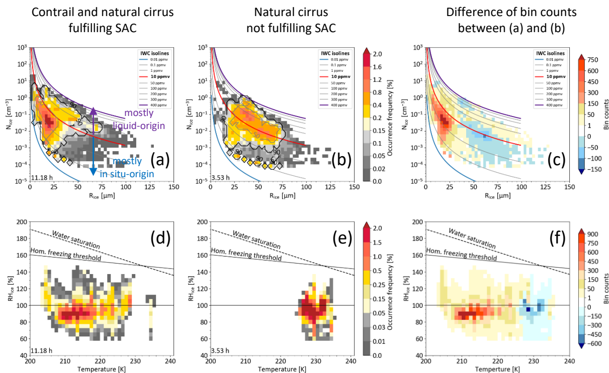
Figure 4. Upper panels: similar to Fig. 3c, but for (a): the Schmidt-Appleman criterion (SAC) fulfilled dataset of contrail and natural cirrus (median: N_{ice} = 0.04 \text{ cm}^{-3} and R_{ice} = 20.6 \mu m ); (b) the SAC unfulfilled dataset of natural cirrus (median: N_{ice} = 0.018 \text{ cm}^{-3} and R_{ice} = 42.4 \mu m ); (c): the difference of data points between a and b in single N_{ice} – R_{ice} bins. Lower panels: similar to Fig. 3d, but for (d): the dataset of contrail or natural cirrus fulfilling SAC; (e): the natural cirrus not fulfilling the SAC; (f): the difference of data points between d and e in single RH_{ice} – T_{amb} bins.
