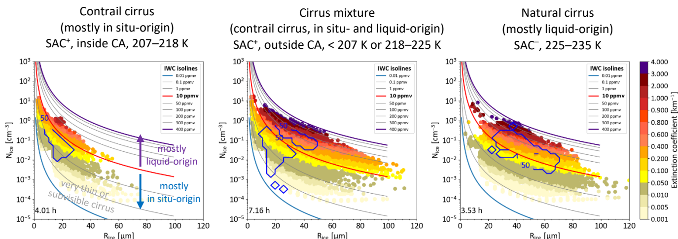
Figure 11. Ice crystal number concentration N_{ice} vs. mass mean radius R_{ice} colour coded with extinction coefficient Ext (unit: km^{-1} ) of ice particles. Ice water content IWC isolines in relation to N_{ice} and R_{ice} are also plotted. Left: the contrail cirrus that fulfil the Schmidt-Appleman criterion (SAC) inside the cruising altitude (CA; ambient pressure 200–245 hPa, ambient temperature 207–218 K), also identified as in situ-origin cirrus; median: N_{ice} = 0.045 cm^{-3} , R_{ice} = 16.6 μm , IWC = 3.5 ppmv , Ext = \sim 0.056 km^{-1} . Middle: the cirrus mixture (fulfilling SAC and outside the CA range), which is a mixture of contrail cirrus, in situ- and liquid-origin natural cirrus; median: N_{ice} = 0.038 cm^{-3} , R_{ice} = 24.1 μm , IWC = 8.3 ppmv , Ext = \sim 0.096 km^{-1} . Right: the natural cirrus of liquid-origin (not fulfilling SAC and below the CA range); median: N_{ice} = 0.018 cm^{-3} , R_{ice} = 42.4 μm , IWC = 21.7 ppmv , Ext = \sim 0.137 km^{-1} . The 50% (blue) contour enclose 50% the most frequently occurring ice crystals. The total sampling hours of each cirrus dataset at 1 Hz sampling frequency are inserted in the lower left corners of the figures.
