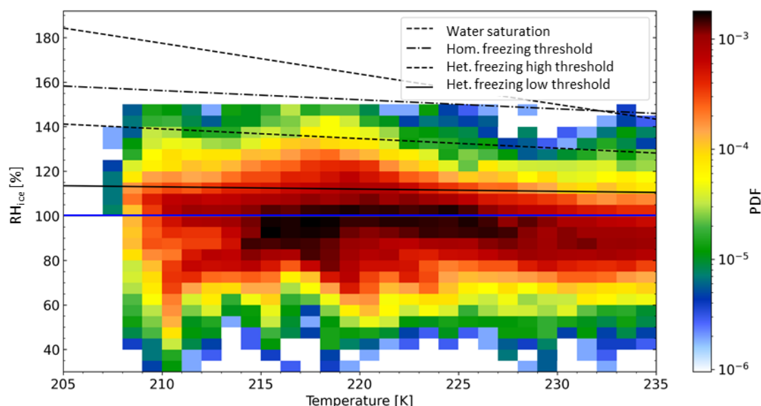
Figure 8. Probability distribution of in-cloud RH_{ice} measured by the lidar WALES below 235 K in dependence on ECMWF model temperature. Only the cloud particles producing a back-scattering ratio greater than 3 and depolarisation greater than 20% included in the plot. The water saturation (Murphy and Koop, 2005), homogeneous freezing threshold (Koop et al., 2000), and heterogeneous freezing high (mineral dust as ice nucleating particles) and low (coated soot) thresholds (Krämer et al., 2016) are added in the figure.
