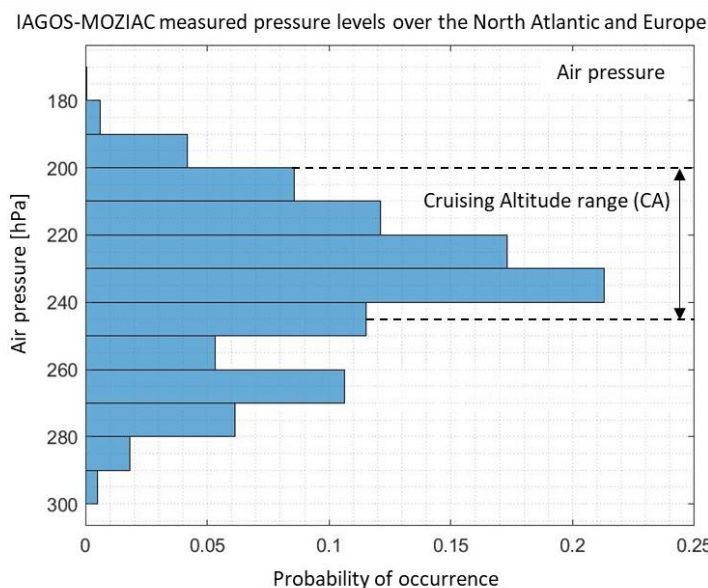
250 Figure 2. Occurrence fractions of passenger aircraft flight levels in pressure (unit: hPa) measured during the IAGOS-MOZAIC period (1996–2010) over the North Atlantic and Europe. The pressure range 200–245 hPa between the dashed lines is adopted as the most frequent aircraft cruising altitude (CA) range (see text for the determination of the boundary pressure thresholds).
