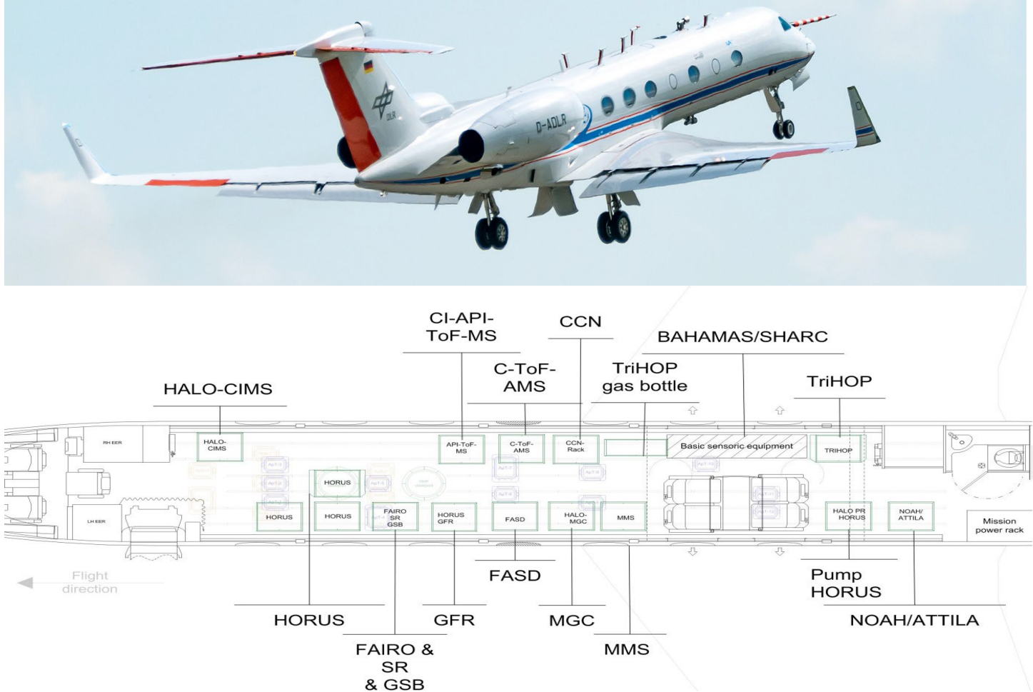
Fig. 4. (top) Photo and (bottom) cabin layout of the comprehensive trace gas and aerosol instrumentation of HALO during BLUESKY.
