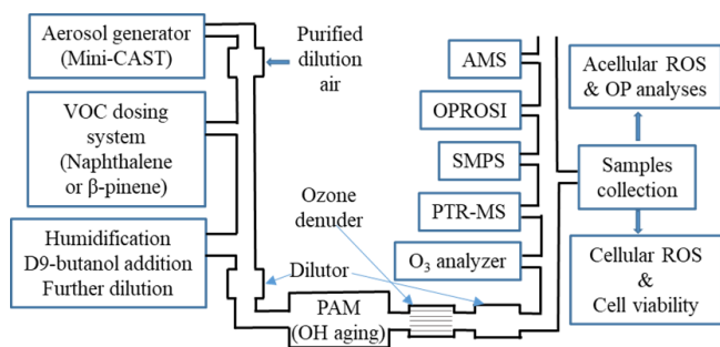
Figure 1. A schematic of the experimental setup for SOA generation and characterization. SOA was generated from naphthalene and \beta -pinene condensed on soot particles (SP) from a miniature combustion aerosol standard (mini-CAST) soot generator under varied atmospheric conditions (UV lamp intensity and humidity). Several online instruments were used for a comprehensive gas- and particle-phase characterization (including the online ROS instrument OPROSI). Filter samples were collected for various chemical and biological offline analyses.
