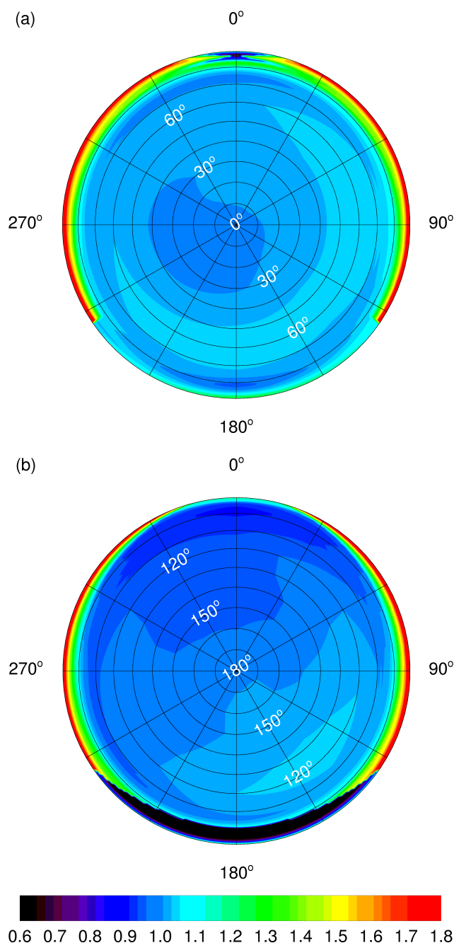
Figure 5. Contour plots of HALO total relative angular sensitivities Z_p^T of the FLT 4\pi receiver combination at 400 nm (top views). (a) Upper hemisphere, (b) lower hemisphere. An azimuth angle of 0° corresponds to the flight direction. Polar angles of incidence are indicated (white). For the FLT configuration field-of-view and fuselage reflection effects are considered including the influence of a containment on the lower fuselage causing missing cross-talk in panel (a) and dark areas in panel (b) in rearward directions. Note that compared to Fig. 3, the features in the lower panel are laterally reversed because the receiver is now facing downwards.
