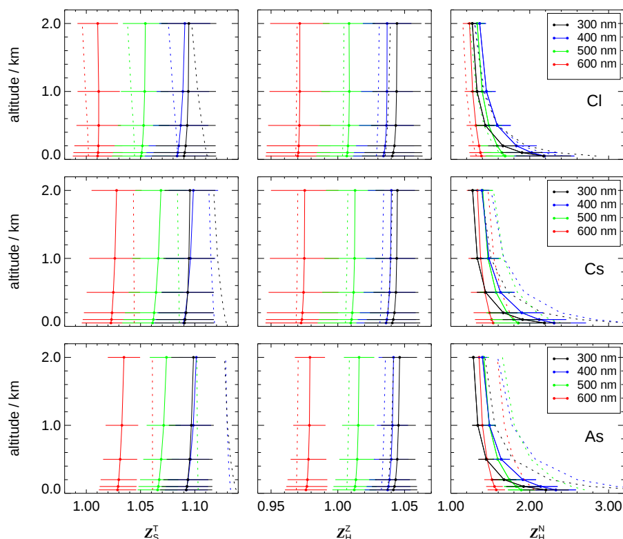
Figure 10. Altitude dependence of modelled Zeppelin correction functions Z_S^T , Z_H^Z and Z_H^N for total, downward and upward spectral actinic flux densities for a solar zenith angle of 40^\circ and selected wavelengths. Corrections apply to normal aerosol load and ground albedos at different cloud cases. Top row (CI): clear-sky; middle row (Cs): Cs cloud layer; bottom row (As): As cloud layer. Error bars include the effects of \pm 5^\circ attitude variations. Dashed lines show results assuming hemispherical-isotropic distributions of downward and upward diffuse spectral radiances.
