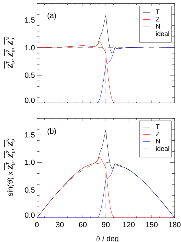
Figure 6. (a) Azimuthal averages of total relative angular sensitivities Z_p^T (T) shown in Fig. 5 with contributions Z_p^Z (Z) and Z_p^N (N) of top and bottom receivers, respectively, for a wavelength of 400 nm. The sensitivities of ideal 2π- and 4π-receivers are shown for comparison (dashed lines). (b) The same data as in (a) but multiplied with \sin(\vartheta) to account for the \vartheta -dependence of solid angle contributions.
