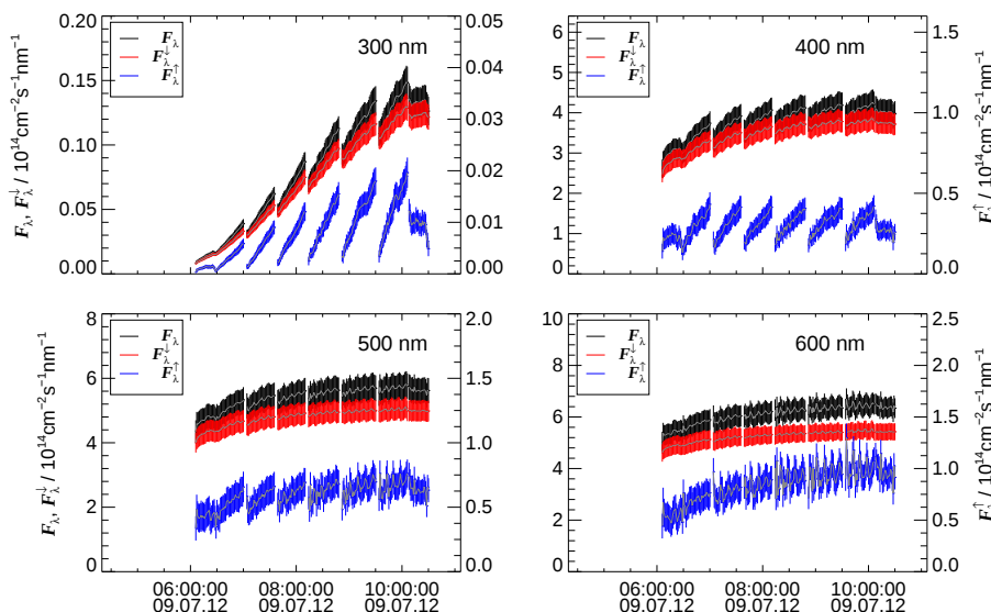
Figure 15. Total ( F_\lambda ), downward ( F_\lambda^\downarrow ) and upward ( F_\lambda^\uparrow ) spectral actinic flux densities of the Zeppelin flight shown in Fig. 14 for the four selected wavelengths. The error bars correspond to total uncertainties including those from corrections and calibrations (Sect. S7, Supplement). The right hand y -axes refer to the F_\lambda^\uparrow . The small, about 10-min periodic patterns were induced by the circular flight pattern.
