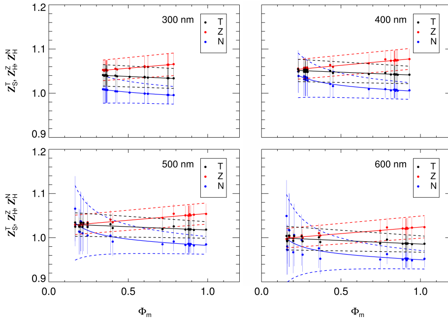
Figure 13. Correction functions Z_S^T (T), Z_H^Z (Z) and Z_H^N (N) for HALO at an altitude of 5 km, a solar zenith angle of 40^\circ and selected wavelengths as a function of \Phi_m (ratio of uncorrected upward/downward spectral actinic flux densities). Data points with error bars show the results for all relevant atmospheric scenarios (Tab. S1, Supplement) for a solar heading angle \gamma_o = 90^\circ of the FLT configuration. Full lines are parametrizations with estimated uncertainty ranges indicated by the dashed lines. A second example for a solar zenith angle of 70^\circ is shown in Fig. S30 of the Supplement.
