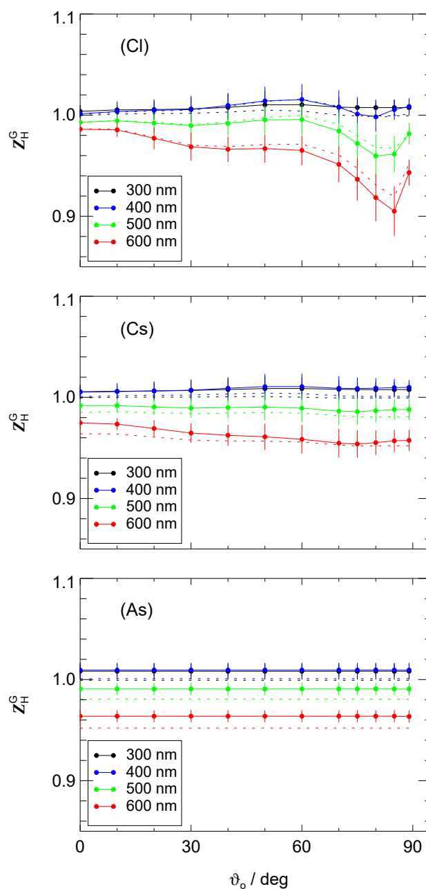
Figure 9. Modeled correction functions Z_H^G for ground-based measurements of downward spectral actinic flux densities with the HALO top receiver as a function of solar zenith angle for selected wavelengths. Corrections apply to a scenario with normal aerosol load and ground albedos at different cloud cases. Upper panel (CI): clear-sky; middle panel (Cs): Cs cloud layer; lower panel (As): As cloud layer. Dashed lines show results assuming isotropic distributions of downward diffuse spectral radiances for comparison.
