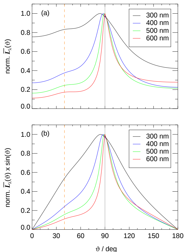
Figure 8. (a) Polar angle of incidence dependence of normalized, azimuthal mean diffuse spectral radiances for different wavelengths under the conditions in Fig. 7. (b) Azimuthal mean spectral radiances as in panel (a) but weighted with \sin(\vartheta) . The vertical grey line indicates the horizon, the dashed orange line the solar zenith angle. Direct sun contribution to spectral actinic flux densities for this scenario are 0.35 (300 nm), 0.53 (400 nm), 0.67 (500 nm) and 0.73 (600 nm). Compare with Fig. S18 of the Supplement.
