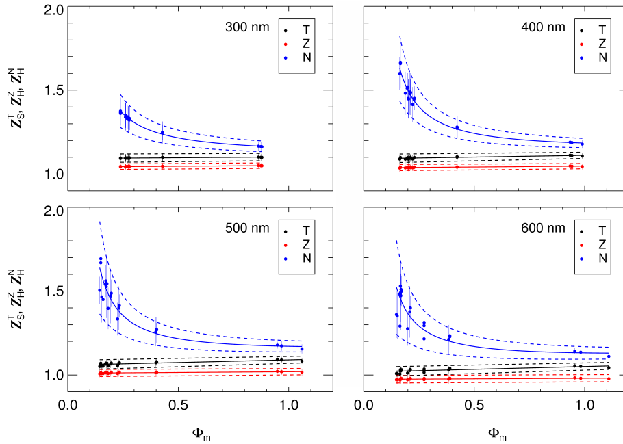
Figure 12. Correction functions Z_S^T (T), Z_H^Z (Z) and Z_H^N (N) for the Zeppelin at an altitude of 1 km, a solar zenith angle of 40^\circ and selected wavelengths as a function of \Phi_m (ratio of uncorrected upward/downward spectral actinic flux densities). Data points with error bars show the results for all relevant atmospheric scenarios (Tab. S1, Supplement). Full lines are parametrizations with estimated uncertainty ranges indicated by the dashed lines. A second example for a solar zenith angle of 70^\circ is shown in Fig. S29 of the Supplement.
