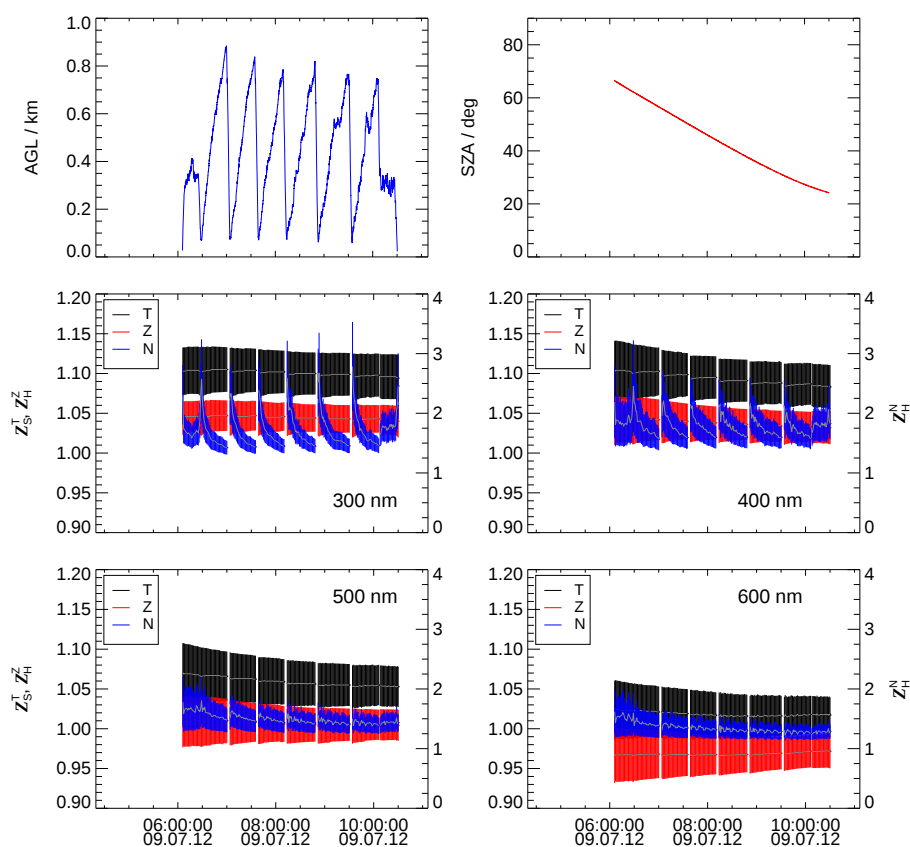
Figure 14. Zeppelin flight example with height profiles on 09 July 2012 about 40 km east of Bologna, Italy (PEGASOS campaign). Upper panels: Heights above ground, (AGL, left) and solar zenith angles (SZA, right) as a function of time of day (UTC). Middle and lower panels: Parametrized correction functions Z_S^T (T), Z_H^Z (Z) and Z_H^N (N) for four selected wavelengths with error bars indicating uncertainties. For clarity, 1-minute averages are shown with grey overlays. The right hand y-axes refer to the Z_H^N .
