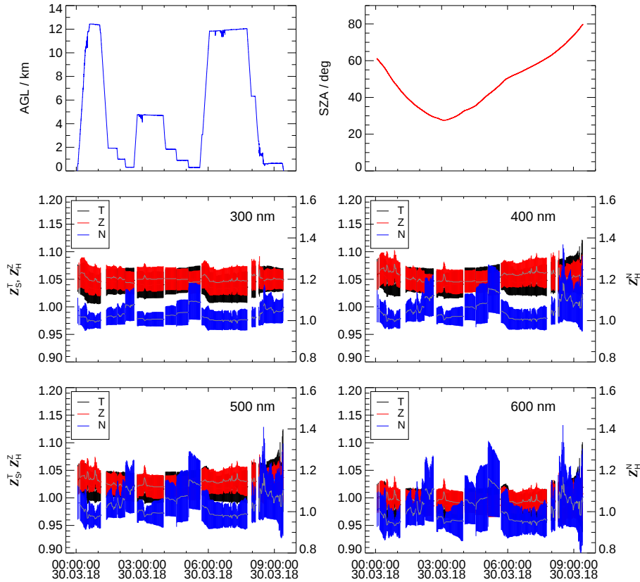
Figure 16. HALO flight example with a return flight from Taiwan to Japan on 30 March 2018 over the East China Sea (EMerGe campaign). Upper panels: Heights above ground (AGL, left) and solar zenith angles (SZA, right) as a function of time of day(UTC). Middle and lower panels: Parameterized correction functions Z_S^T (T), Z_H^Z (Z) and Z_H^N (N) for four selected wavelengths with error bars indicating uncertainties (FLT configuration). For clarity, 1-minute averages are shown with grey overlays. The right hand y -axes refer to the Z_H^N .
