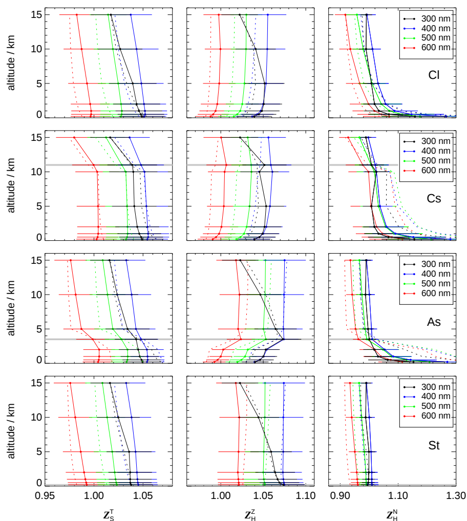
Figure 11. Altitude dependence of modelled HALO correction functions Z_S^T , Z_H^Z and Z_H^N for total, downward and upward spectral actinic flux densities for a solar zenith angle of 40^\circ and selected wavelengths. Corrections apply to normal aerosol load, normal ground albedos and a solar heading angle \gamma_o = 90 \pm 22^\circ of the HALO configuration FLT for four cloud cases. Top row (CI): clear-sky; middle upper row (Cs): Cs cloud layer; middle lower row (As): As cloud layer; lower row (St): St cloud layer. Cloud layer heights are indicated by horizontal grey lines. Error bars include the effects of \pm 2.5^\circ attitude variations. Dashed lines show results assuming hemispherical-isotropic distributions of downward and upward diffuse spectral radiances.
