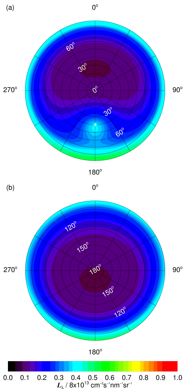
Figure 7. Contour plots of modelled diffuse spectral radiance distributions for a wavelength of 400 nm at an altitude of 5 km under clear-sky conditions at solar zenith and azimuth angles of 40° and 180°, respectively. (a) Downward spectral radiance. (b) Upward spectral radiance. Polar angles (white) are defined as angles of incidence. The position of the sun is indicated by the white cross in panel (a). In this example, ground albedos were scaled to 0.04 at 470 nm and aerosol optical depths to 0.2 at 550 nm (normal conditions). The colour scale was chosen for better comparability with Fig. S17 where the effects of an underlying As cloud layer are shown.
