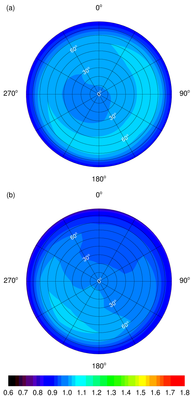
Figure 3. Contour plots of hemispherical relative angular sensitivities Z_p of HALO 2\pi (a) top and (b) bottom receivers at 400 nm (top views). Azimuth angles of 0^\circ correspond to flight directions of aircraft-installed receivers. Polar angles of incidence are indicated (white). Note that cross-talk to the lower hemisphere is invisible in this representation. The color scale was chosen for better comparability with Fig. 5.
