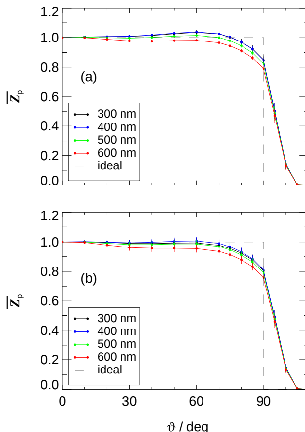
Figure 4. Azimuthal averages of relative angular sensitivities Z_p of HALO (a) top and (b) bottom receivers for selected wavelengths. Error bars indicate standard deviations of the azimuthal variabilities. The sensitivity of an ideal 2\pi receiver is shown for comparison (dashed line). The receivers were built into substitutes of aircraft flanges as shown in Fig. 1.
