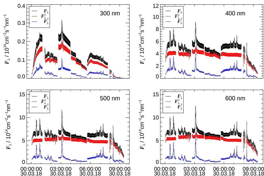
Figure 17. Total ( F_\lambda ), downward ( F_\lambda^{\downarrow} ) and upward ( F_\lambda^{\uparrow} ) spectral actinic flux densities of the HALO flight shown in Fig. 16 for the four selected wavelengths. The error bars correspond to total uncertainties including those from corrections and calibrations (Sect. S7, Supplement).
