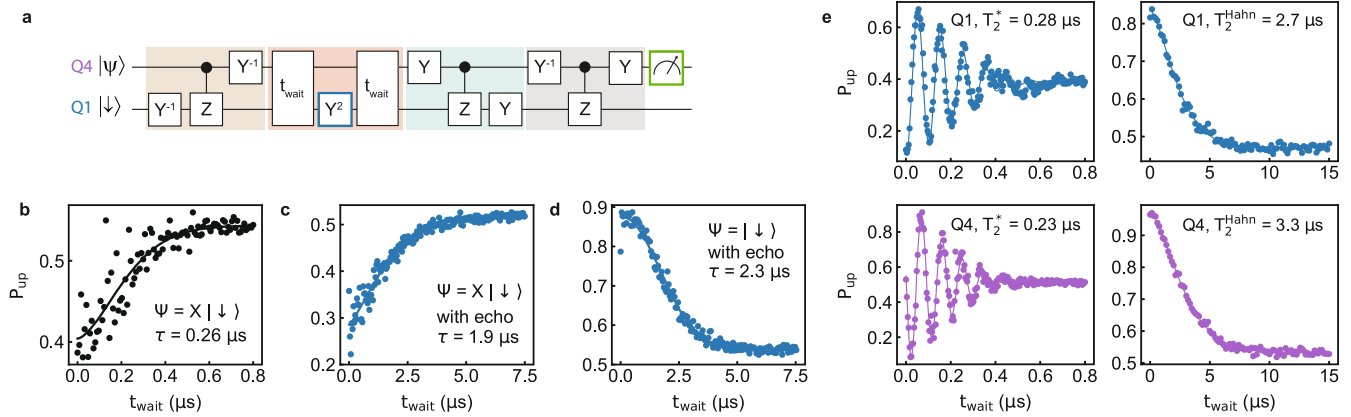
Fig. 2 Two-qubit phase flip code. a Circuit diagram. The encoding, decoding and correction are implemented using a combination of Y , Y^{-1} and CZ gates. By adding a wait time ( t_{\text{wait}} ) after the encoding, phase errors will occur due to the dephasing of the qubits. Q4 is the data qubit and Q1 the ancilla qubit. b–d P_{\text{up}} as a function of t_{\text{wait}} when executing the two-qubit phase flip code, which gives a decay time \tau . Results for the data qubit prepared in |\Psi\rangle = X|\downarrow\rangle (b), and through single-qubit gates projected to a basis state for readout, without an echo pulse Y^2 (b), with an echo pulse Y^2 (c), and with an echo pulse with the data qubit prepared to |\Psi\rangle = |\downarrow\rangle (d). e For comparison we show the individual qubit dephasing T_2^* and coherence T_2^{\text{Hahn}} times for Q1 (blue) and Q4 (purple).
