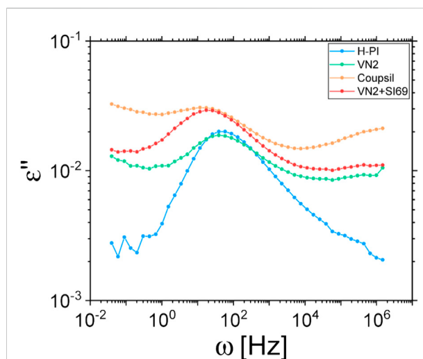
FIGURE 8 Alpha relaxation of the neat polyisoprene matrix and different filler types, with or without silane coupling agent, measured by dielectric spectroscopy at 223 K.
