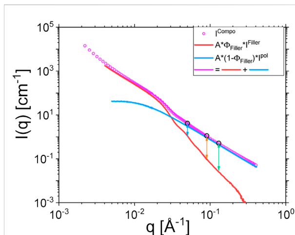
FIGURE 4 Reproduction of composite scattering signal following Eq. 3 . The example is given for sample II. Vertical arrows indicate the scattering vector moduli at which the NSE measurements are performed. The extracted filler scattering using the experimental polymer scattering is congruent with independent SAXS scattering experiments. The same details of the silica particle form factor and intraparticle structure factor are visible in the range 0.03 < q < 0.06 \text{ Å}^{-1} .
