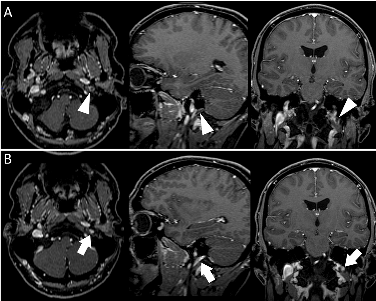
Fig. 2. Thrombosis of the distal left sigmoid sinus after Vaxzevria® vaccination.
