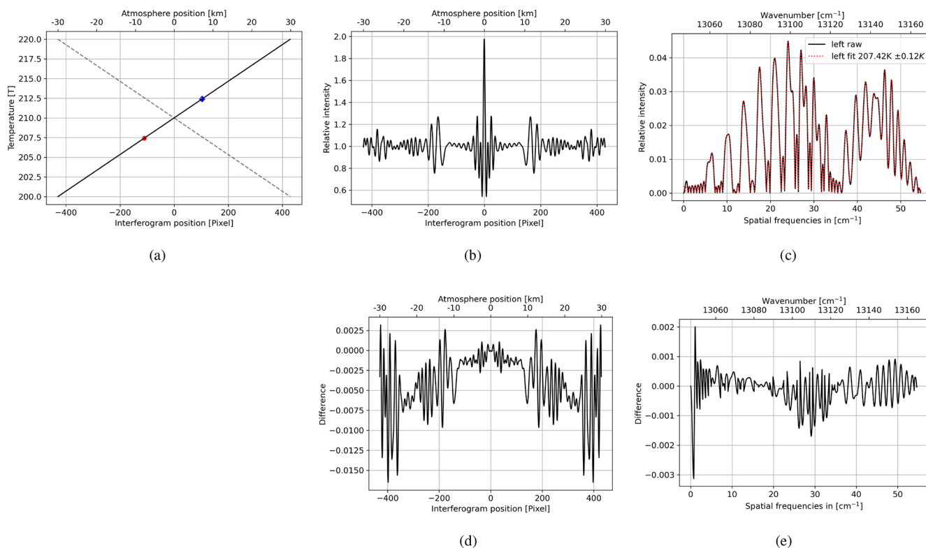
Figure 7. Simulation of interferogram split assuming a linear temperature gradient. Panel (a) shows the temperature gradient from 200 to 220 K across the horizontal field (solid line) with each side symmetrically extended around the center (dashed lines); the red circle and the blue diamond indicate the location of the retrieved temperature for the left and right hand side. Panel (b) shows the left symmetrically extended interferogram. Panel (c) shows the temperature retrieval of (b). Panel (d) shows the difference between the left and right symmetrically extended interferogram. Panel (e) shows the difference between the left and right symmetrically extended raw spectrum.
