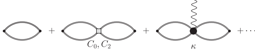
Figure 3. Two-point function of the composite field \phi^2(x) . Double lines denote the full one-particle propagator in the external field, see figure 4. The diagrams, in which the external field is attached to the four-particle vertex, are explicitly included.
