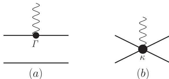
Figure 2. Diagrams contributing to the kernel \tilde{I} which, convoluted with the wave functions \bar{\Psi}, \Psi , yields the resonance form factor, see eq. (2.23). The troublesome triangle diagram (a) in the finite-volume form factor, mentioned in the Introduction, emerges from the disconnected part, where the photon is attached to one of the particles, whereas the second one acts as a spectator. The fully connected diagram (b), where the photon is emanated from the four-particle vertex, is unproblematic.
