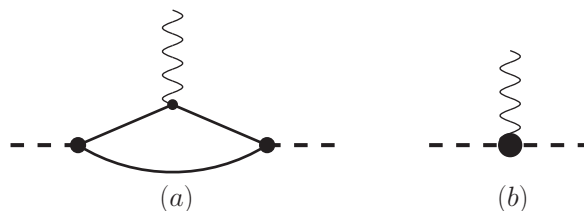
Figure 1. a) The triangle diagram which leads to an irregular behavior of the matrix element in a finite volume, and b) a local vertex that has a regular behavior. The dashed, single and wiggled lines denote the resonance, its constituents and the external current, respectively.
