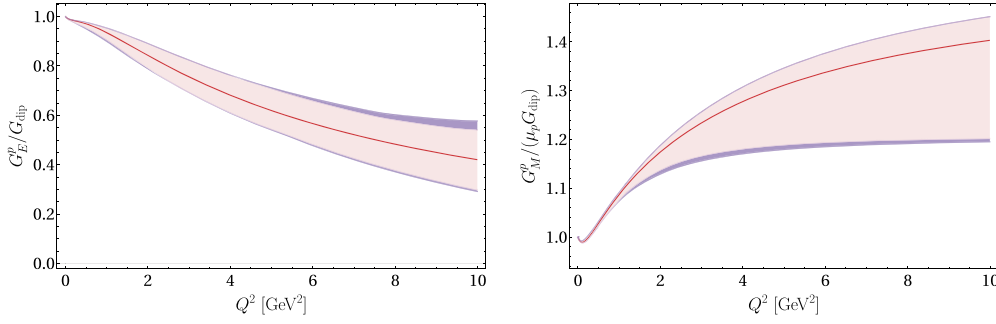
Fig. 2. Electric (left panel) and magnetic (right panel) form factor of the proton from Ref. [5] divided by the canonical dipole form factor are shown by the red lines. The light red band is the statistical uncertainty and the purple band shows the systematic error added in quadrature.
