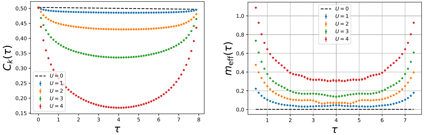
FIG. 5. Dependence of correlators for the lowest energy localized state (left) and its corresponding effective masses (right) as defined in Eq. (5). In both cases, the black dashed line corresponds to the noninteracting result.
