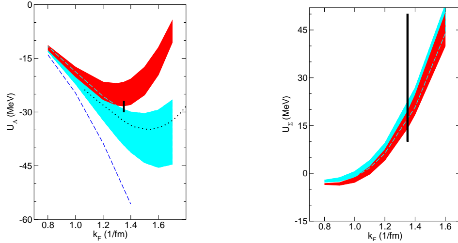
FIGURE 1. Single particle potential for momentum p_Y = 0 depending on the Fermi momentum in symmetric nuclear matter for \Lambda (left) and \Sigma (right). The red (dark) bands are results for NLO13 and the cyan (light) bands result for NLO19 with cutoffs in the range between 500 and 650 MeV. For a comparison also results for Jülich '04 [21] (dashed blue line) and Nijmegen SC97f [20] (dotted black line) are given. The black bars indicate the empirical value [1].
