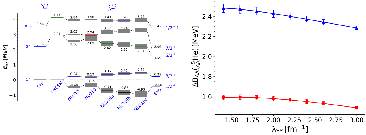
FIGURE 3. Left: Level scheme of {}^7_\Lambda\text{Li} based on SRG evolved YN interactions at NLO. The levels are related to the levels of the {}^6\text{Li} core. For all calculations, \lambda_{YN} has been chosen such that {}^5_\Lambda\text{He} is correctly predicted. The grey bands show the dependence on the chiral cutoffs. Right: \Lambda\Lambda excess energy for {}^5_\Lambda\text{He} depending on the SRG parameter \lambda_{YY} . The upper blue symbols are for the LO, the lower red symbols are for the NLO interaction for a 600 MeV cutoff. Lines are added to guide the eye. Error bars indicate the numerical uncertainty.
