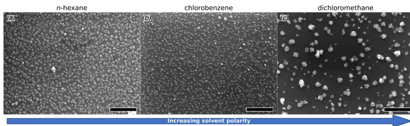
Figure 6. SEM micrographs of Sb 2 Se 3 deposits after 50 cycles obtained by sALD on Si/SiO 2 substrates from 1 mM SbCl 3 and 1 mM of Se precursor 5 from (a) n -hexane, (b) chlorobenzene, and (c) dichloromethane as the solvent, respectively. The scale bar in each micrograph represents 500 nm.
