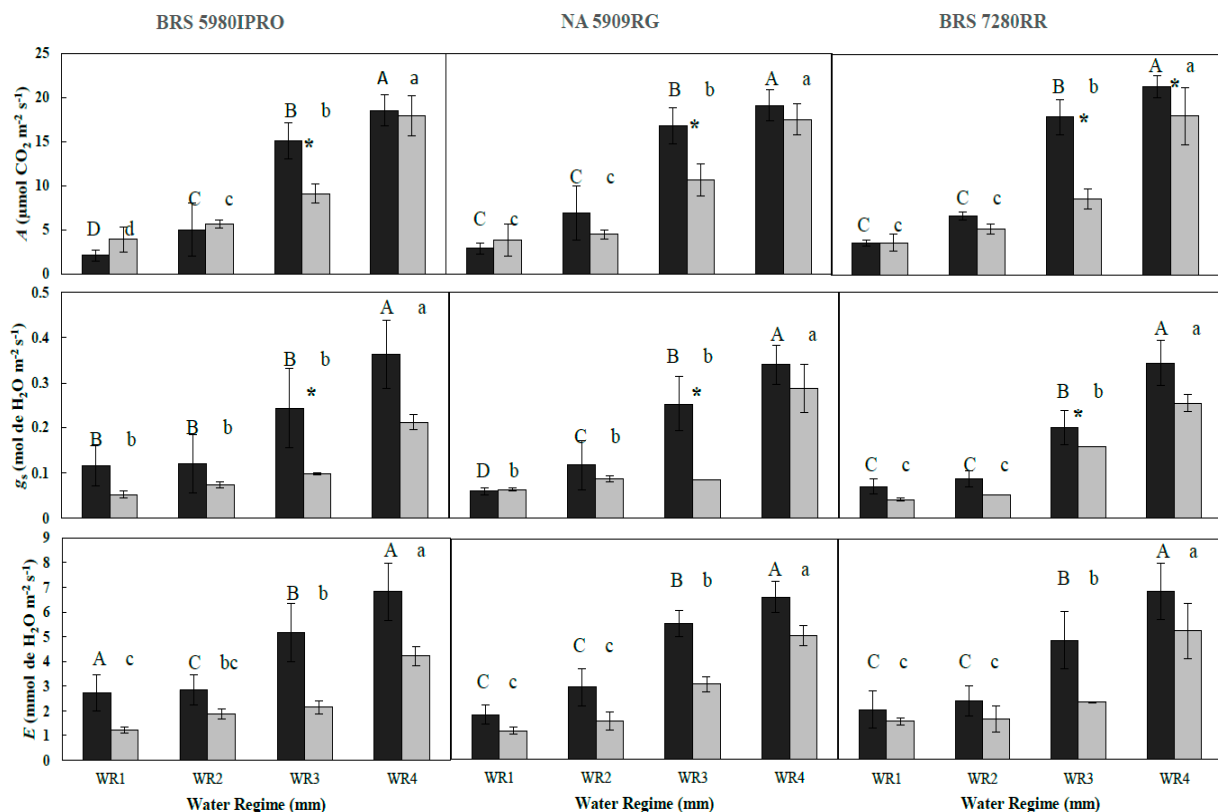
Figure 3. Photosynthesis (A), stomatal conductance ( g_s ) and transpiration (E) in three soybean cultivars submitted to four water regimes (WR) for three cultivars (BRS 5980IPRO, NA 5909RG and BRS 7280RR) with and without polymer supply (WR1 157 mm, WR2 263 mm, WR3 432 mm and WR4 630 mm) in 2016. Uppercase letters indicate differences between the WR for control (without polymer) and lowercase letters indicate differences between the WR for polymer treatment and “*” indicates significant differences between the treatments with and without polymer supply by Tukey's test ( p < 0.05 ).
