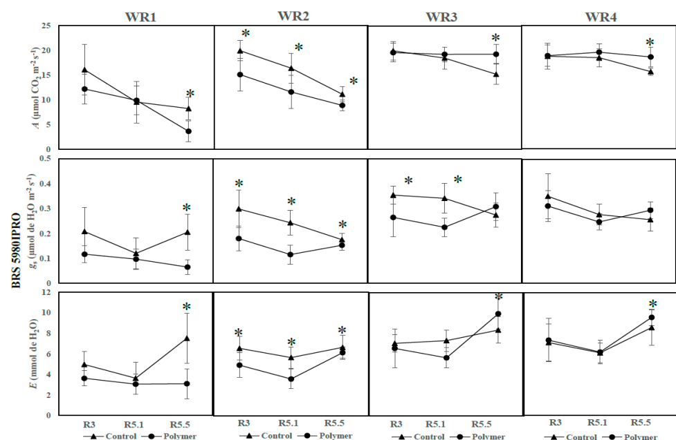
Figure 4. Photosynthesis, ( A ), stomatal conductance ( g_s ) and transpiration ( E ) under four water regimes (WR)
