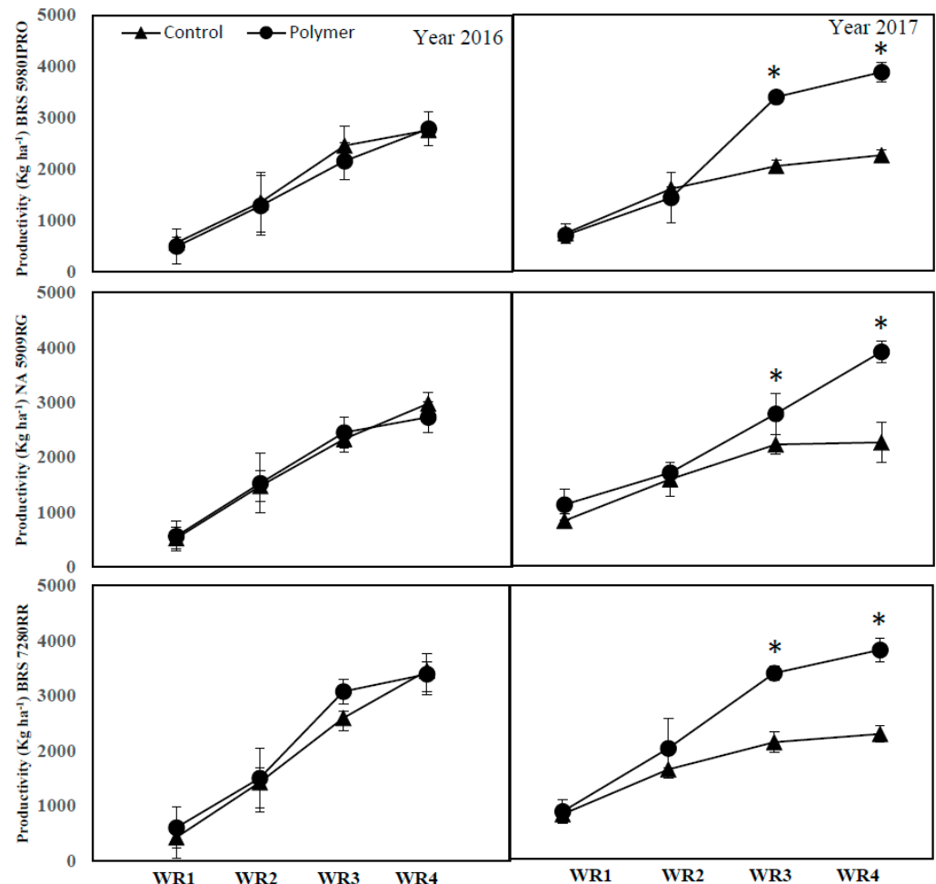
Figure 8. Productivity (Kg ha -1 ) in three soybean cultivars submitted to four water regimes WRs. control (triangles) and polymer-treated (circles) in 2016 and 2017. * indicates significant differences between control and polymer-treated plants by Tukey's test ( p < 0.05 ) (WR1 157 mm, WR2 263 mm, WR3 432 mm and WR4 630 mm in 2016; WR1 167 mm, WR2 237 mm, WR3 341 mm and WR4 534 mm in 2017).
