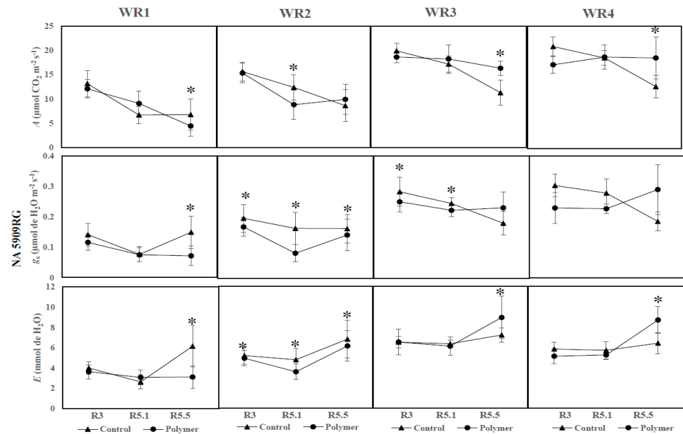
Figure 5. Photosynthesis, (A), stomatal conductance ( g_s ) and transpiration (E) under four water regimes (WR) in three phenological stages of soybean with and without polymer supply (WR1 167 mm, WR2 237 mm, WR3 341 mm, WR4 534 mm) for the NA 5909RG cultivar, in 2017. * indicates significant differences between the control and polymer treatments within each WR and phenological phase by Tukey's test ( p < 0.05 ).
