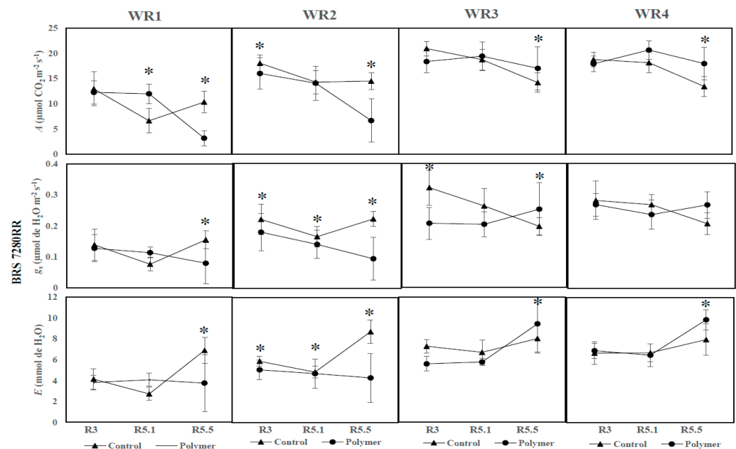
Figure 6. Photosynthesis, (A), stomatal conductance ( g_s ) and transpiration (E) under four water regimes (WR) in three phenological stages of soybean with and without polymer supply (WR1 167 mm, WR2 237 mm, WR3 341 mm, WR4 534 mm) for the BRS 7280RR cultivar, in 2017. * indicates significant differences between the control and polymer treatments within each WR and phenological phase by Tukey's test ( p < 0.05 ).
