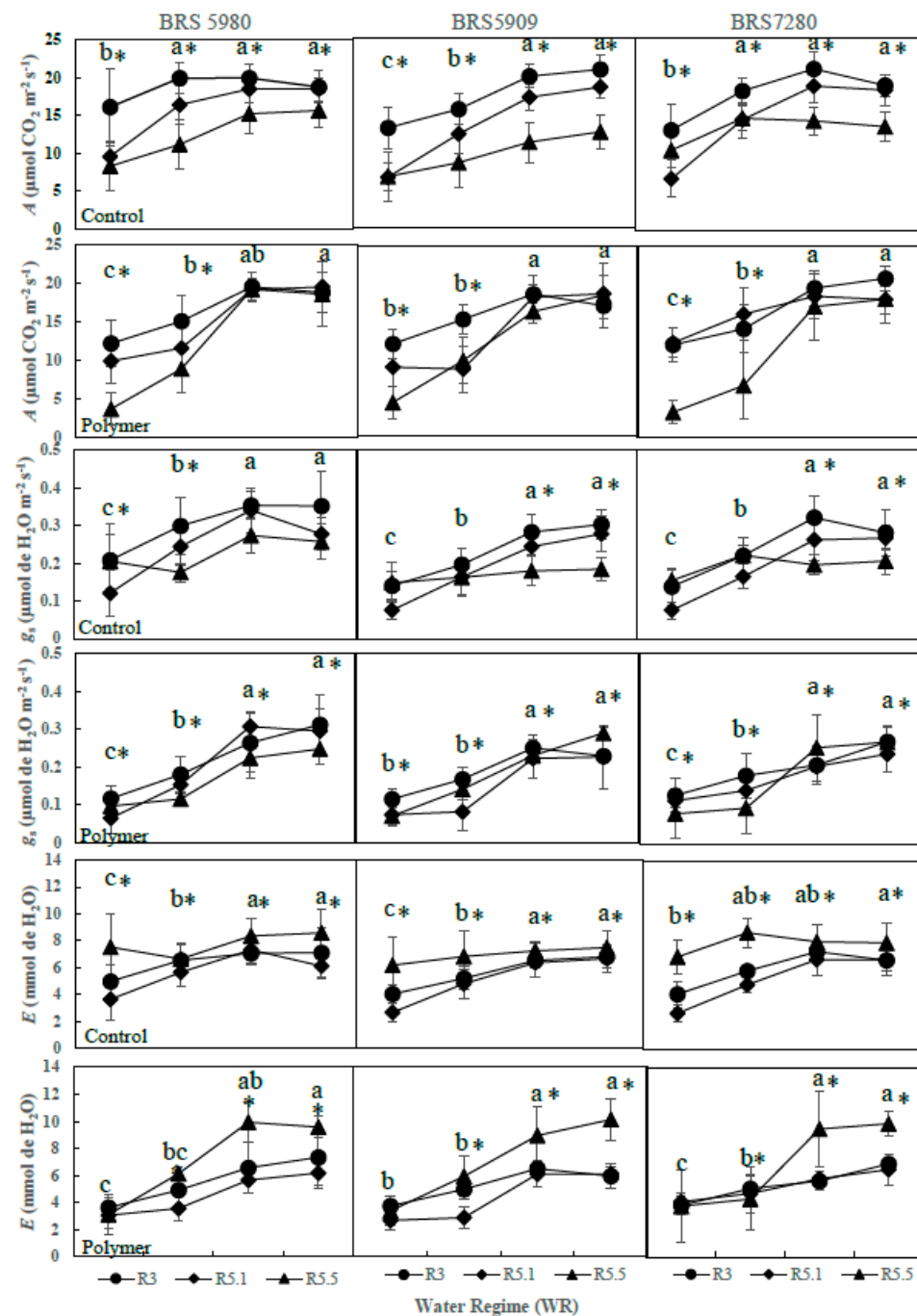
Figure 7. Photosynthesis, ( A ), stomatal conductance ( g_s ) and transpiration ( E ) in three soybean cultivars submitted to four water regimes (WR) in three phenological stages of soybean development with and without polymer supply (WR1 167 mm, WR2 237 mm, WR3 341 mm, WR4 534 mm), in 2017. Lowercase letters indicate differences between the WR for each cultivar and * indicates significant differences between the phenological phases within each WR by Tukey's test ( p < 0.05 ).
