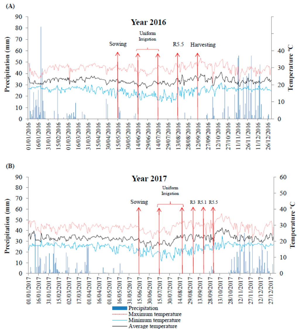
Figure 1. (A) Precipitation, maximum, minimum and average temperatures, rainfall and the sowing, evaluation and harvesting dates of soybean plants in 2016 and (B) 2017.
