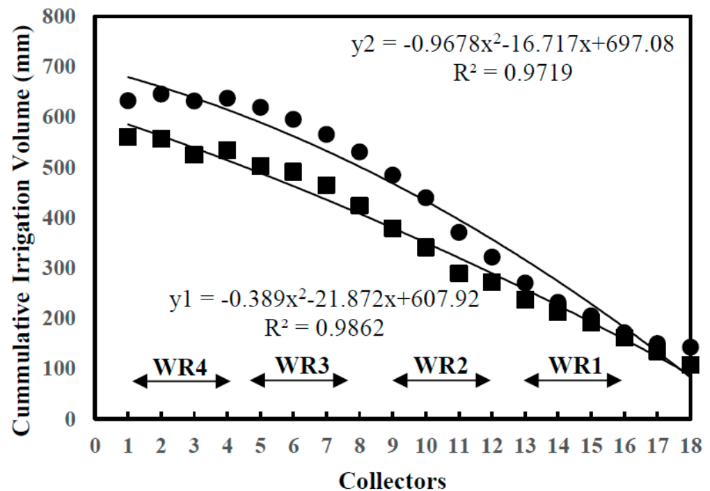
Figure 2. Cumulative irrigation volume applied in soybean crop during the dry season in 2016 (y1) and 2017 (y2).
