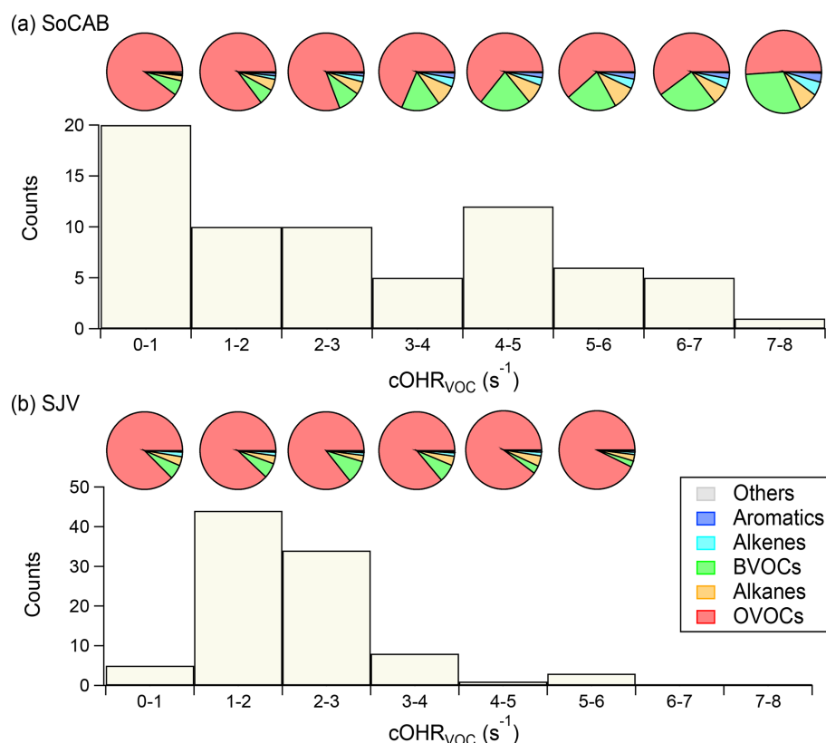
Figure 6. Frequency distribution of cOHR_{VOC} in the (a) SoCAB and (b) SJV. Also shown above each 1 s^{-1} binned cOHR_{VOC} range is a pie chart presenting the average contribution to the cOHR_{VOC} by VOC categories (shown in the legend).
