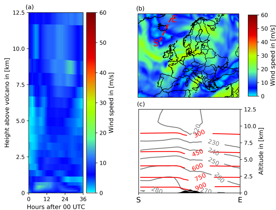
Figure 5. Meteorological conditions on 29 April 2010. (a) Wind speed above the volcano for the whole simulation period. (b) Wind speed at 500 hPa on 29 April 2010, 12:00 UTC, which corresponds to approx. 5 km above the volcano. (c) Vertical cross section of isobars in [hPa] (red) and isotherms in [K] (gray) along the red line in (b) on 29 April 2010, 12:00 UTC.
