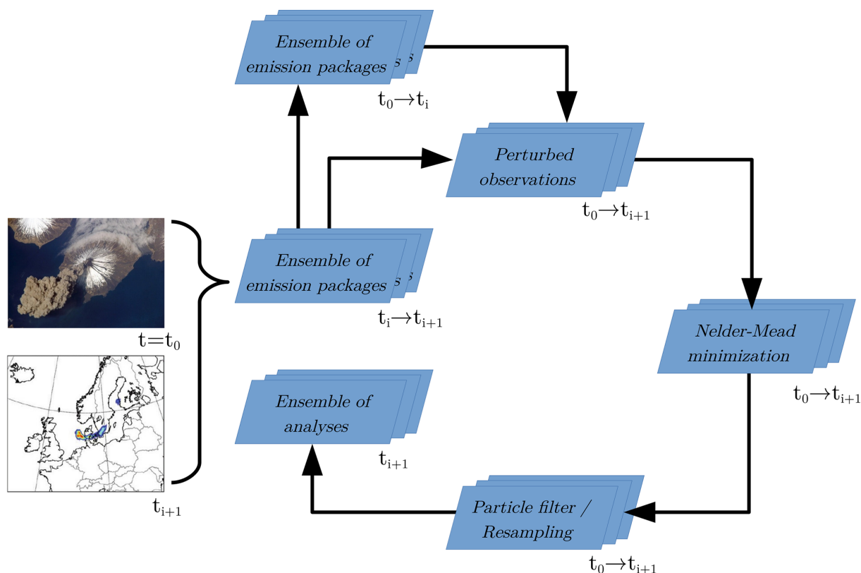
Figure 1. Schematic of the ESIAS-chem analysis workflow. The analysis is initiated at time t = t_0 and restarted when new observations become available (left side, see Sect. 2.1.1). Here, t_{i+1} corresponds to the observation time. Previously calculated simulations with emission packages within the time interval t_0 - t_i may be restored (upper blue box). Simulated volcanic ash is compared with perturbed observations for the whole simulation (i.e., from t_0 to t_{i+1} ; upper central blue box). The resulting volcanic ash concentrations are passed to the DENM minimization algorithm that produces an ensemble of emission profile analyses (right blue box, see Sect. 2.1.2) by finding an optimal combination of the pairwise distinct emission packages. This ensemble of emission profile analyses is evaluated by the particle filter and resampling method to assign a weight to each emission profile according to the fit of the resulting volcanic ash to the observations. Emission profiles are replaced if their corresponding volcanic ash content does not fit the observations well (lower blue box, see Sect. 2.1.3). Credits for volcano image: NASA ( https://www.nasa.gov/multimedia/imagegallery/image_feature_756.html , last access: 13 January, 2021; Cleveland volcano, Aleutian Islands).
