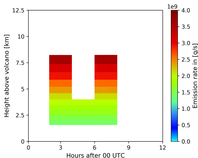
Figure 2. Hovmöller-like plot of the volcanic ash emission profile used in the nature run to generate the synthetic observations simulating SEVIRI-like column mass loading data for the ESIAS-chem system tests. Shown is the emission rate (colored) for a given time ( x axis) and height above the volcano ( y axis).
