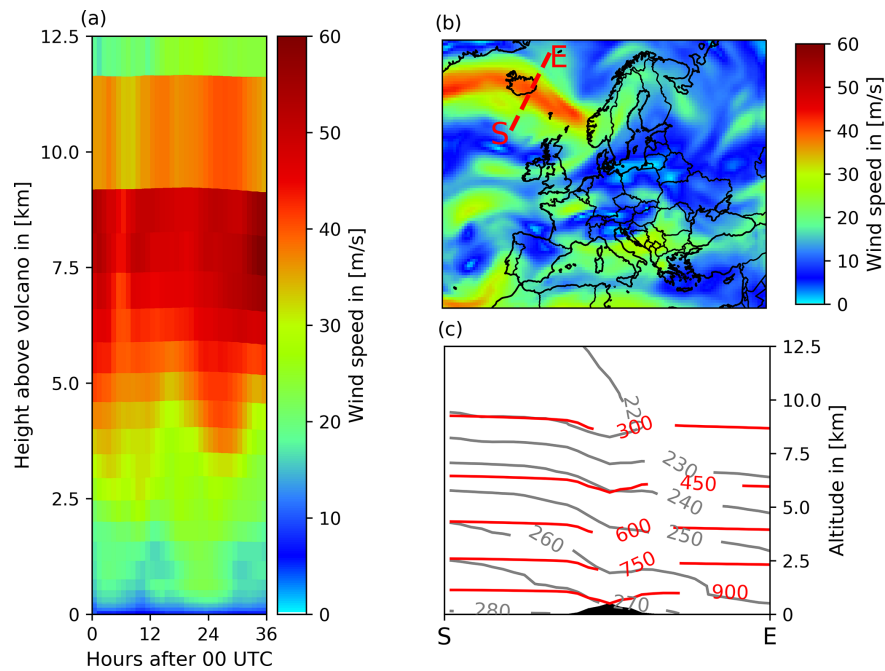
Figure 4. Meteorological conditions on 15 April 2010. (a) Wind speed above the volcano for the whole simulation period. (b) Wind speed at 500 hPa on 15 April 2010, 12:00 UTC, which corresponds to approx. 5 km above the volcano. (c) Vertical cross section of isobars in [hPa] (red) and isotherms in [K] (gray) along the red line in (b) on 15 April 2010, 12:00 UTC.
