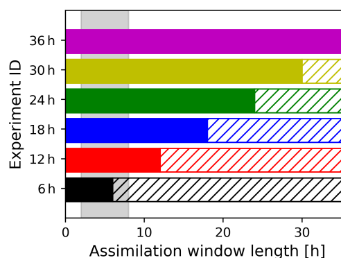
Figure 3. Illustration of the varying assimilation window lengths for the identical-twin experiment (filled bars). After each assimilation window, a free forecast until 36 h after the start of the simulation is appended (hatched bars). Color codes and experiment IDs correspond to the annotations in the subsequent figures. The gray background area indicates the duration of the volcanic eruption from hours 2 to 8.
