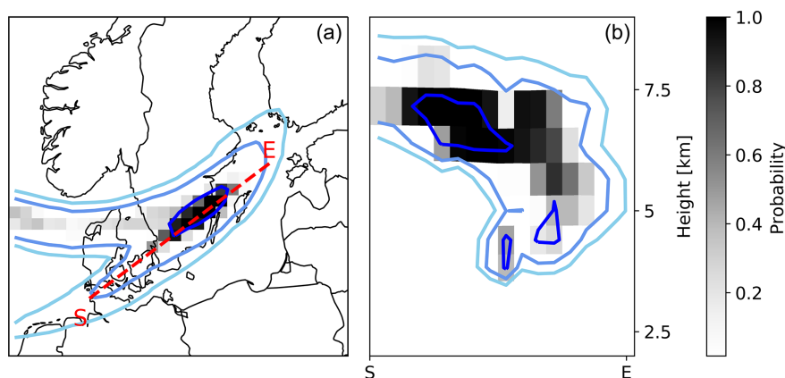
Figure 14. Probability maps on 16 April 2010, 00:00 UTC, from the 24 h assimilation window test case. (a) Probability of the analysis ensemble for volcanic ash column mass loading exceeding 2 \text{ g m}^{-2} (shaded areas). Contour lines of nature run volcanic ash column mass loading for 0.5, 1, and 2 \text{ mg m}^{-2} are given by blue lines. (b) Vertical contours of the probability of the analysis ensemble of volcanic ash concentration exceeding 500 \text{ µg m}^{-3} along the red dashed line in (a) . Contour lines of nature run volcanic ash concentrations for 250, 350, and 500 \text{ µg m}^{-3} are shown by blue lines.
