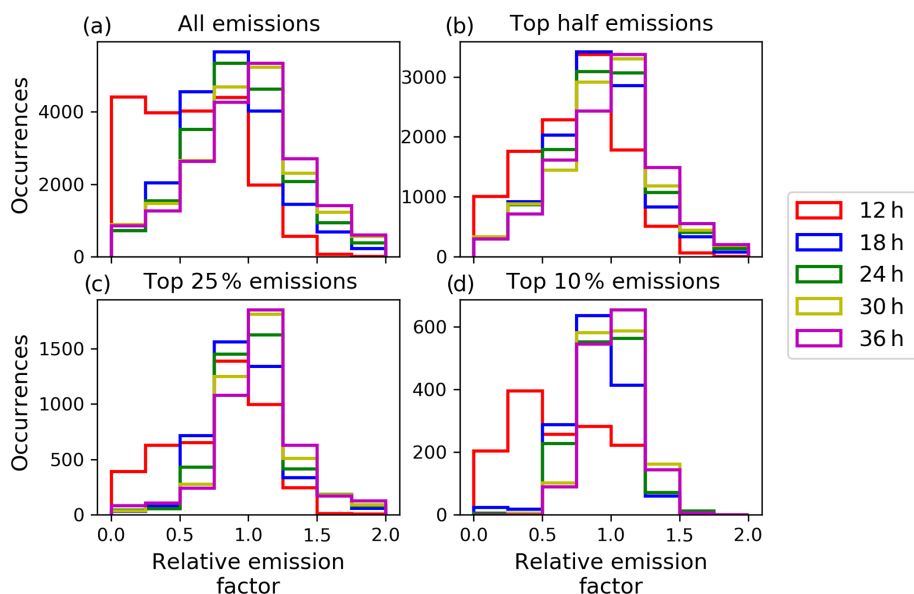
Figure 11. Histogram of the relative emission factors for different assimilation window lengths for the test case on 15 April, 2010 with color codes as in Fig. 3. The relative emission factor is calculated according to Eq. (14). The histograms are shown for (a) all emission rates, (b) the top half, (c) the top 25 %, and (d) the top 10 % emission rate.
