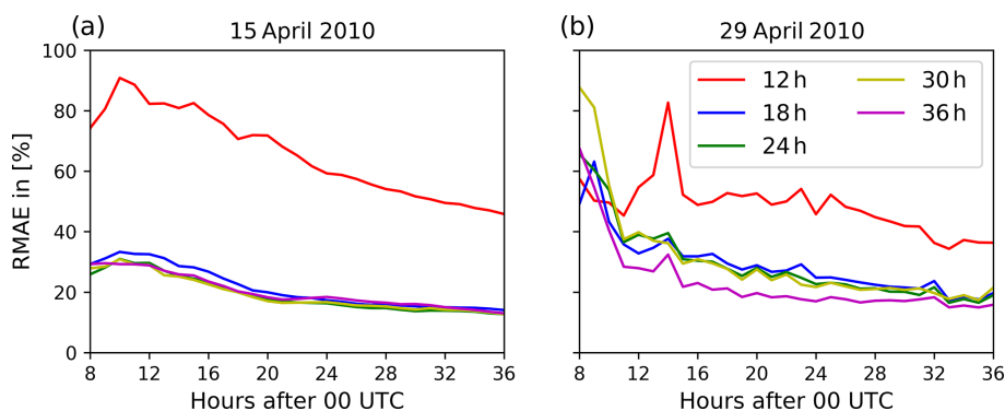
Figure 8. Relative mean absolute error of the volcanic ash concentrations defined by Eq. (9) for the eruption on (a) 15 April 2010 and on (b) 29 April 2010. The different lines indicate different assimilation window lengths from 12 h (red) to 36 h (magenta) as defined by Fig. 3.
