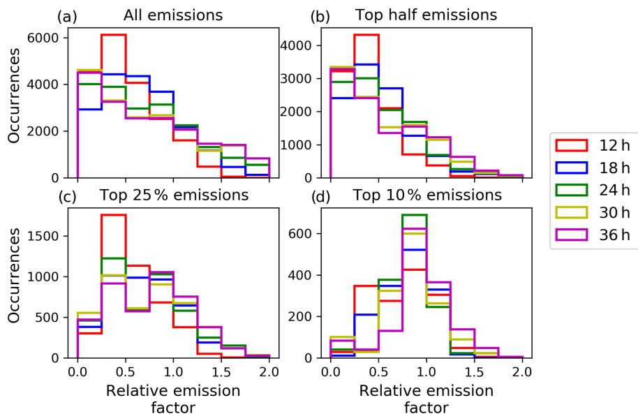
Figure 12. Histogram of the relative emission factors for different assimilation window lengths for the test case on 29 April 2010, with color codes as in Fig. 3. The relative emission factor is calculated according to Eq. (14). The histograms are shown for (a) all emission rates, (b) the top half, (c) the top 25 %, and (d) the top 10 % emission rate.
