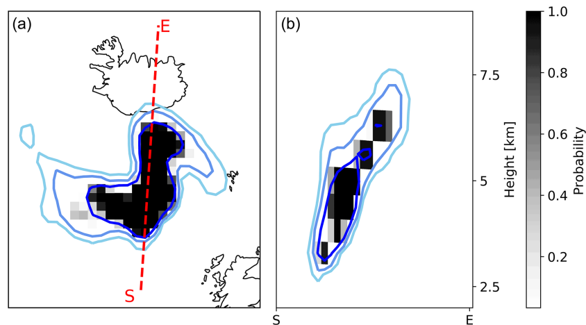
Figure 15. Probability map on 30 April 2010, 12:00 UTC, from the 24 h assimilation window test case. (a) Probability of the analysis ensemble for volcanic ash column mass loading exceeding 2 \text{ g m}^{-2} (shaded areas). Contour lines of nature run volcanic ash column mass loading for 0.5, 1, and 2 \text{ g m}^{-2} are given by blue lines. (b) Vertical contours of the probability of the analysis ensemble of volcanic ash concentrations exceeding 2 \text{ mg m}^{-3} along the red dashed line in (a) . Contour lines of nature run volcanic ash concentrations for 0.5, 1, and 2 \text{ mg m}^{-3} are shown by blue lines.
