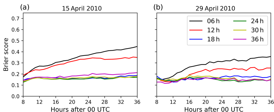
Figure 13. Brier score as calculated by Eq. (10) for each hour and all assimilation window lengths for (a) 15 April and (b) 29 April 2010.
